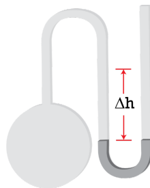
Closed-end Manometer
