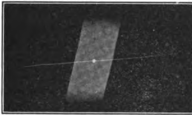
FIG. 8.—PYROMETER FILAMENT PROJECTED AGAINST HOLE AND SURFACE OF A PERFORATED TUBULAR TUNGSTEN FILAMENT AS BACKGROUND, AS USED IN EMISSIVE POWER DETERMINATIONS OF TUNGSTEN.
