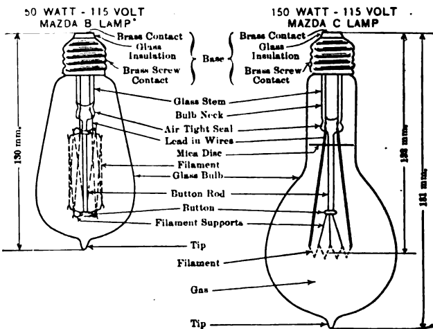
FIG. 1.—ARRANGEMENT OF PARTS IN MAZDA B AND MAZDA C LAMPS.
