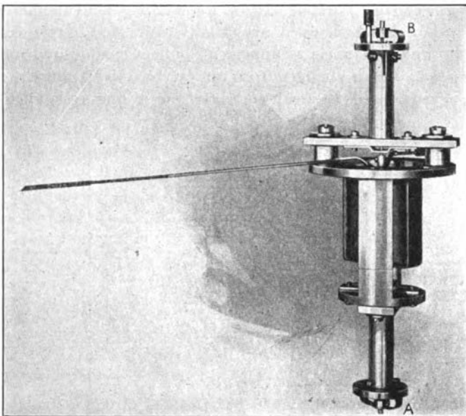
FIG. 4.—MOVING ELEMENT OF THE ENGELHARD INDICATOR. A DOUBLE-SUSPENSION INSTRUMENT IN WHICH THE SUSPENSIONS ARE KEPT UNDER TENSION BY THE SPRINGS A AND B . THE TENSION IS SUFFICIENT TO MAINTAIN AXIAL ALIGNMENT OF THE COIL WITHOUT PRECISE LEVELING. THE INSTRUMENT IS VERY ROBUST AND HAS A HIGH RESISTANCE, ABOUT 50 OHMS PER MILLIVOLT.
