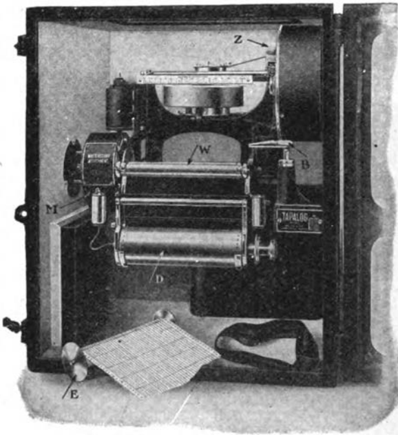
FIG. 15.—WILSON-MAEULEN RECORDER.
