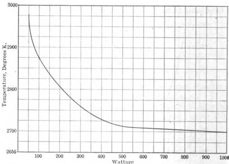
FIG. 4.—VARIATION OF TEMPERATURE WITH LAMP SIZE.
