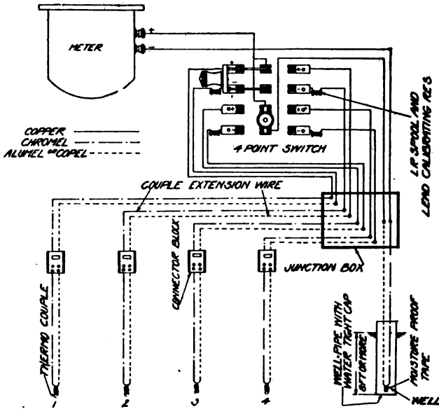
FIG. 1.—WIRING DIAGRAM FOR ONE COUPLE EXTENSION CIRCUIT.
