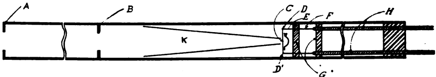
FIG. 8.—RECEIVING SYSTEM OF THWING RADIATION PYROMETER.
