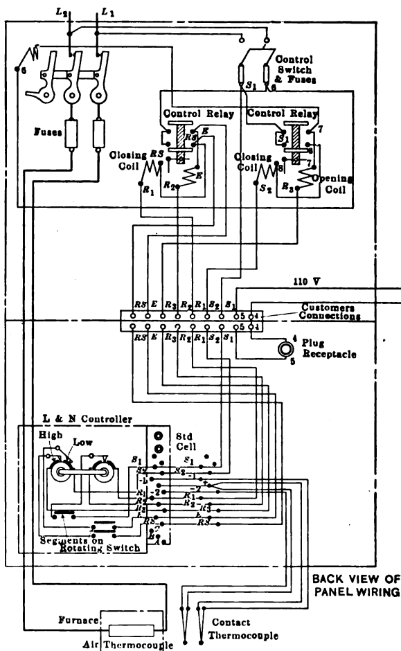
FIG. 9.—WIRING DIAGRAM OF AUTOMATIC CONTROL PANEL FOR ELECTRIC FURNACES.
