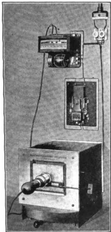
FIG. 7.—AUTOMATIC TEMPERATURE-CONTROL PYROMETER.
