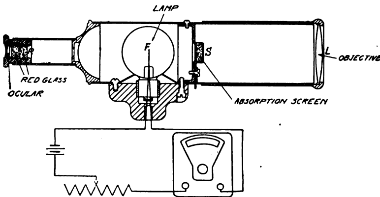
FIG. 6.—LEEDS & NORTHRUP OPTICAL PYROMETER.
