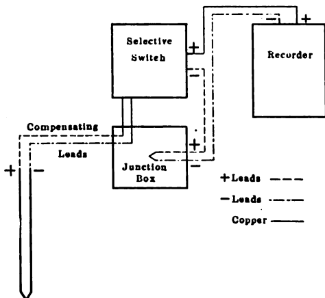
FIG. 33.—ILLUSTRATING USE OF JUNCTION BOX WITHOUT COLD-JUNCTION CONTROL.
