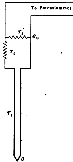
FIG. 22.—COLD-JUNCTION COMPENSATION BY SHUNT AND SERIES RESISTANCE.
