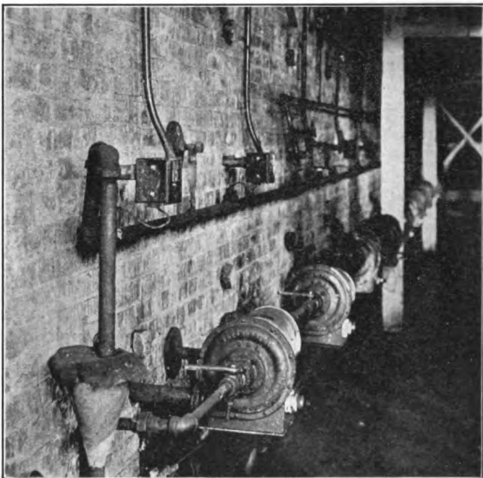
FIG. 4.—STEAM-TREATERS, SHOWING PREMIX BURNERS, PYROMETER TUBES, CONNECTION BOXES, COMPENSATING COUPLES, AND COLD-JUNCTION WELLS. TYPICAL OF FIRST FORTY STEAM-TREATERS ERECTED.
