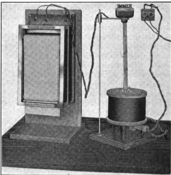
FIG. 5.—RECORDING PYROMETERS FOR TRANSFORMATION POINTS.
