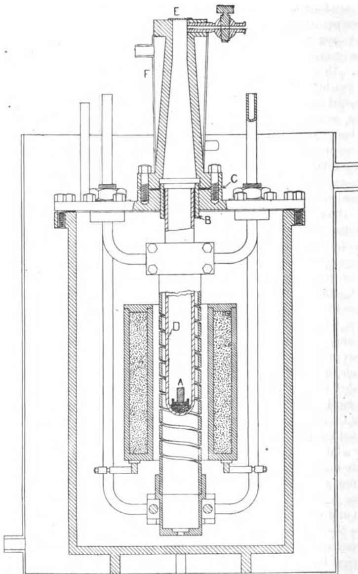
FIG. 1.—CROSS-SECTION OF ARSEM GRAPHITE RESISTANCE VACUUM FURNACE. A IS COMPRESSED CYLINDRICAL SAMPLE. D IS SILLIMANITE PROTECTION TUBE.
