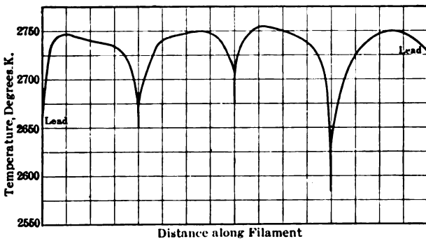
FIG. 6.—6.6 AMP. STREET SERIES LAMP, FOUR SECTIONS.
