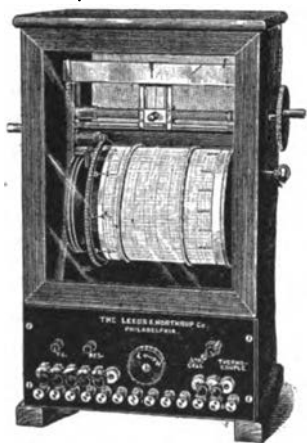
FIG. 22.—LEEDS & NORTHROP TRANSFORMATION POINT INDICATOR.
