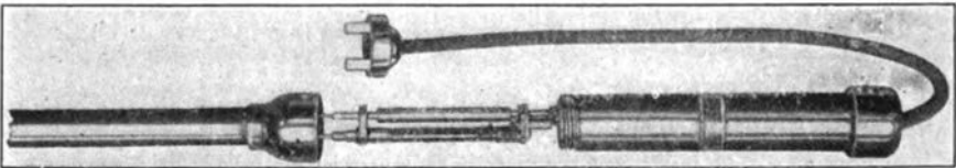
FIG. 3.—INTERIOR OF THERMOCOUPLE HEAD MADE BY BEIGHLEE ELECTRIC Co., SHOWING THE COLD-JUNCTION COMPENSATOR DESCRIBED UNDER FIG. 23.
