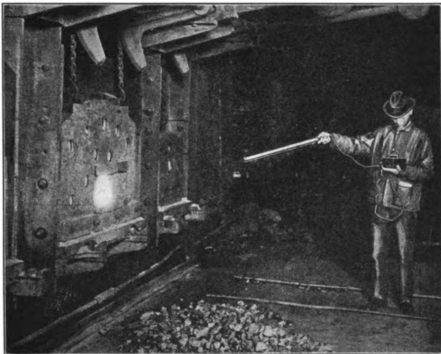
FIG. 9.—OBSERVING TEMPERATURE OF A FURNACE WITH THWING RADIATION PYROMETER.
