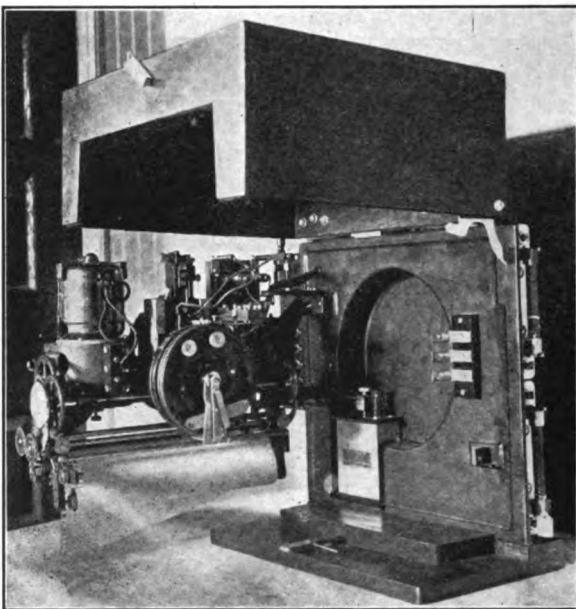
FIG. 20.—LEEDS & NORTHRUP RECORDER.
