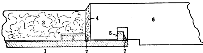
FIG. 3.—ARRANGEMENT OF TUBE FOR TAKING STEEL TEMPERATURES. 1. WROUGHT-IRON TUBE 2\frac{3}{8} - 2\frac{1}{2} IN. OUTSIDE DIAMETER; 2. CERAMIC SLEEVE; 3. WROUGHT-IRON RING TO SUPPORT SLEEVE; 4. CLAY OR CEMENT; 5. WROUGHT-IRON LUGS 1 IN. LONG; 6. GRAPHITE TUBE; 7. WELD TO W.I. PIPE.
