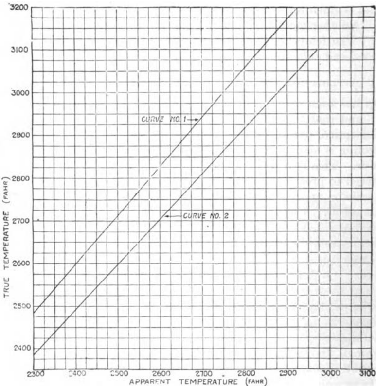
FIG. 5.—EMISSIVITY CORRECTIONS FOR STEEL AND SLAG. Curve 1—Steel. Curve 2—Slag.
