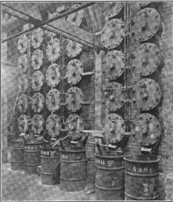
FIG. 2.—DISCHARGE END OF AIR-TREATERS, SHOWING ENDS OF PYROMETER TUBES AND CONDUIT FOR THE LEAD WIRES.
