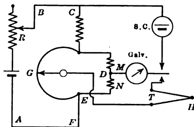
FIG. 20.—AUTOMATIC COLD-JUNCTION COMPENSATOR.
