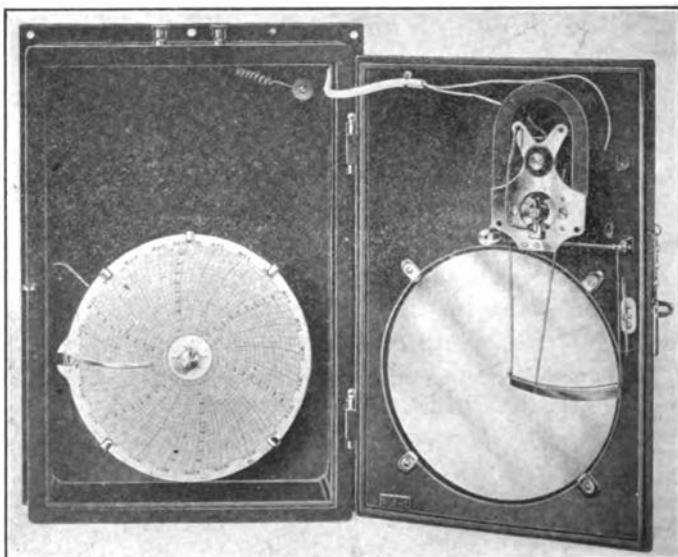
FIG. 6.—BROWN RECORDER.
