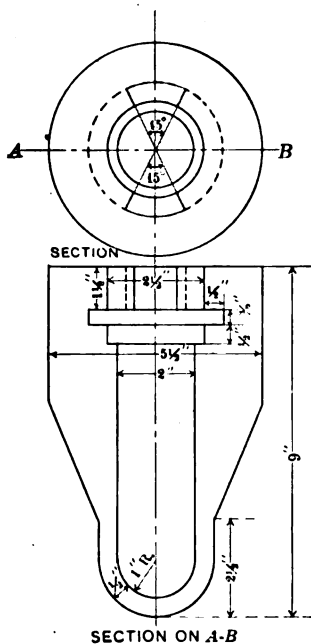
FIG. 2.—REFRACTORY TUBE FOR TAKING STEEL TEMPERATURES.
