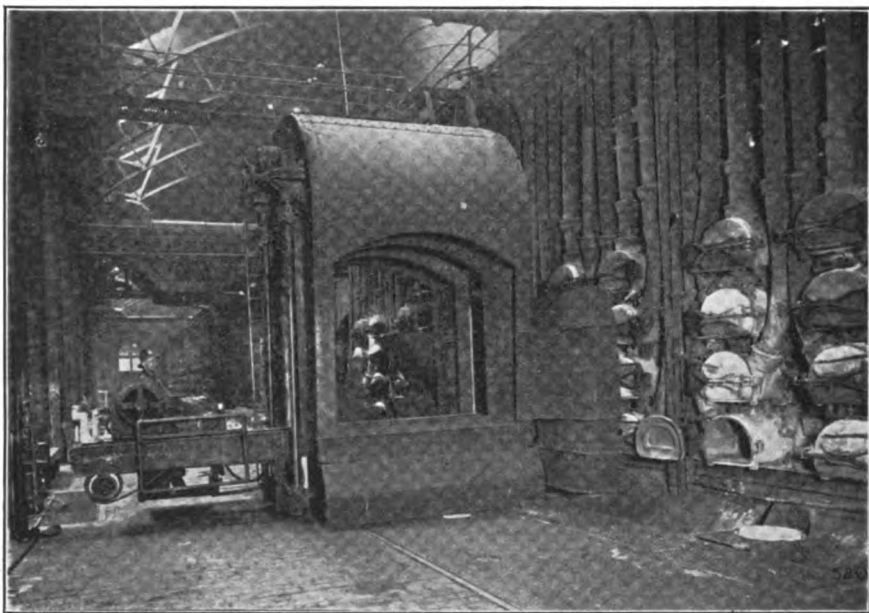
FIG. 1.—RETORTS, SHOWING A RETORT BEING DRAWN BY THE DISCHARGING MACHINE.
