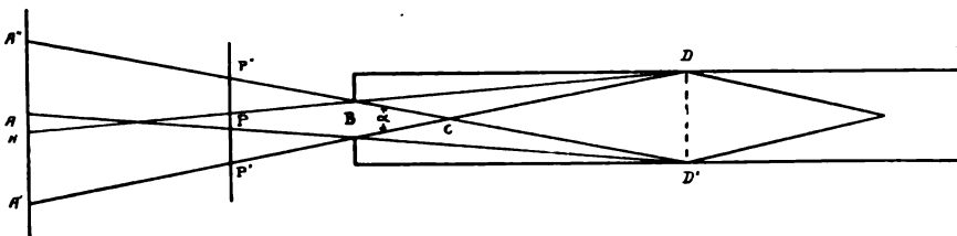
FIG. 10.—CONE TYPE OF FIXED-FOCUS RADIATION PYROMETER.
