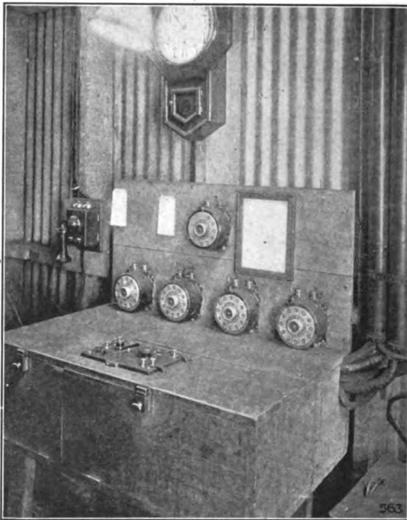
FIG. 3.—PYROMETER FOR AIR-TREATERS, SHOWING COMMON COLD-JUNCTION BOX, WILSON-MAEULEN SWITCHES, AND LEEDS & NORTHRUP POTENTIOMETER.
