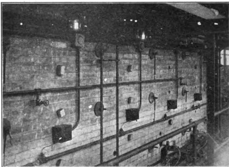
FIG. 7.—STEAM-TREATERS, SHOWING THERMOCOUPLE CONNECTION BOXES, COLD-JUNCTION WELLS, AND SIGNAL LIGHTS. ARRANGED FOR CENTRAL-STATION CONTROL. TYPICAL OF LAST SIXTY STEAM-TREATERS ERECTED.
