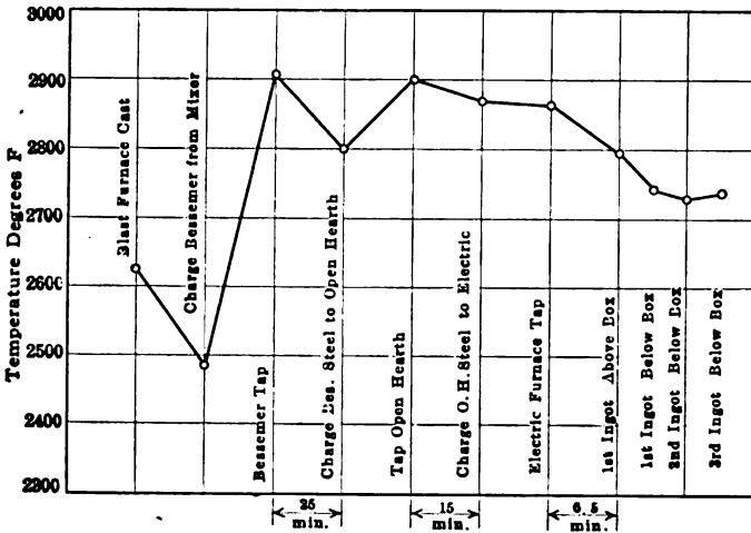
FIG. 3.—TEMPERATURES IN TRIPLEX PROCESS.
