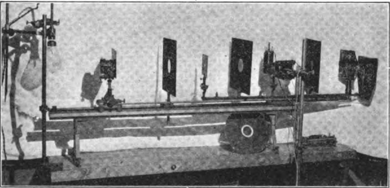
FIG. 3.—LABORATORY FORM OF OPTICAL PYROMETER. LENGTH FROM EYEPIECE TO OBJECTIVE LENS, 225 CM.
