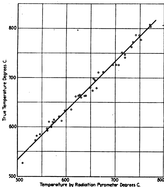
FIG. 4.—RADIATION TEMPERATURE AND TRUE TEMPERATURE RELATION FOR IRON OXIDE ACCORDING TO BURGESS AND FOOTE.
