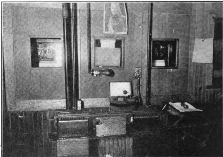
FIG. 6.—RECORDING PYROMETER AS SEEN FROM FURNACE ROOM, SHOWING LEEDS & NORTHRUP RECORDING POTENTIOMETER IN THE CASE, AND PUSH-BUTTON SWITCHES AND INDICATING POTENTIOMETER BELOW.
