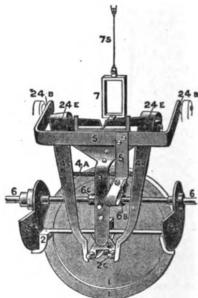
FIG. 5.—MECHANISM BALANCED.
