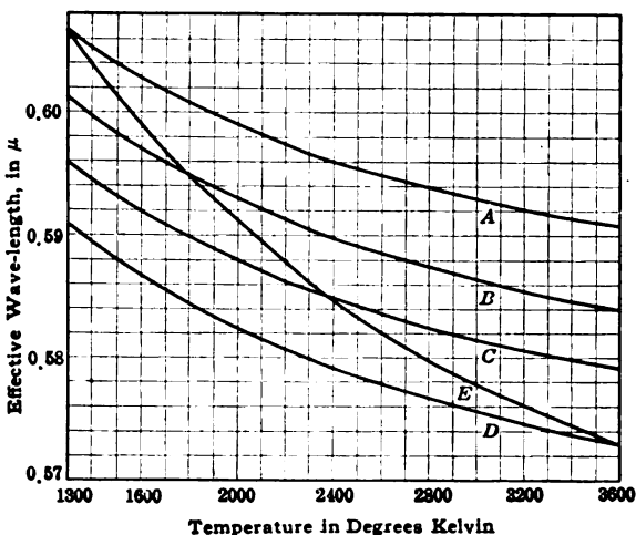
FIG. 5.—EFFECTIVE WAVE-LENGTHS FOR CORNING RED GLASS. SPECTRAL TRANSMISSION SHOWN BY CURVE B , FIG. 4. CURVE A , EFFECTIVE WAVE-LENGTHS FROM 1300° TO OTHER TEMPERATURE. CURVE B , EFFECTIVE WAVE-LENGTHS FROM 1800° TO OTHER TEMPERATURE. CURVE C , EFFECTIVE WAVE-LENGTHS FROM 2400° TO OTHER TEMPERATURE. CURVE D , EFFECTIVE WAVE-LENGTHS FROM 3600° TO OTHER TEMPERATURE. CURVE E , LIMITING EFFECTIVE WAVE-LENGTH.
