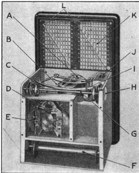
FIG. 8.—HOSKINS RECORDER.
