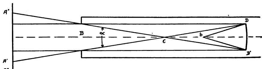
FIG. 12.—MIRROR TYPE OF FIXED-FOCUS RADIATION PYROMETER.
