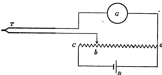
FIG. 8.—SIMPLE WIRING DIAGRAM FOR POTENTIOMETRIC INDICATOR.
