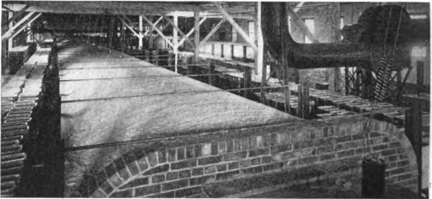
FIG. 3.—AMERICAN DRESSLER TUNNEL KILN.
