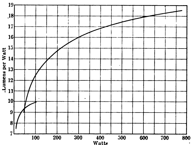
FIG. 5.—VARIATION OF EFFICIENCY WITH LAMP SIZE, 1000-HR. LIFE.
