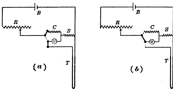
FIG. 11.—WIRING DIAGRAM OF PYROVOLTER.
