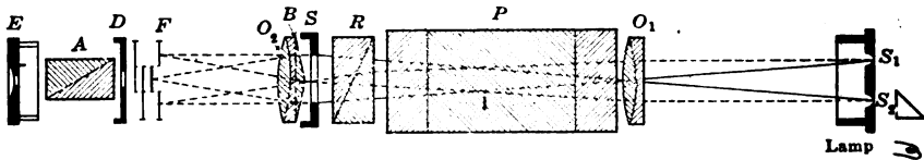
FIG. 3.—WANNER PYROMETER.
