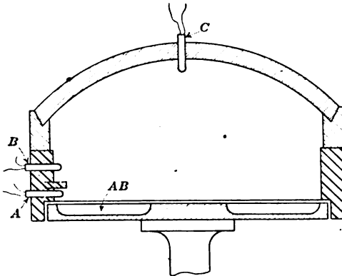
FIG. 2.—OWENS REVOLVING POT.
