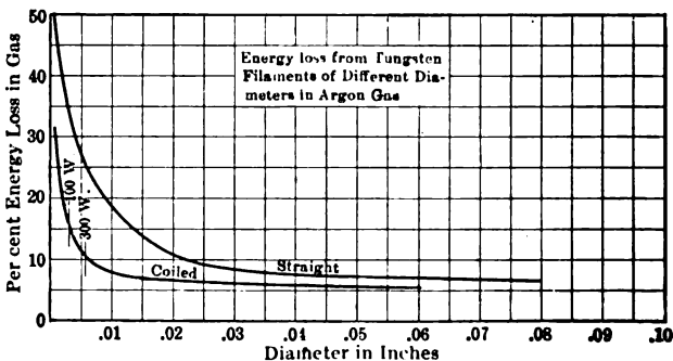
FIG. 4.—PER CENT. GAS LOSS FOR STRAIGHT AND COILED FILAMENTS IN GAS.
