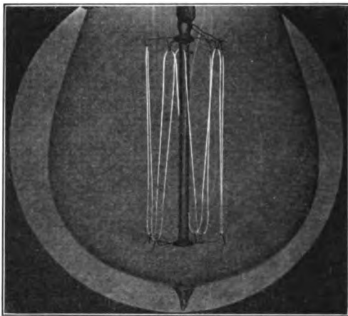
FIG. 3.—100-WATT MAZDA B CONSTRUCTION LAMP WHICH HAS BEEN GAS-FILLED.
