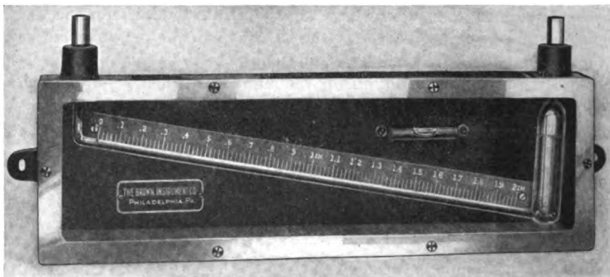
FIG. 2.—DRAFT GAGE 0 TO 2" OF WATER.
