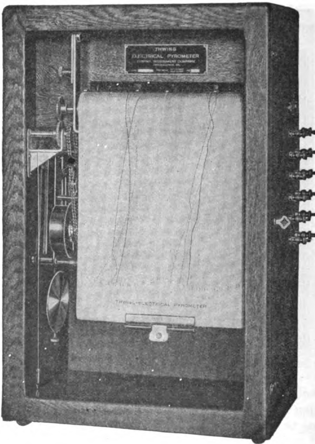
FIG. 13.—THWING RECORDER.
