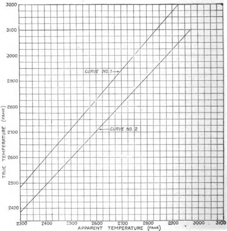
FIG. 1.—EMISSIVITY CORRECTIONS FOR STEEL AND SLAG. Curve 1.—Steel. Curve 2.—Slag.
