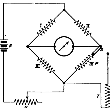
FIG. 1.—COMMON ARRANGEMENT OF RESISTANCES OF DIRECT TEMPERATURE-READING INSTRUMENTS.
