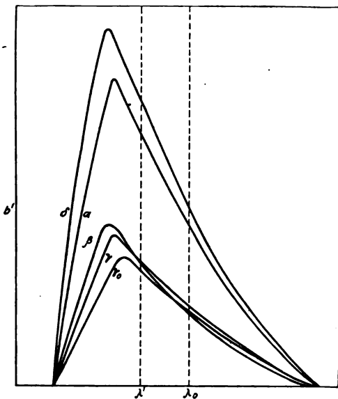
FIG. 9.—VARIOUS SPECTRAL BRIGHTNESS, b' , DISTRIBUTIONS CONNECTED WITH TUNGSTEN FILAMENTS, WHICH ARE HELPFUL IN DETERMINING THE WAVE-LENGTH TO WHICH TO ASCRIBE BRIGHTNESS TEMPERATURE MEASUREMENTS.
