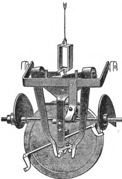
FIG. 4.—MECHANISM UNBALANCED.
