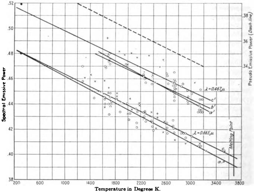
FIG. 10.—EMISSIVE POWER RESULTS AND A COMPUTED PSEUDO-EMISSIVE POWER CURVE FOR TUNGSTEN AS A FUNCTION OF THE TEMPERATURE AT 0.665\mu AND 0.467\mu . X VALUES OBTAINED ON UNPOLISHED FILAMENT IN MUCH STRIATED BULBS; + VALUES OBTAINED ON POLISHED FILAMENTS IN MUCH STRIATED BULBS; ° VALUES OBTAINED ON POLISHED FILAMENT IN FAIRLY CLEAR BULBS; ● VALUES OBTAINED AT ROOM TEMPERATURE BY REFLECTION METHOD; a, a', WEIGHTED CURVES FOR DATA OBTAINED; b', CURVE a' CORRECTED FOR LACK OF MONOCHROMATISM FOR THE UVIOLETT GLASS; c, c', FINAL CURVES CONTAINING CORRECTIONS FOR DIFFERENCES IN TEMPERATURE BETWEEN INTERIOR AND EXTERIOR SURFACES OF THE FILAMENTS.
