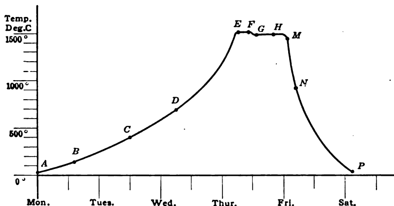
FIG. 1.—TEMPERATURE CYCLE.
