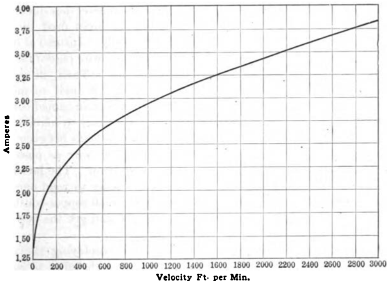
Fig. 2.—RELATION BETWEEN SPEED OF WIRE THROUGH AIR AT ROOM TEMPERATURE AND CURRENT NECESSARY TO MAINTAIN THERMOCOUPLE FUNCTION AT 200° C.
