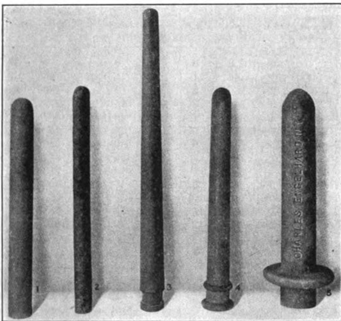
FIG. 35.—PROTECTING TUBES FOR COUPLES.
