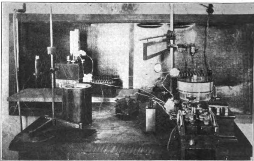
FIG. 1.—APPARATUS USED TO OBTAIN TEMPERATURE OF BURNING CIGAR.
