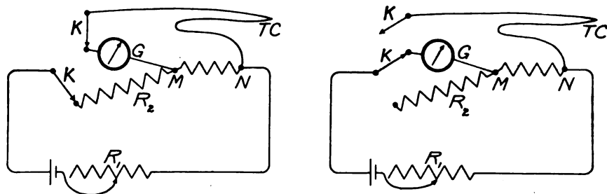
FIG. 2.—PYROVOLTER. FIRST POSITION, POTENTIAL DROP MN IS MADE EQUAL TO ELECTROMOTIVE FORCE OF THERMOELEMENT; SECOND POSITION, CURRENT IS MEASURED BY SAME GALVANOMETER.
