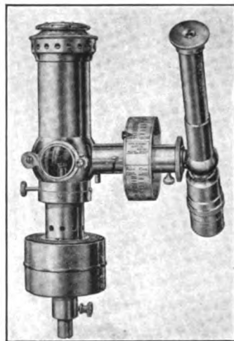
FIG. 2.—SHORE PYROSCOPE.
