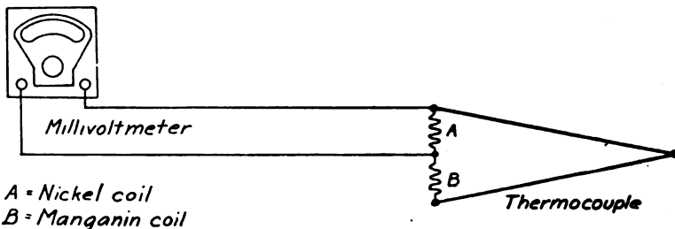
FIG. 3.—USE OF NICKEL AND MANGANIN COILS FOR COMPENSATING FOR COLD-JUNCTION TEMPERATURE CHANGES.
