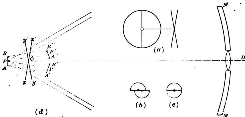
FIG. 14.—OPTICAL SYSTEM OF FERY RADIATION PYROMETER.
