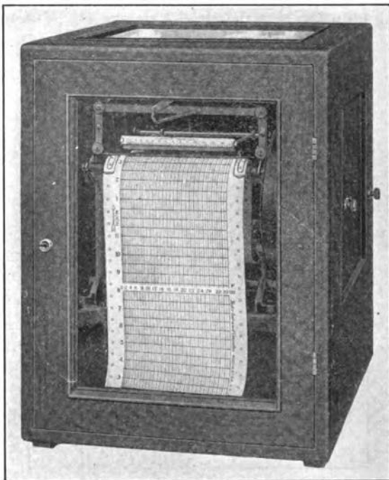
FIG. 9.—THREAD RECORDER.
