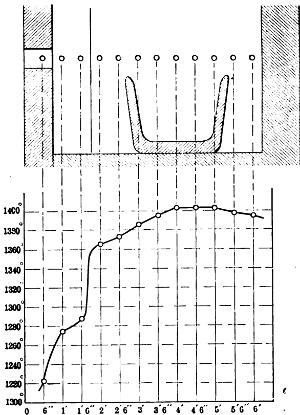
FIG. 2.—CROSS-SECTION OF FURNACE, SHOWING POINTS AT WHICH TEMPERATURE MEASUREMENTS WERE MADE, AND THE CORRESPONDING DISTANCE-TEMPERATURE CURVE.
