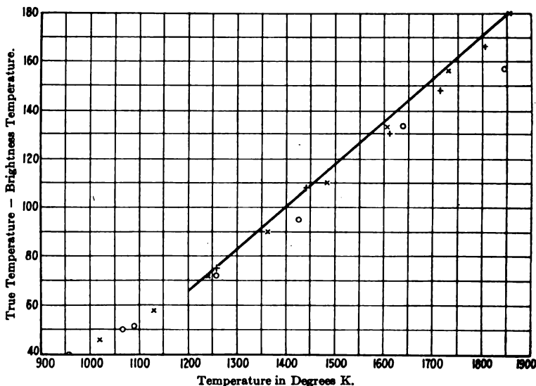
FIG. 5.—BRIGHTNESS TEMPERATURE, TRUE TEMPERATURE RELATIONS FOR PLATINUM ACCORDING TO MEASUREMENTS MADE WITH DISAPPEARING-FILAMENT PYROMETERS WITH RED-GLASS ABSORBING SCREENS. °, HOLBORN AND KURLBAUM; X, WAIDNER AND BURGESS; —, MENDENHALL; +, SPENCE.
