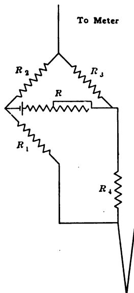
FIG. 1.—DEVICE PERMITTING ACCURATE COMPENSATION FOR TEMPERATURE CHANGES.
