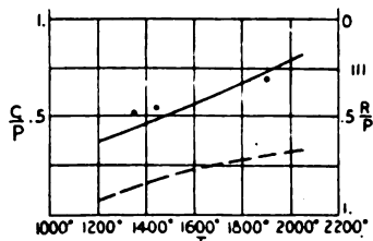
FIG. 1.—CONVECTION LOSSES AS CALCULATED FROM SPECIFIC HEAT OF PRODUCTS: C, CONVECTED ENERGY; P, APPLIED ENERGY; R, RADIATED ENERGY. FULL LINE IS COMBUSTION IN AIR. BROKEN LINE IS COMBUSTION IN OXYGEN.
