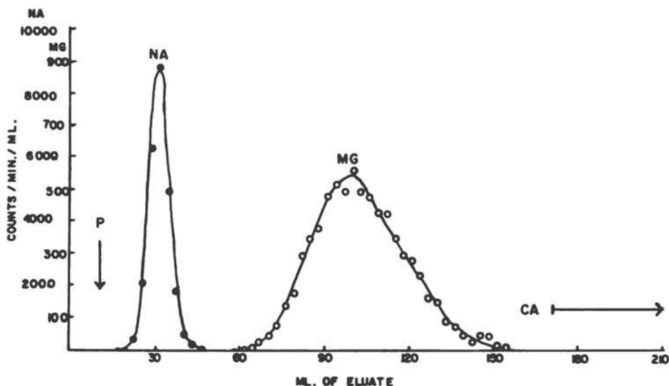
Figure 2. A study of the isolation of magnesium from bone ash solution using tracers for Mg and Na and Dowex 50 resin, 50-100 mesh, in a column 0.5 x 37 cm. An amount of bone ash solution, equivalent to 50-80 mg of dry bone ash, in dilute HCl was passed through the column. The absorbed ions were then eluted with 0.7 N HCl at a flow rate of about 0.7 ml/min. Data of reference 26.
