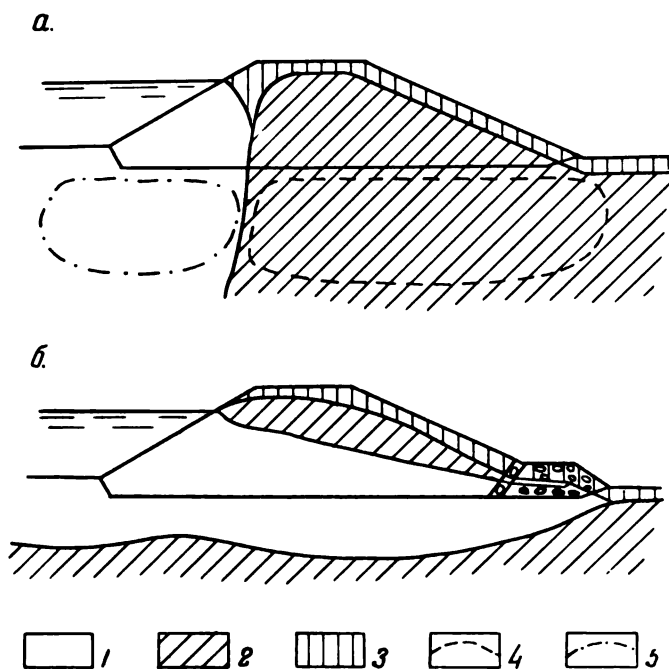
Fig. 1. Typical diagrams of earth dams a. Impervious dam with frozen soil for stability and water tightness. b. pervious dam. 1—zone of permanently thawed soil; 2—zone of permanently frozen soil; 3—zone of alternating thawing and freezing; 4—zone in which it is necessary to freeze naturally unfrozen ground; and 5—zone in which it is desirable to thaw previously
