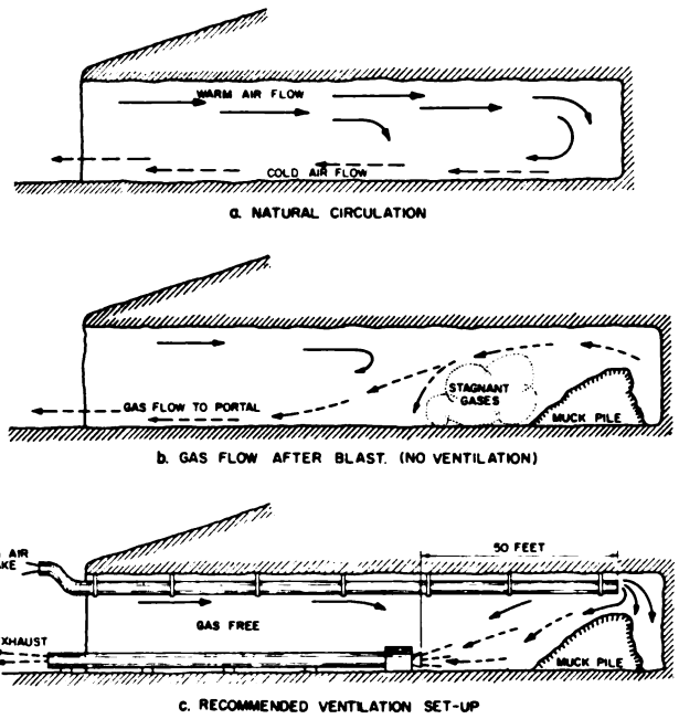
Fig. 4. Summer ventilation in a cold permafrost tunnel
