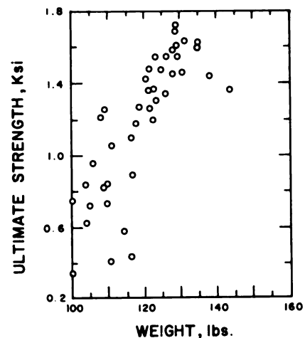
Fig. 8. Relationship between ultimate strength and specimen weight
