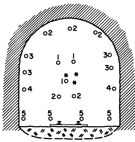
Fig. 2. Tunnel cross section shows the 18 charged holes; numbers indicate firing order; asterisk indicates relief holes; high velocity explosives (indicated by 1) are recommended for use in the burn
