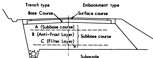
Fig. 4. Trench and embankment types of subbases
