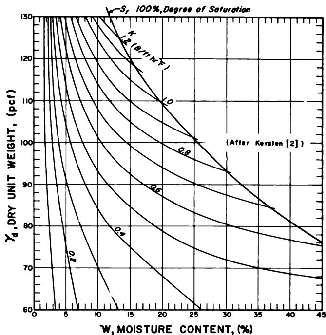
Fig. 4. Dry unit weight, water content, and coefficient of thermal conductivity. Fine-grained soils—unfrozen
