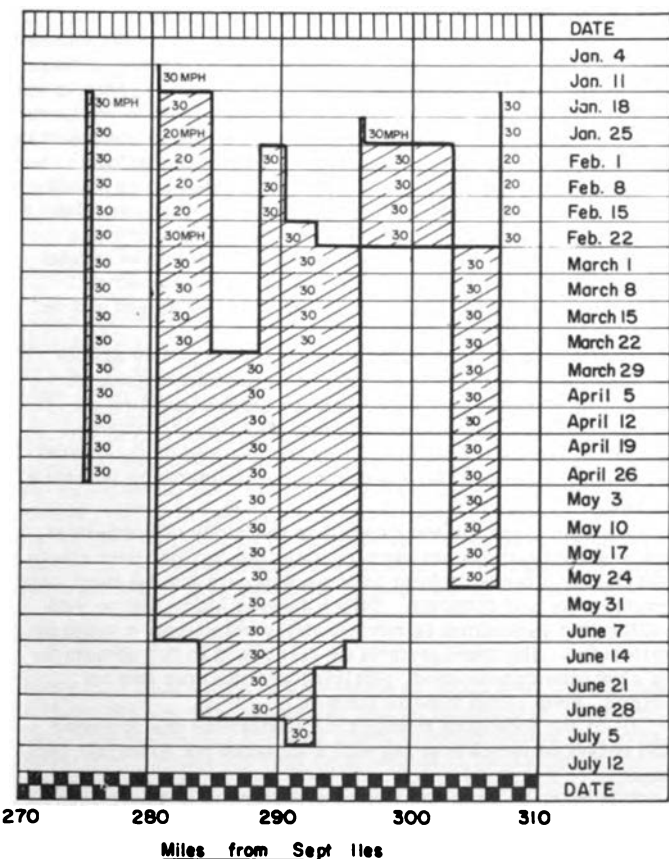
Q.N.S. & L. RAILWAY - MILEPOST 270 TO MILEPOST 310 Fig. 3. Speed restrictions due to frost damage, 1961
