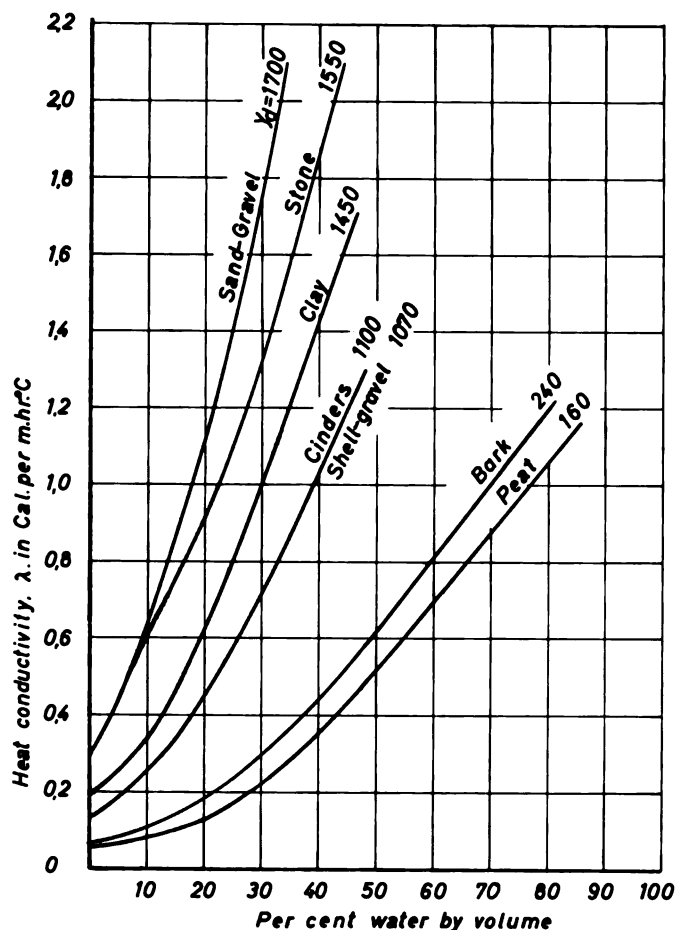
Fig. 1. Heat conductivity of frozen material, mean temperature -5^{\circ}\text{C}
