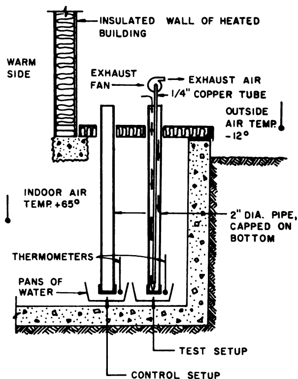
Fig. 1. Experiment in pile freezing using air as heat transfer media
