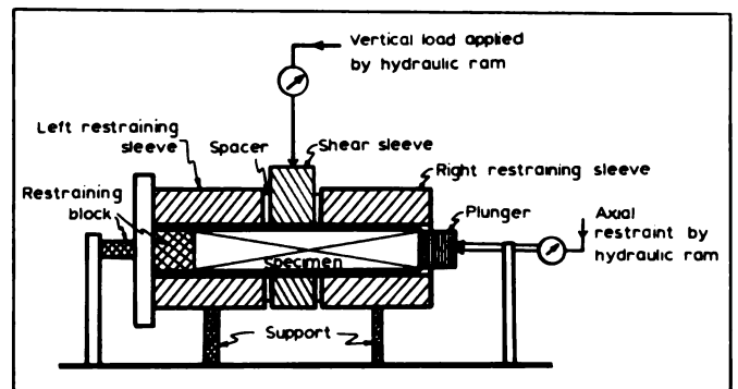
Fig. 1. Schematic picture of ring shear tester
