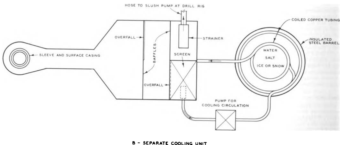
Fig. 10. Arrangements for cooling drilling fluid
