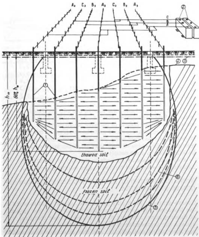
Fig. 3. Bed preparation by the electrical method (thawing stage). A, B, C, are rows of electrodes uniformly distributing the load by phases. 1. Iron pipe electrodes; 2. Step-down transformers; 3. Water table; 4. Upper surface of permafrost; 5. Outline of limit of thawing bowl during the period of use; 6. Changes of the thawing bowl with time
