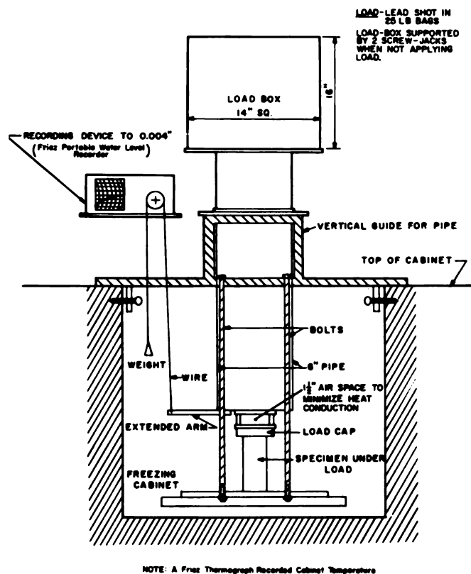
Fig. 1. Diagram of test apparatus for plastic deformation tests
