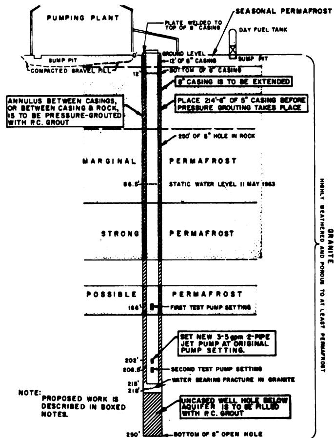
Fig. 6. Diagrammatic sketch of casing and cement (vertical scale, 1 in. = 30 ft)
