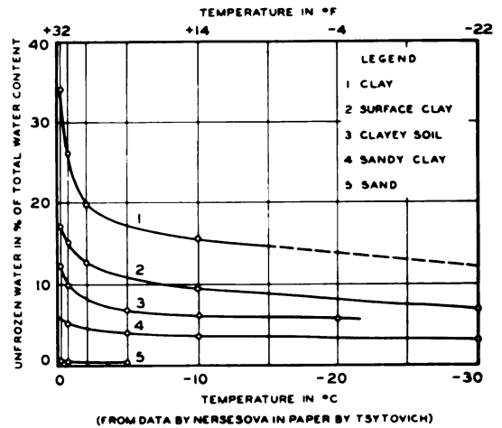
Fig. 2. Unfrozen water content of frozen soils
