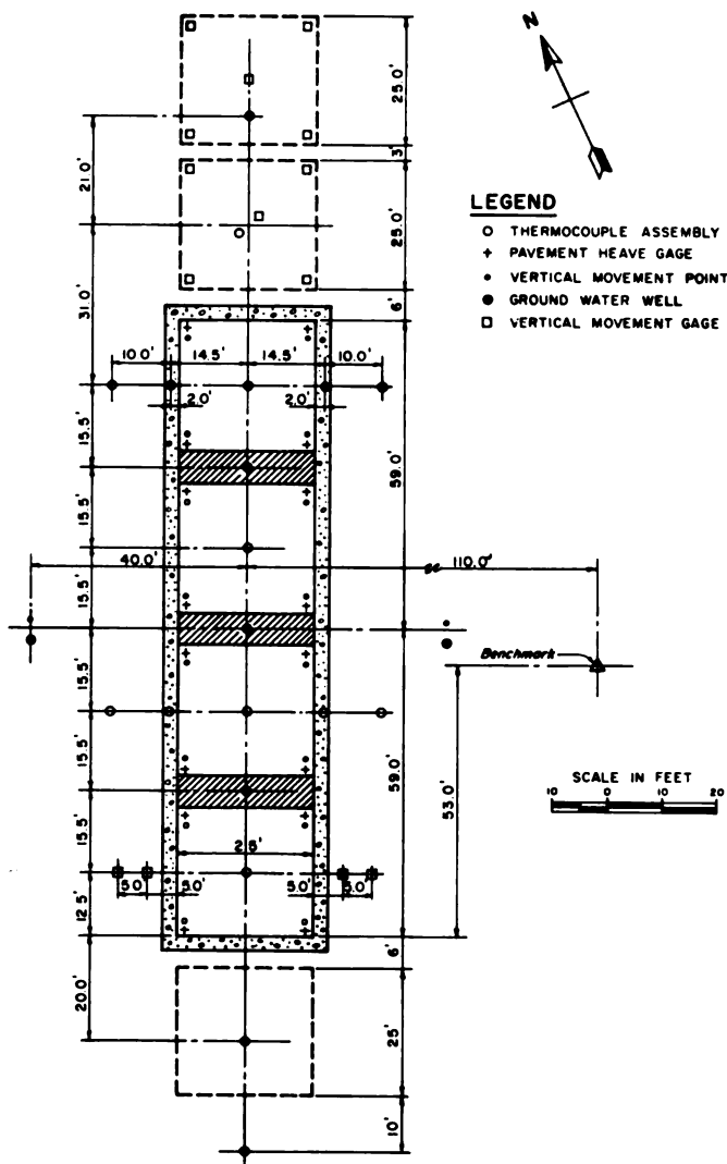
Fig. 3. Instrumentation layout
