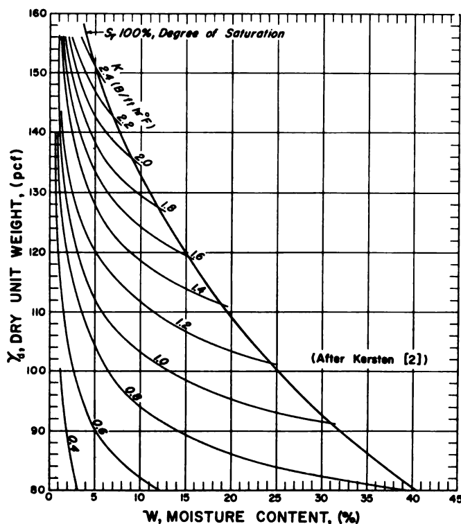
Fig. 2. Dry unit weight, water content, and coefficient of thermal conductivity. Coarse-grained soils—unfrozen
