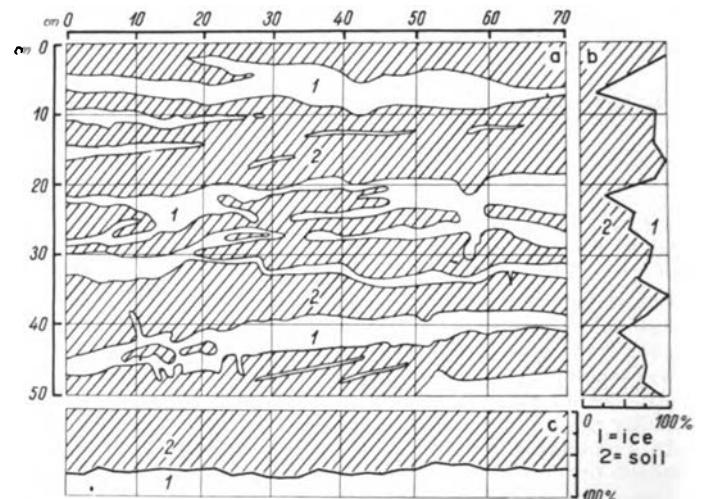
Fig. 1. Typical texture of frozen clay-loam: (a) Distribution of ice-lenses in vertical section; (b) Percentage of ice along vertical; (c) Percentage of ice along horizontal
