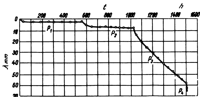
Fig. 3. Settlement versus time curve for incremental load testing of a pile
