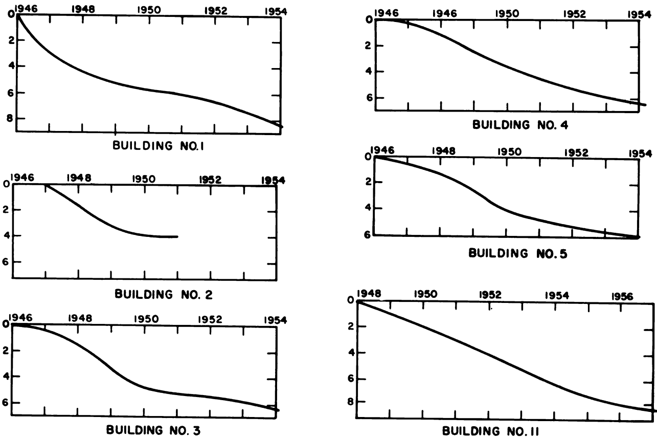
Fig. 4. Permafrost degradation beneath center of buildings on gravel fills of various thicknesses
