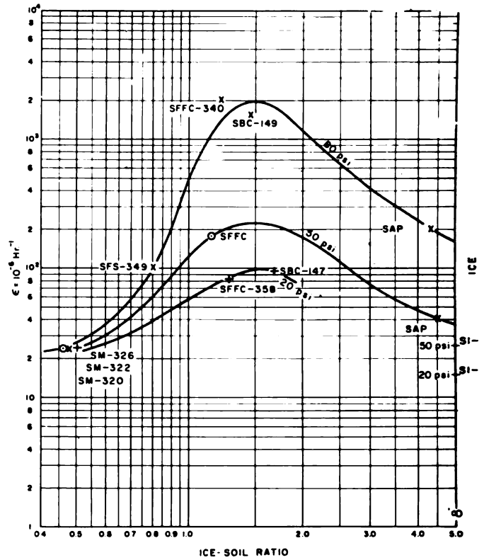
Fig. 11. Rate of strain-volumetric ice-soil ratio at 28°F
