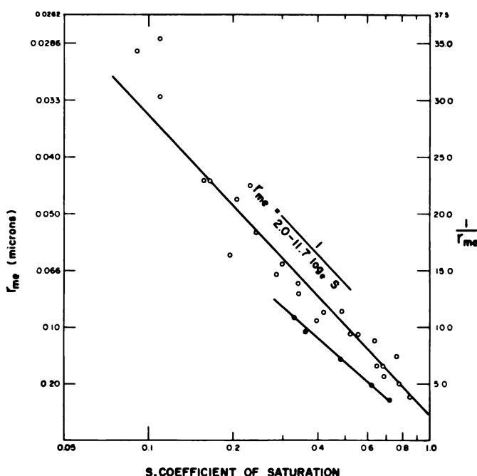
Fig. 7. Pore size vs. saturation calculated from freezing-point depression and from capillary head
