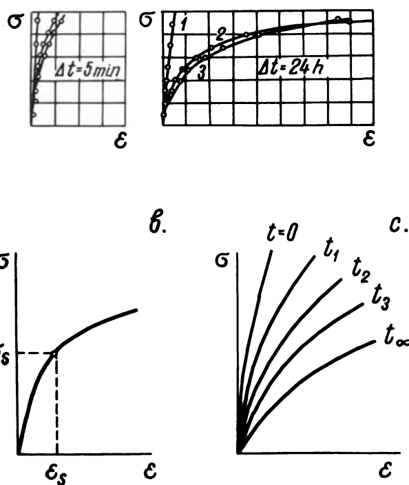
Fig. 3. Curves showing relation between stress ( \sigma ) and deformation ( \epsilon ) of frozen soil: a—division of total deformation (3) into recoverable (1) and nonrecoverable (2) parts for different durations of load; b—schematic curve; c—group of curves for various durations
