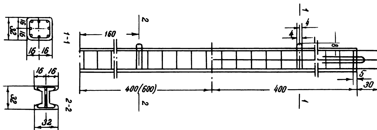
Fig. 9. Square double-T pile
