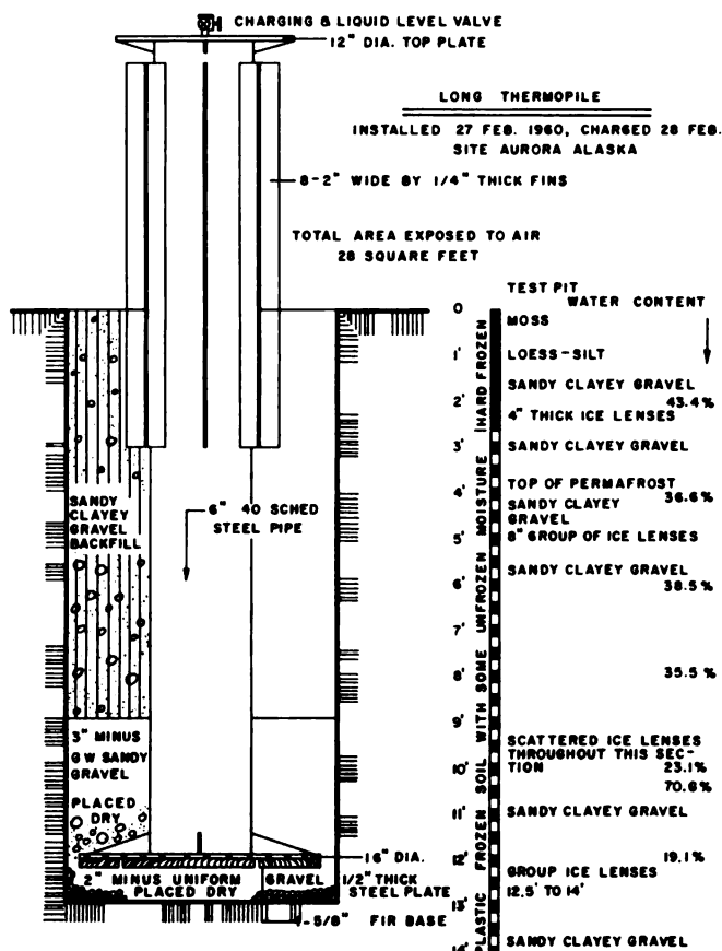
Fig. 1. Long thermopile at Aurora, Alaska
