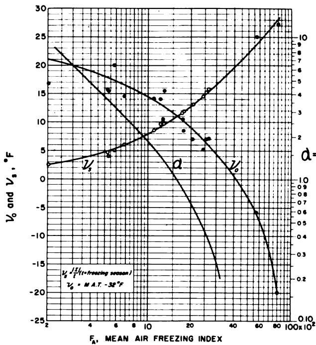
Fig. 7. Air freezing index and temperature parameters
