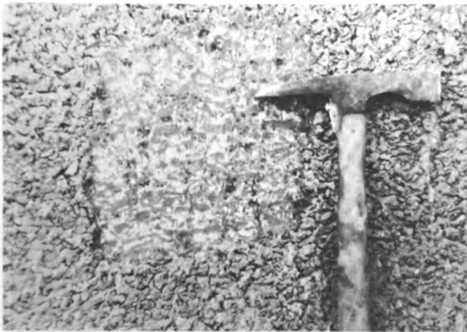
Fig. 2. Typical structure of the ice of a lens in the interior of a palsen-like mound in the border zone of a polygon
