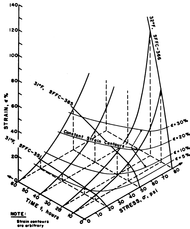
d. TIME-STRESS-STRAIN at 31°F and 32°F
