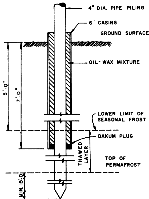
Fig. 2. Sleeves through the active layer around piles in permafrost
