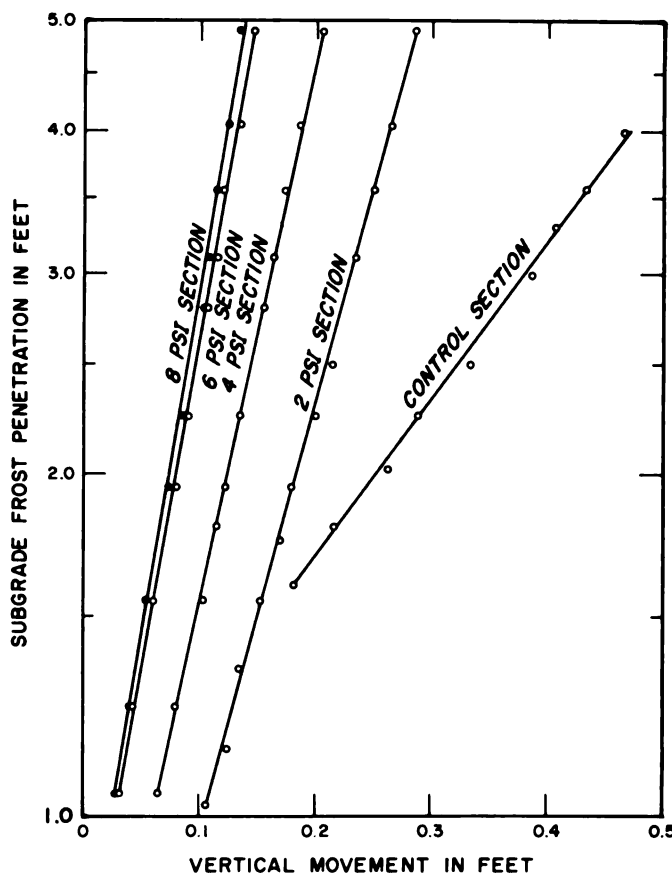
Fig. 15. Frost penetration versus heave 1962 to 1963
