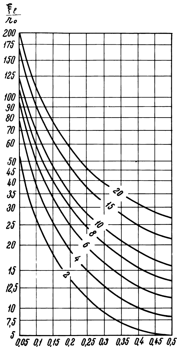
Fig. 3. Thawing limit under center of tube with different values of m
