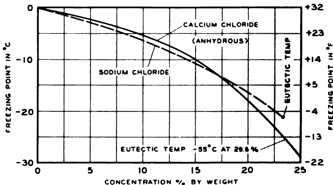
Fig. 8. Freezing temperatures of brines
