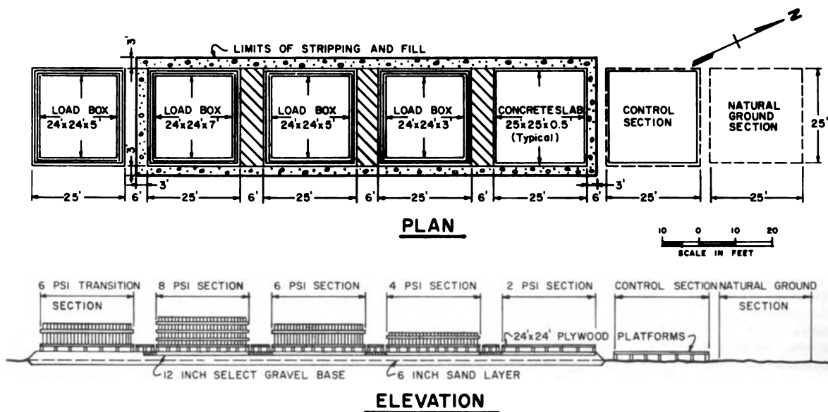
Fig. 2. Test section
