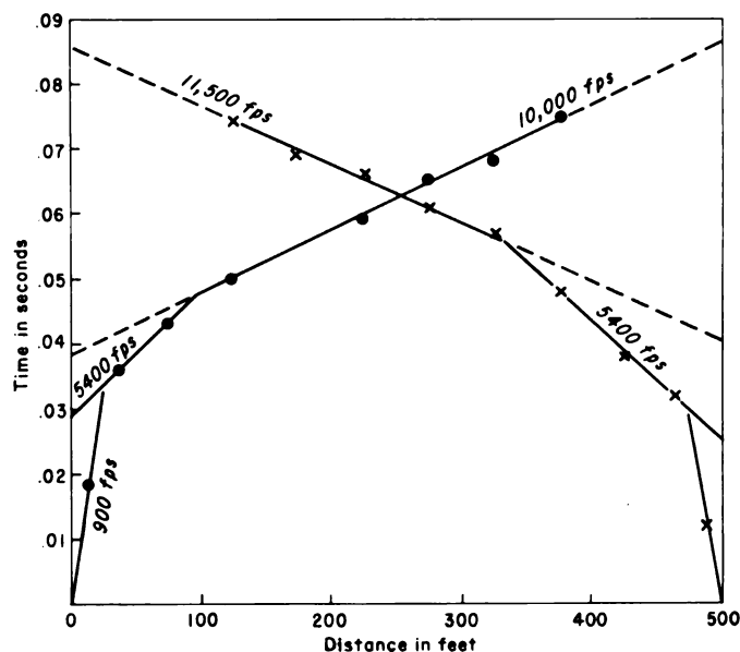
Fig. 4. Seismic travel-time curves near Fairbanks, Alaska, showing 15 ft of dry alluvium (velocity 900 ft/sec), overlying about 40 ft of water-saturated sediments (velocity 5,400 ft/sec), above permafrost (velocity 10,750 ft/sec) (author's 1952 data)
