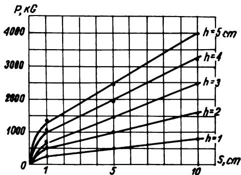
Fig. 2. Forces of cutting as related to depth of cutting and width of cutter
