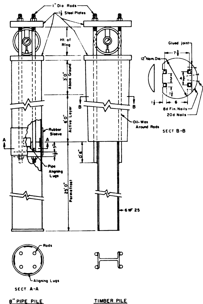
Fig. 7. Construction details of test piles for measurement of frost thrust
