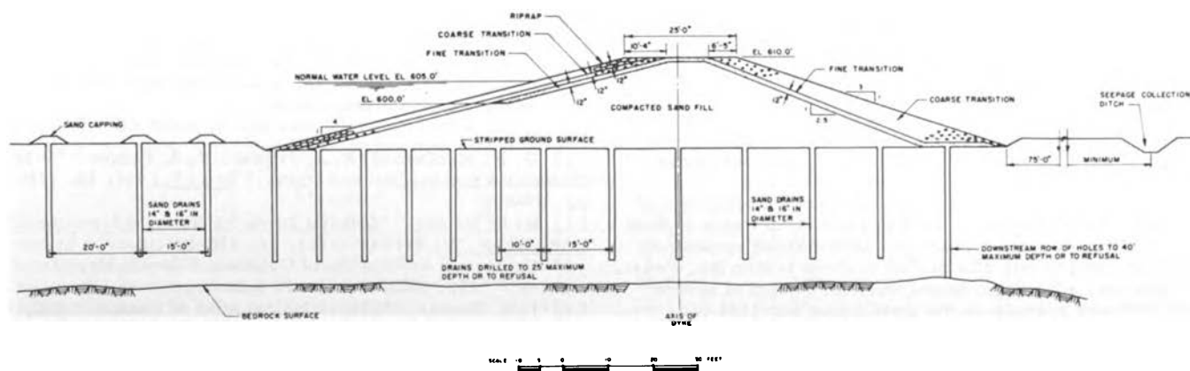
Fig. 6. Typical section through No. 2 east and No. 2 west
