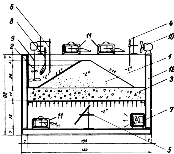
Fig. 5. Diagram of dam model: 1—body of dam made of fine-grained sand; 2—water; 3—concrete; 4—thermometer for air; 5—base plate thermometer; 6—water thermometer; 7—heat ventilator; 8—electric heater for water; 9—mixer for water; 10—ventilator for mixing air in chamber; 11—thermographs; and 12—foam plastic
