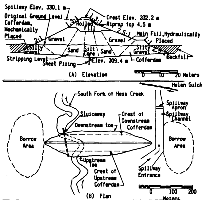
Fig. 2. Plan and typical elevation of Hess Creek Dam
