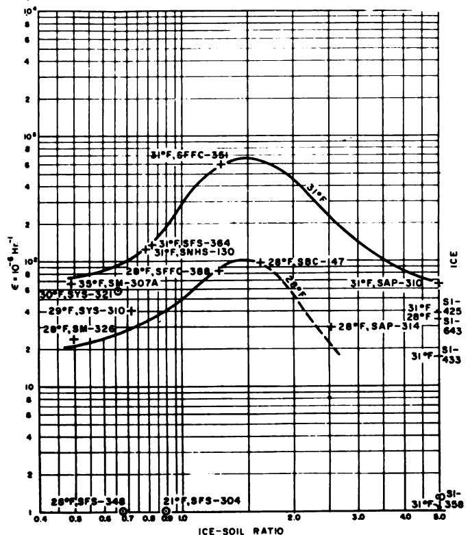
Fig. 9. Rate of strain-volumetric ice-soil ratio at 20 psi
