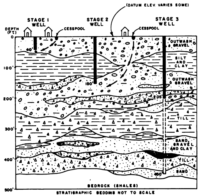
Fig. 3. Well development, Anchorage area (vertical scale, 0.5 in. = 1 ft)
