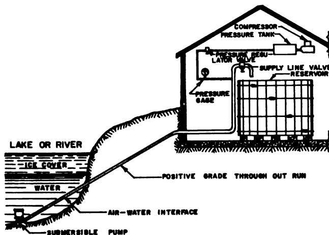
Fig. 1. Air-lock water pump supply for intermittent operation
