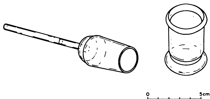
Fig. 2. Pycnometer used for dry density determinations
