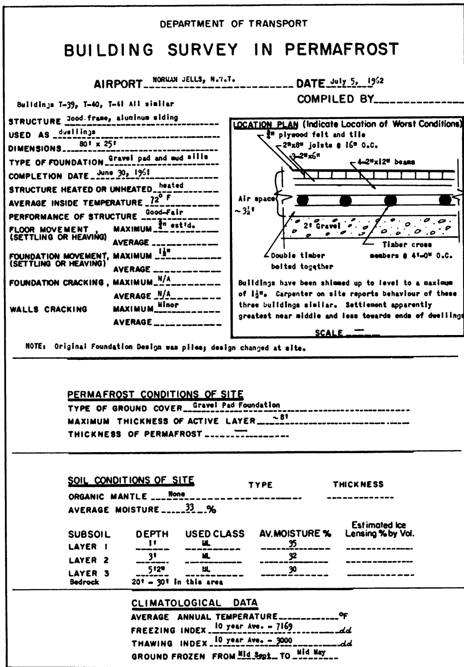
Fig. 5. Building survey in permafrost
