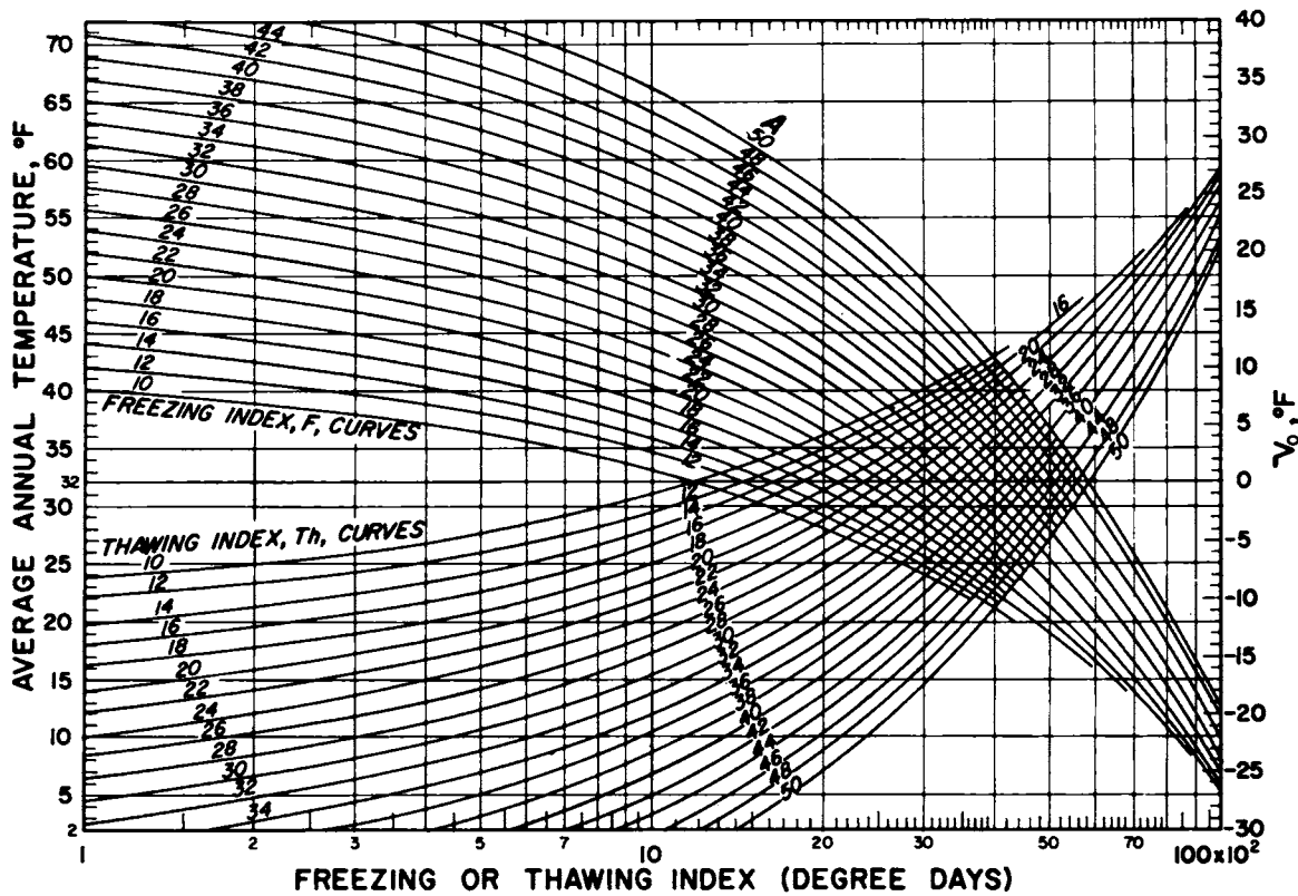
Fig. 14. Frost penetration in uniform soils under various surface conditions
