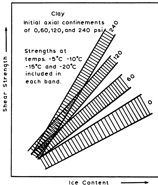
Fig. 11. Ice content and shear strength
