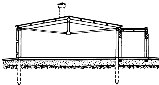
Fig. 7. Stepdown substation on pile foundation
