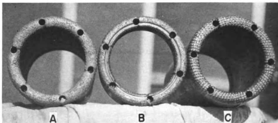
Fig. 7. Bottom discharge diamond coring bits: (A) Run 67 ft, worn bit; (B) Run 35 ft, damaged bit; and (C) Run 86 ft, good condition
