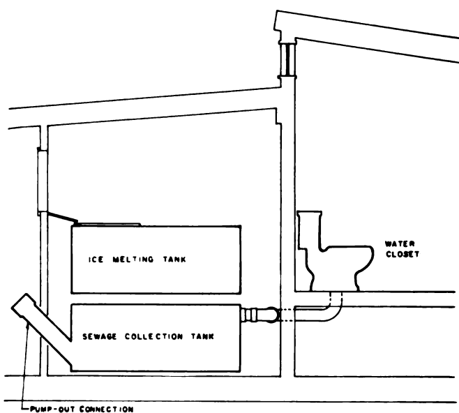
Fig. 3. Typical plumbing layout for trucked system
