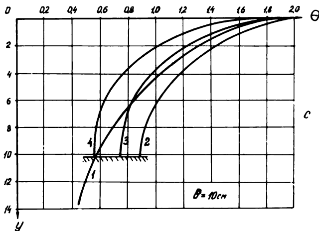
Fig. 3. Nonuniformity in consolidation (expressed as void ratio \Delta e ) and distribution of the sum of principal stresses \theta with depth y in thawing frozen clay
