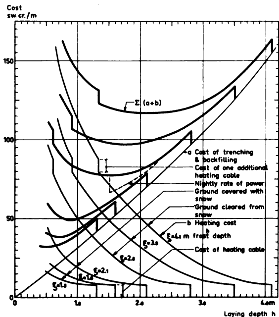
Fig. 2. Relation between cost, laying depth and frost depth in sandy-silty moraine
