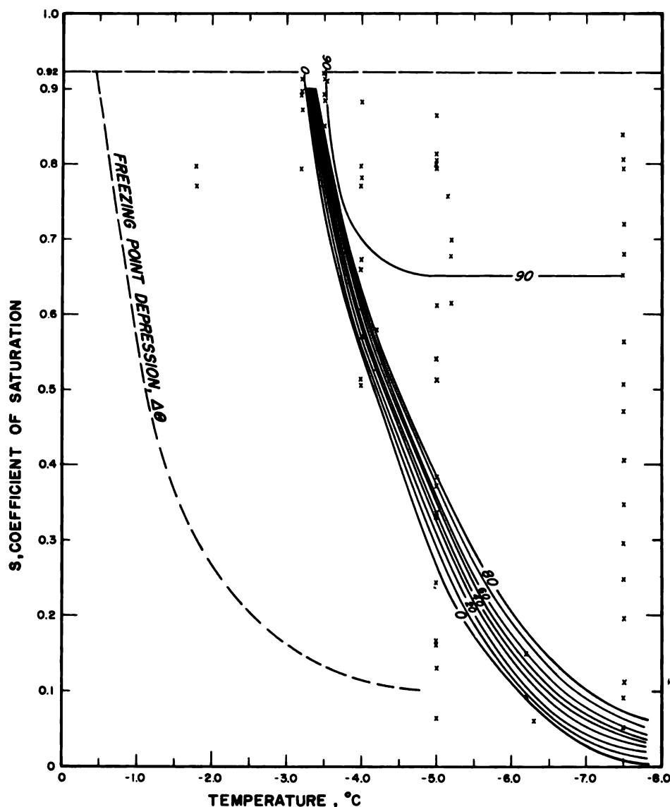
Fig. 5. Combined effect of saturation and temperature upon the per cent of original water frozen. Elevation is per cent frozen
