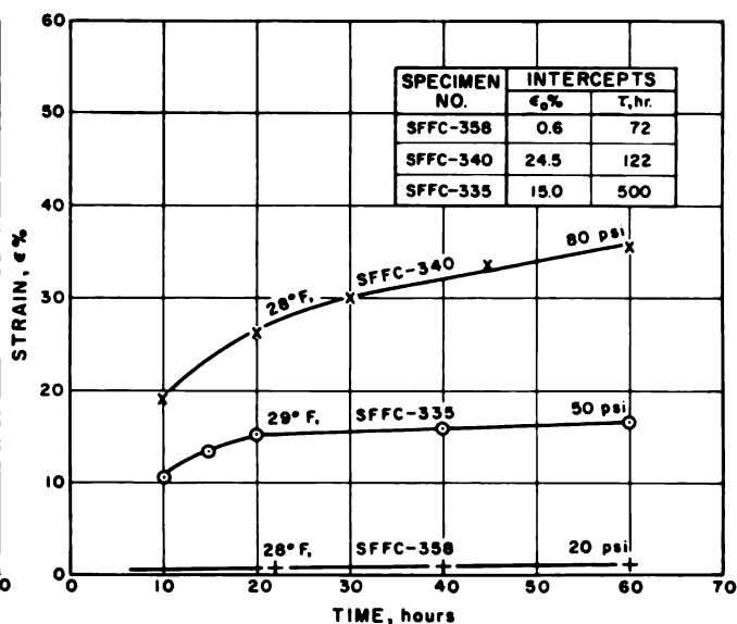
b. STRAIN-TIME at 28°F and 29°F
