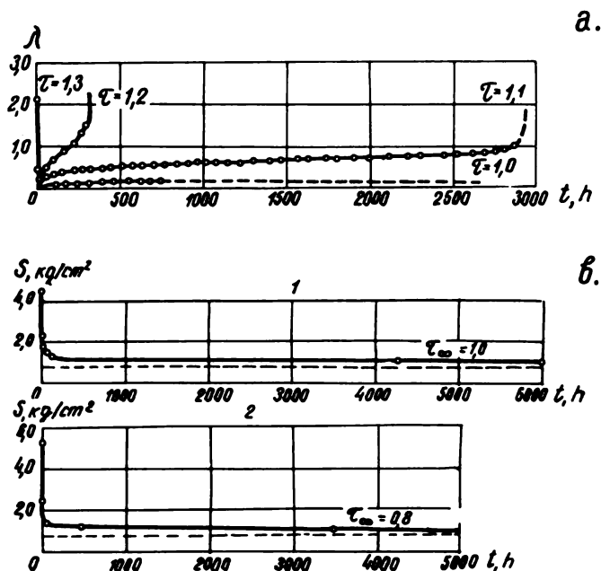
Fig. 2. Pull-out resistance testing of rods embedded in frozen soil: a. Creep curves, b. ultimate strength curves; 1 - silty soil, -0.4^{\circ}\text{C} , rods driven into small diameter boreholes; 2 - the same, rods frozen into soil
