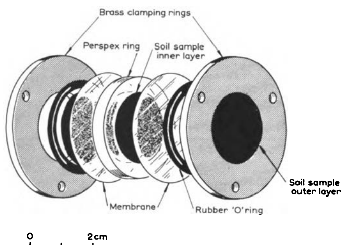
Fig. 1. Sample assembly for freezing experiments
