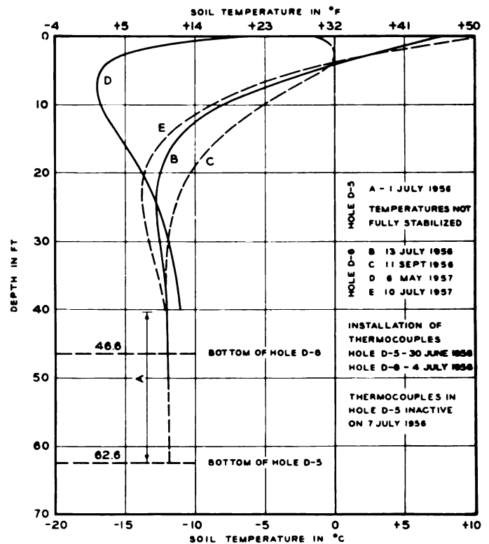
Fig. 3. Soil temperatures in bore holes 5 and 6 at Tuto
