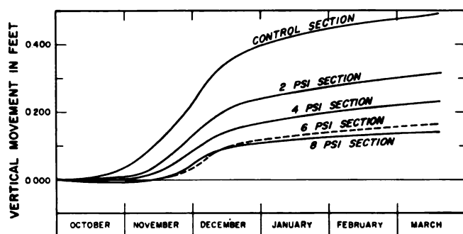
Fig. 12. Heave-time curves, 1962 to 1963 freezing season
