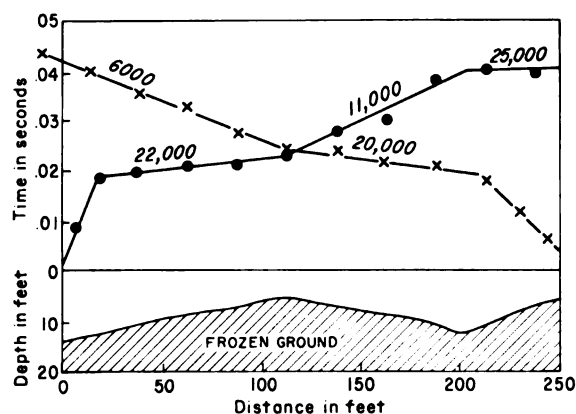
Fig. 3. Seismic travel-time curves and apparent velocities at Eielson Field, Alaska, showing irregular top of permafrost (author's 1952 data)
