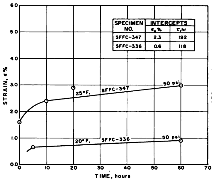
a. STRAIN-TIME at 20°F and 25°F
