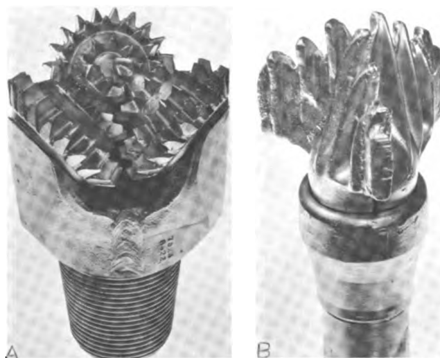
Fig. 4. Drilling bits: (A) Tricone rock bit; (B) Hawthorne bit
