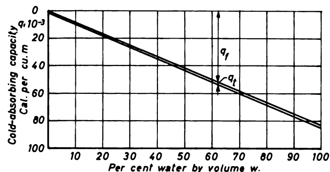
Fig. 2. Frost-storing capacity q = q_f + q_t computed for the temperature interval +2^{\circ}\text{C} to -2^{\circ}\text{C} , where q_f is due to water and q_t to dry material; q_t is maximum value of the materials investigated (found in cobble stones). The minimum value (dried peat) is about 1/10 of the maximum
