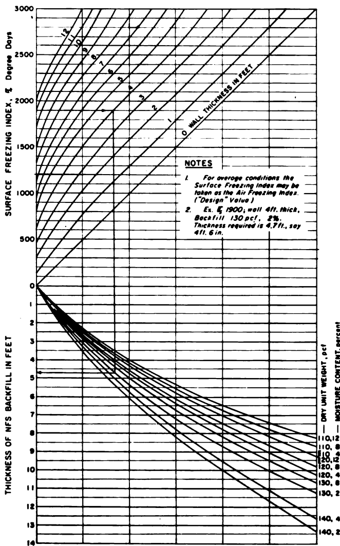
Fig. 17. Concrete retaining walls and nonfrost-susceptible backfills
