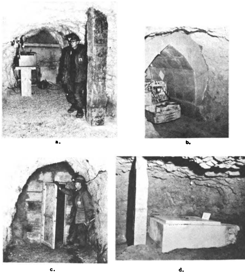
Fig. 5. Application of artificial frozen soil mixtures: a. Column supporting a loose roof slab; b. tunnel section protected by a combination of poured permacrete and pre-cast bricks; c. bulkhead made of large precast bricks; d. diesel fuel storage pit poured in place and lined with fine grain frozen material. Finish: Clay slurry applied with paint brush
