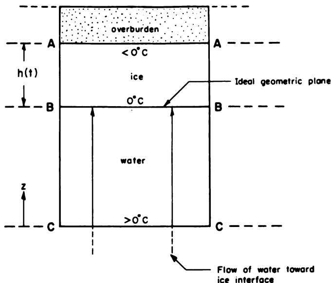
Fig. 3. Simple frost-heaving
