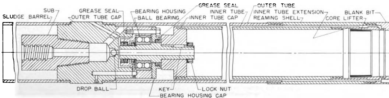
Fig. 5. Standard double tube core barrel
