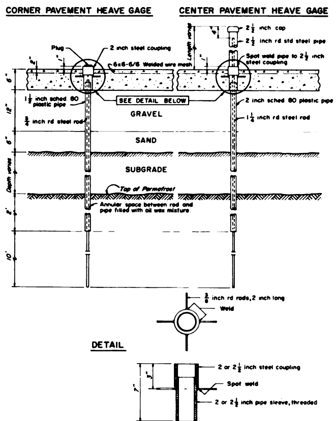
Fig. 4. Heave gage details
