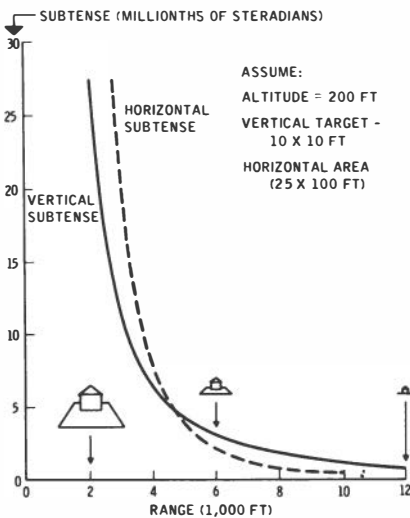
FIG. 5. Apparent size of horizontal and vertical surfaces.
