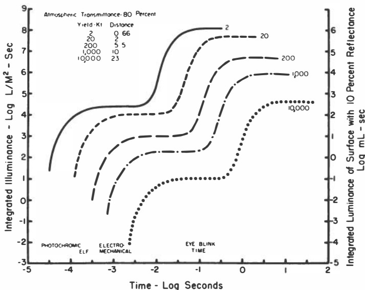
FIG. 11. Integrated fireball illuminance for five weapon yields at minimum safe distances and integrated luminance of 10 per cent reflecting surface at 80 per cent atmospheric transmission.
