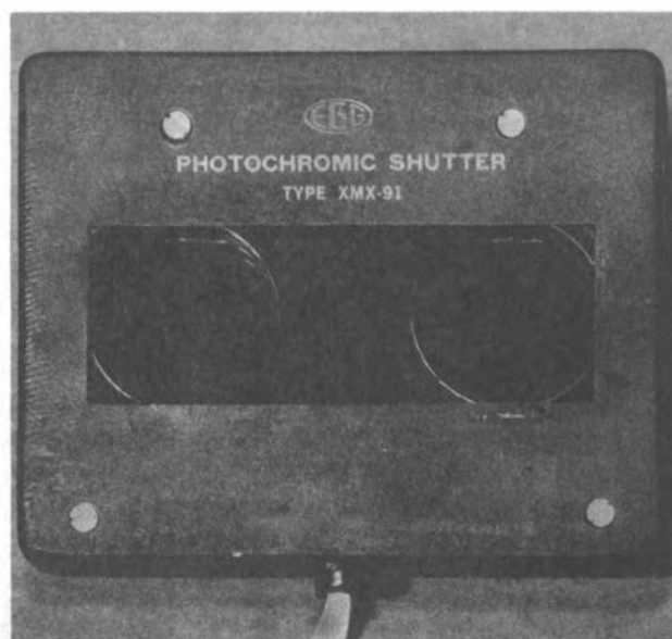
FIG. 4. First photochromic shutter designed for a periscope.
