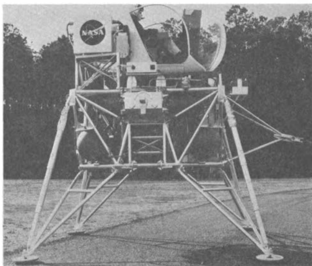
FIG. 10. General research vehicle for Landing Research Facility.
