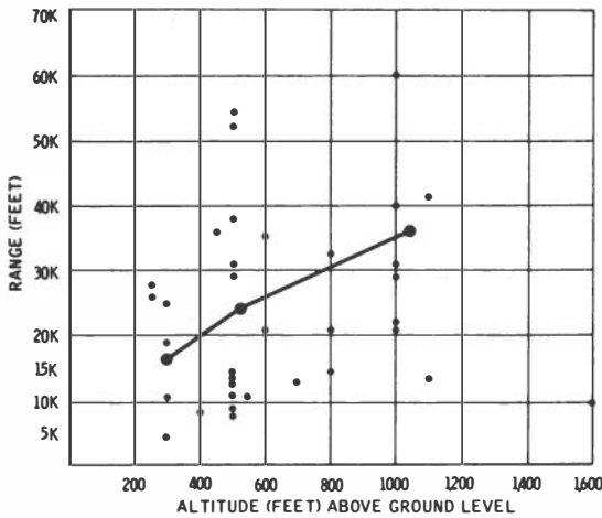
FIG. 10. Data points and mean recognition ranges.
