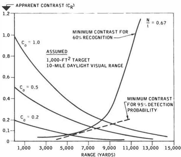
FIG. 6. Recognition range and apparent contrast.
