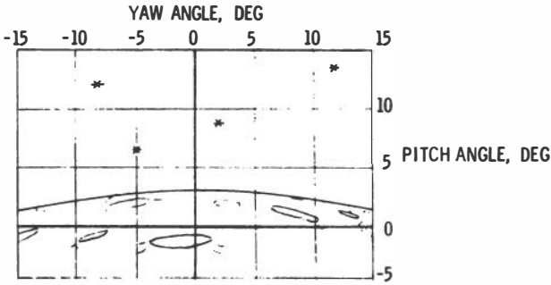
FIG. 6. Window for vehicle alignment.
