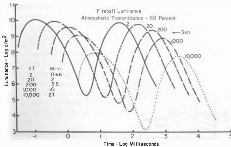
FIG. 6. Fireball luminance for five weapon yields at minimum safe distance with 80 per cent atmospheric transmittance.
