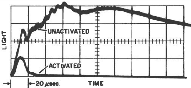
FLASHTUBE VIEWED THROUGH PERISCOPE SHUTTER
