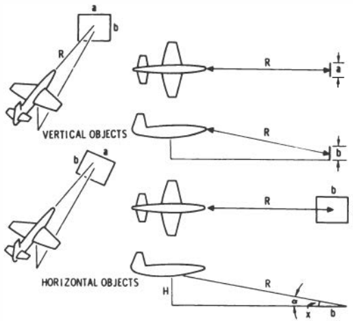
FIG. 4. Subtense of distant objects.
