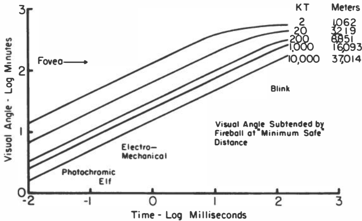
FIG. 9. Visual angles subtended by fireball of five weapon yields at minimum safe distances.
