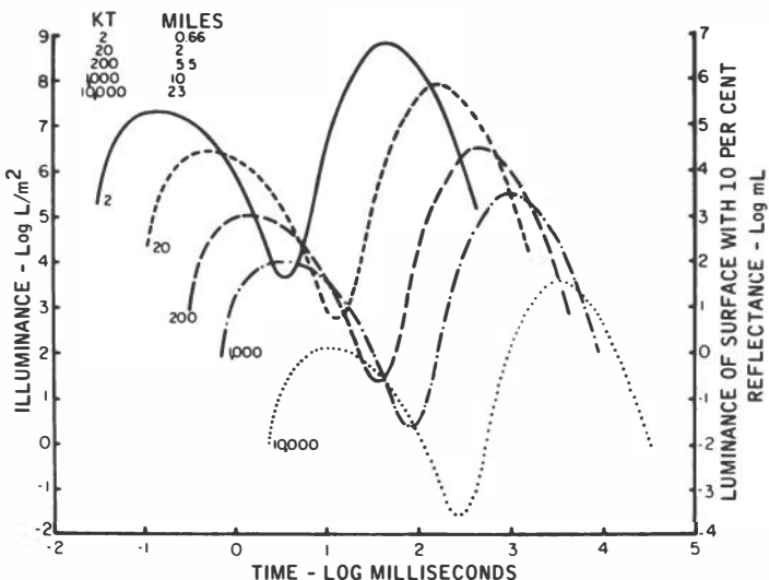
FIG. 10. Fireball illuminances for five weapon yields at minimum safe distance and luminances of 10 per cent reflecting surface at 80 per cent atmospheric transmission.
