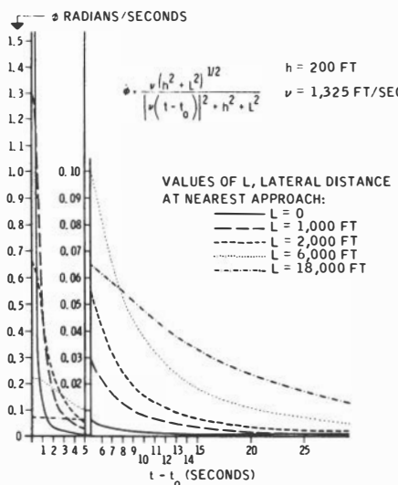
FIG. 2. Apparent angular motion of ground objects.
