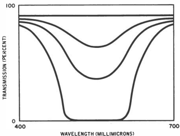
FIG. 1. Behavior of a typical photochromic dye.
