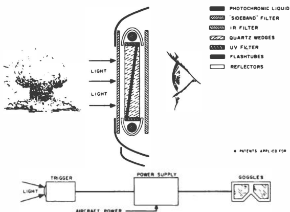
FIG. 2. Schematic diagram, photochromic goggle system.
