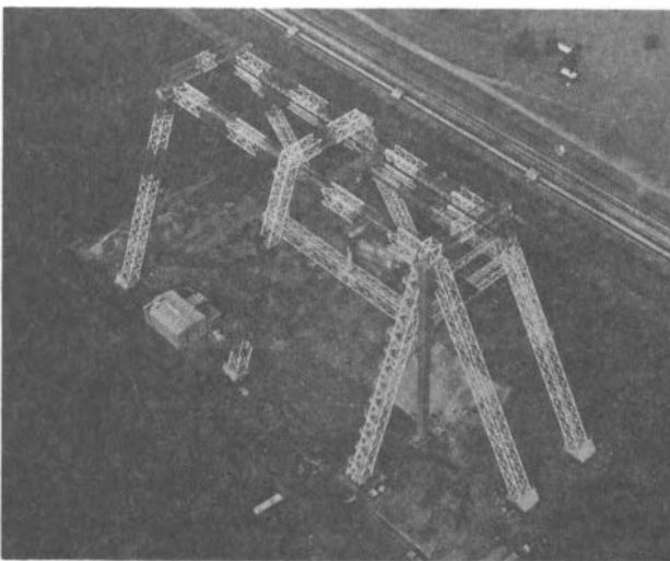
FIG. 9. Lunar Landing Research Facility.
