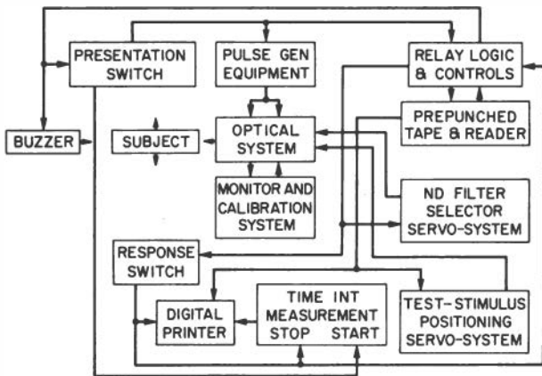
FIG. 1. Block diagram of experimental system.
