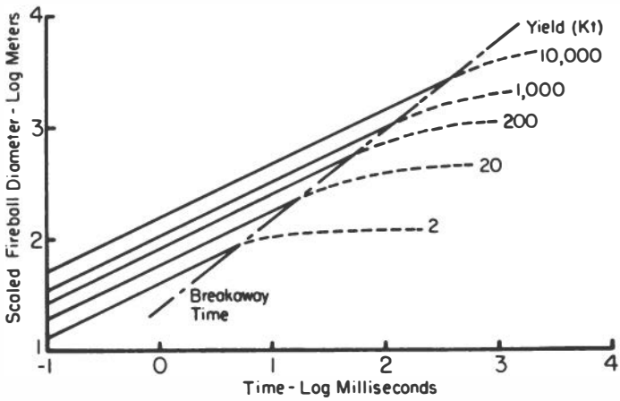
FIG. 8. Fireball diameters for five weapon yields.
