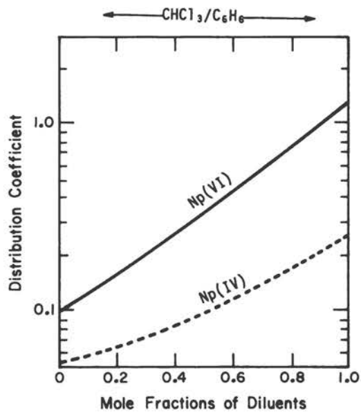
Figure 16. Neptunium Extraction with TBP from 5M HNO 3 into Diluent Mixtures. 203
