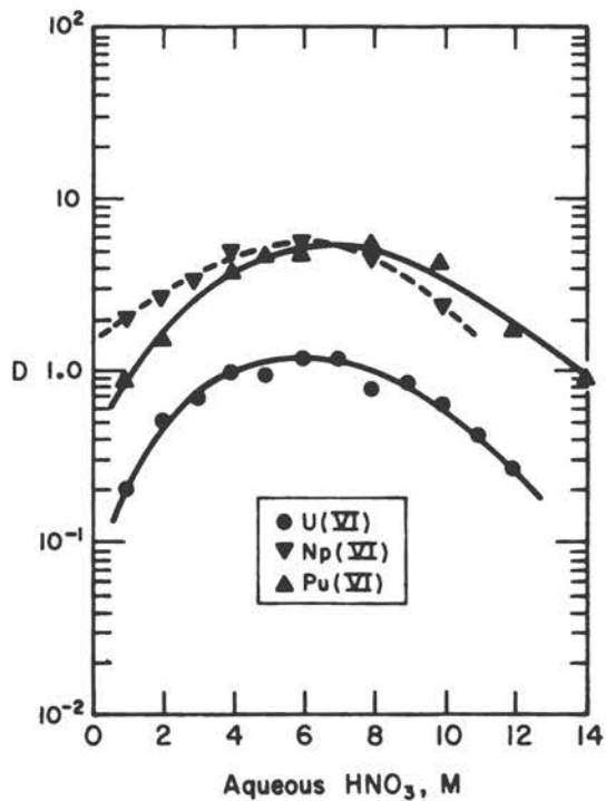
Figure 12. The Extraction of the Hexavalent Actinide Nitrates by 10 vol % TOA in Xylene. 190
