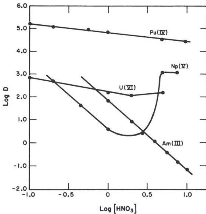
Figure 10. Extraction of Various Actinides into 0.2M H 2 MEHP (Isooctane diluent) from HNO 3 Solutions. 179
