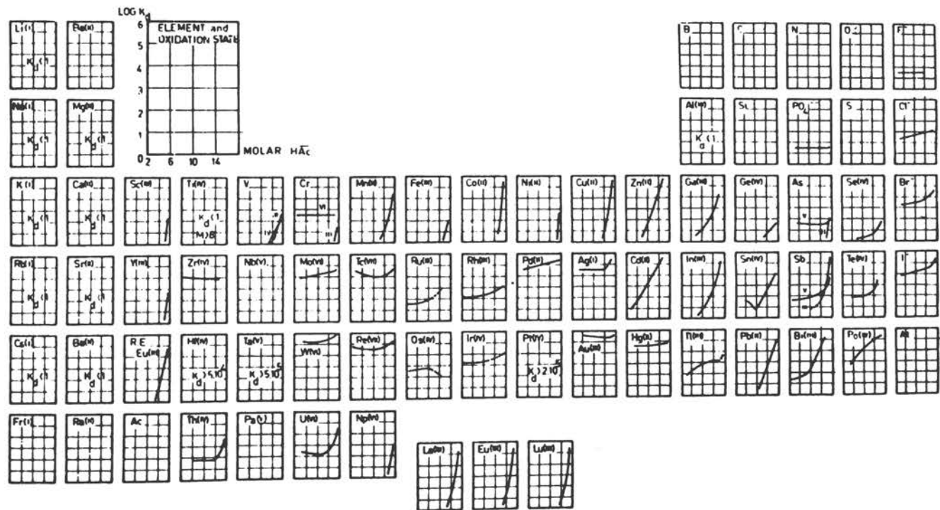
Figure 20. Sorption of the Elements from Acetic Acid Solutions by an Anion-Exchange Resin. 221
