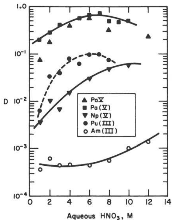
Figure 13. The Extraction of Pentavalent and Trivalent Actinide Nitrates by 10 vol % TOA in Xylene. 190
