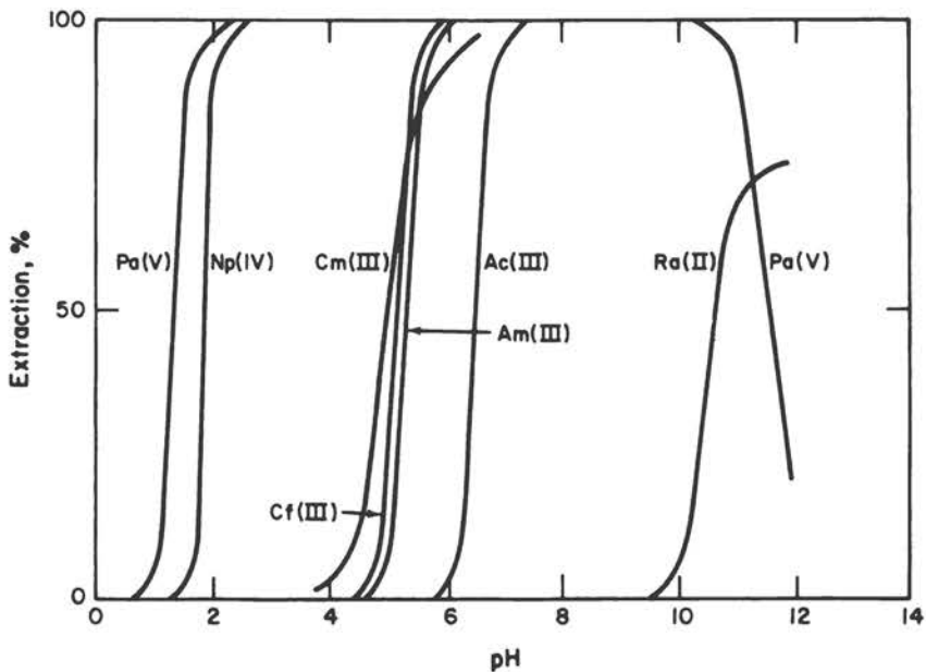
FIGURE 4. Percentage Extraction of Tracer Quantities of Ac(III), Am(III), Cm(III), Cf(III), Np(IV), and Pa(V) with 0.1M 8-Hydroxyquinoline/CHCl 3 and of Ra(II) with 1.0M 8-Hydroxyquinoline/CHCl 3 , [ \mu = 0.1M (Na, NH 4 , H)C10 4 , 25°C]. [C. Keller and M. Mosdzelenki, Radiochim. Acta. 7, 185(1967) Supplemented].
