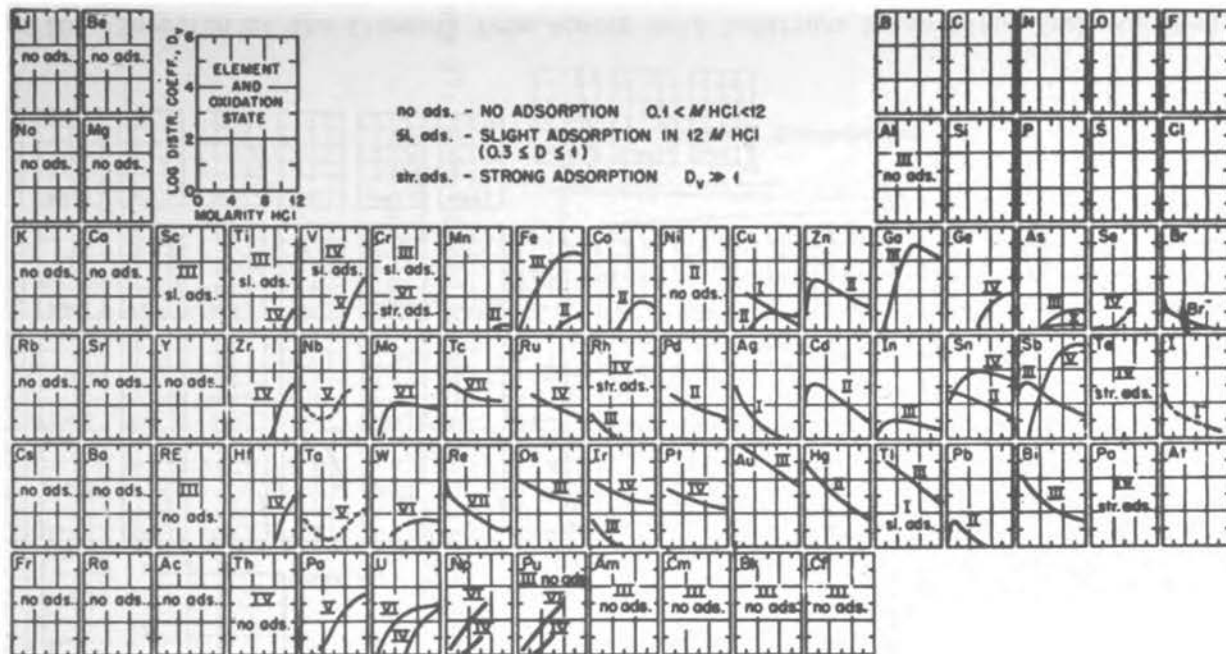
Figure 19. Sorption of the Elements from Hydrochloric Acid Solutions by Strongly Basic Anion Exchange Resins. 219
