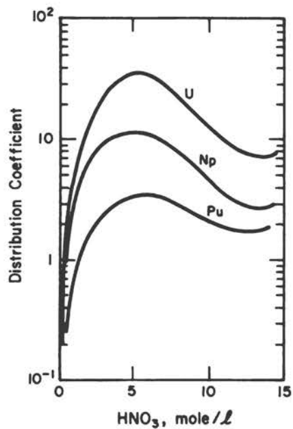
Figure 6. Distribution Coefficients for the Extraction of Hexavalent Actinides by 19 vol % TBP-Kerosene from Nitric Acid Solution. 165
