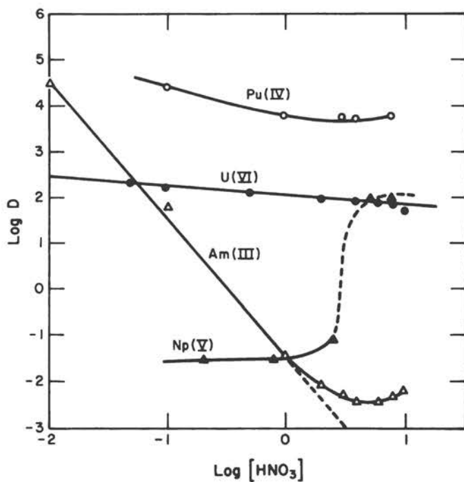
Figure 8. Extraction of Various Actinides into 0.5M HDEHP (isooctane diluent) from HNO 3 Solutions. 179
