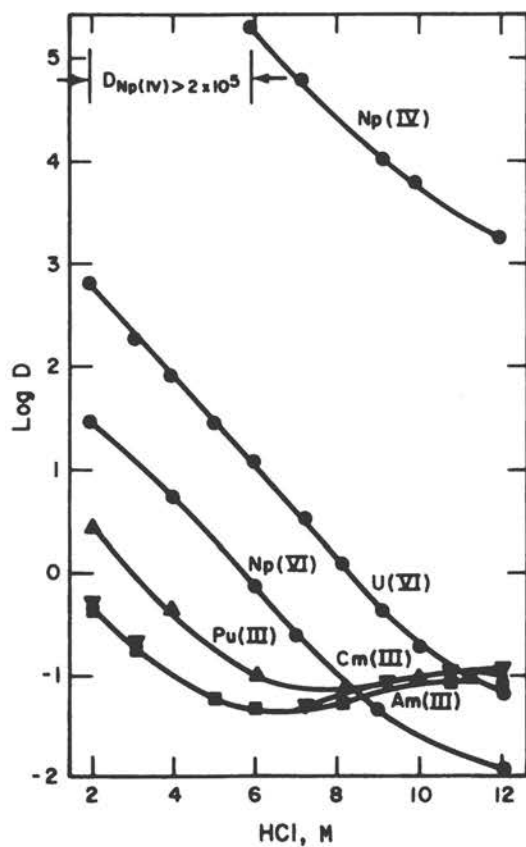
Figure 9. Extraction of some Actinide Cations into 0.48M H 2 MEHP in Toluene as a Function of HCl Concentration. 177
