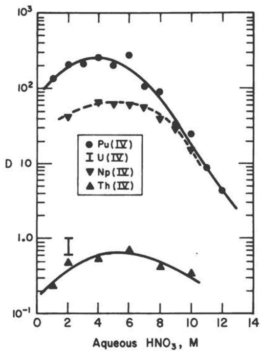
Figure 11. The Extraction of the Quadivalent Actinide Nitrates by 10 vol % TOA in Xylene. 190
