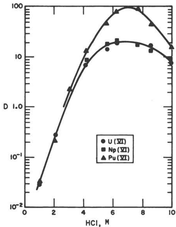
Figure 15. Extraction of Hexavalent U, Np, and Pu from HCl Solution with 1.0% TOA in Xylene. 199
