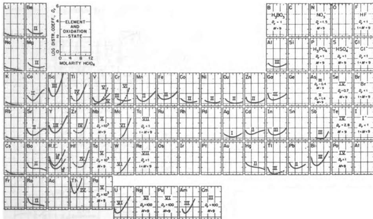
Figure 26. Sorption of the Elements from \text{HClO}_4 Solutions by a Cation Exchange Resin. 238
