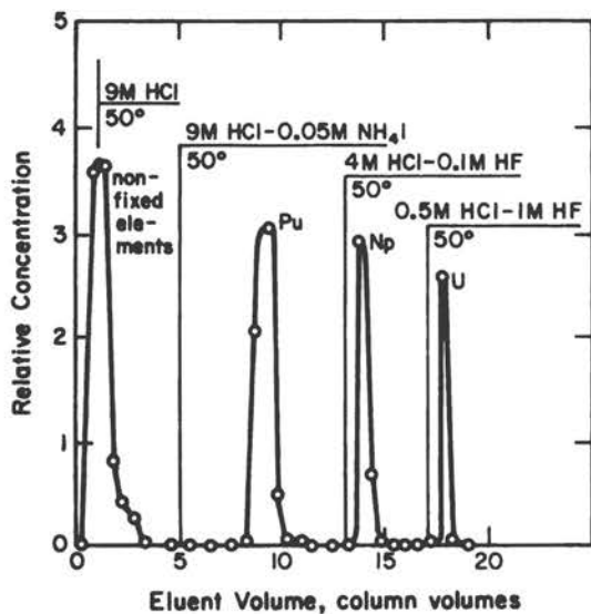
Figure 21. Uranium-Neptunium-Plutonium Separation by Anion Exchange ("Dowex" 1-X10, <400 Mesh, 0.25 cm 2 × 3 cm Column). 225
