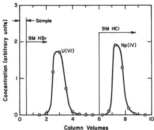
Figure 22. Separation of U(VI) and Np(IV) by Cation Exchange ("Dowex" 50-X4 0.2 cm 2 × 2 cm Column, 25°). 2,37
