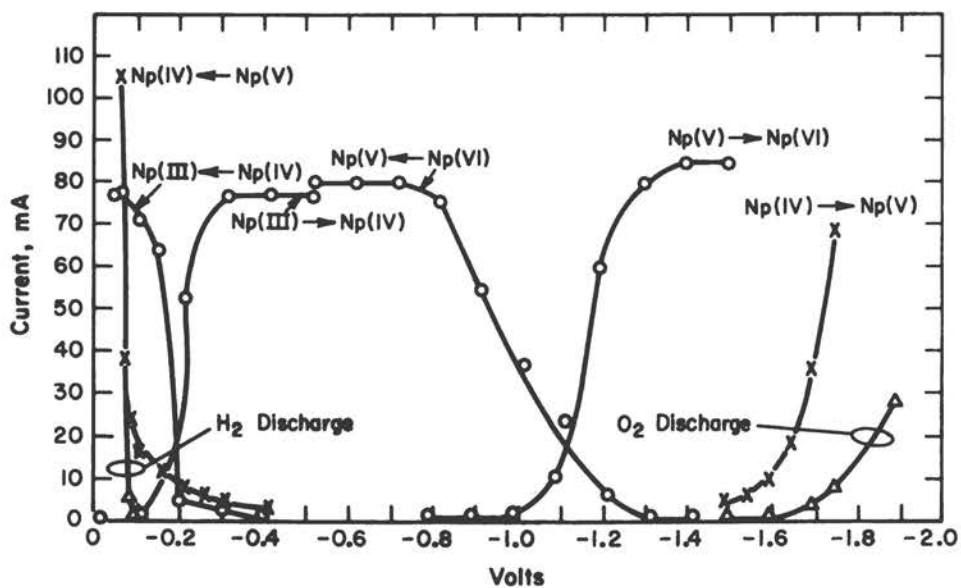
Figure 2. Current-Voltage Curve for Redox Reactions of Neptunium. 71
