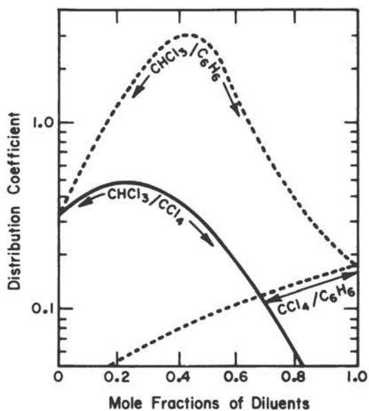
Figure 17. Distribution Coefficients for Np(IV) Extraction with 10^{-2}M Tetrabutyl-Ammonium Nitrate from 3M HNO_3 Using Mixtures of Different Diluents. 2,3
