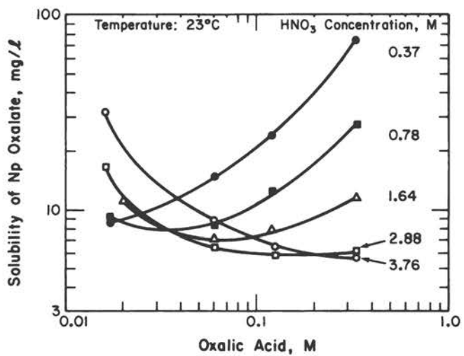
Figure 3. Solubility of Np(IV) Oxalate
