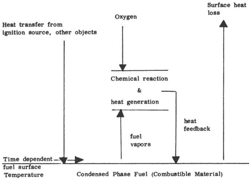
Figure 1. Physical process in gas-phase ignition model.
