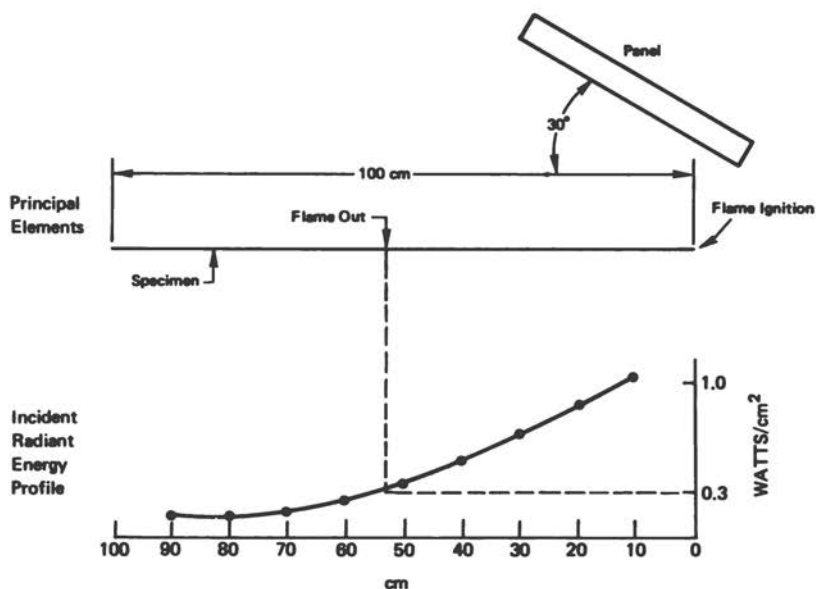
Figure 2. The flooring radiant panel test
