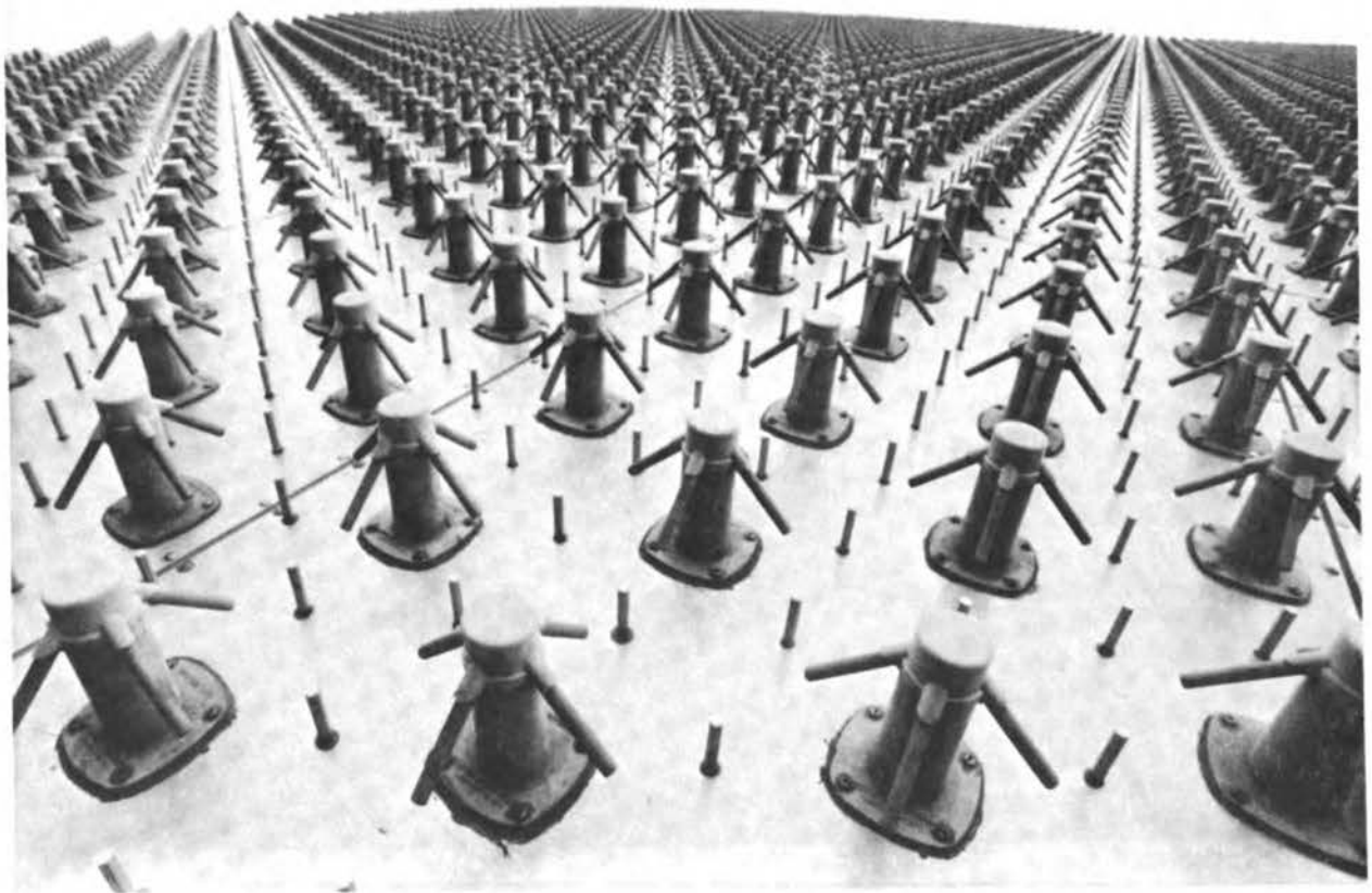
FIGURE 2. Regular array of antenna elements protruding from one face of PAVE PAWS radar.
