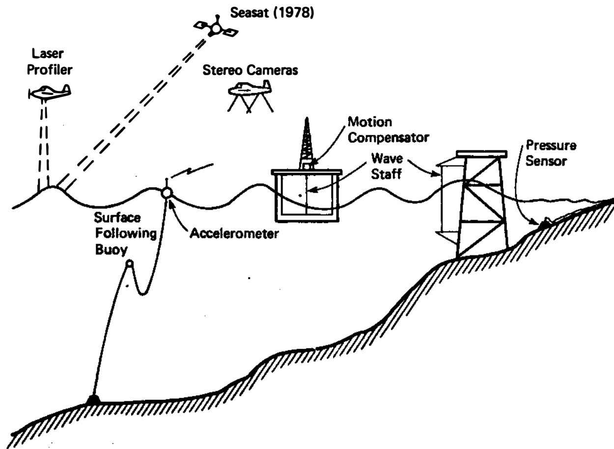
FIGURE 4 Wave Measurements
