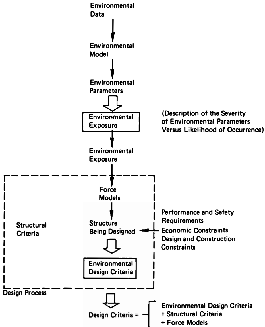
FIGURE 3 Schematic Illustration of Environmental Elements and Processes Used in Developing Design Criteria
