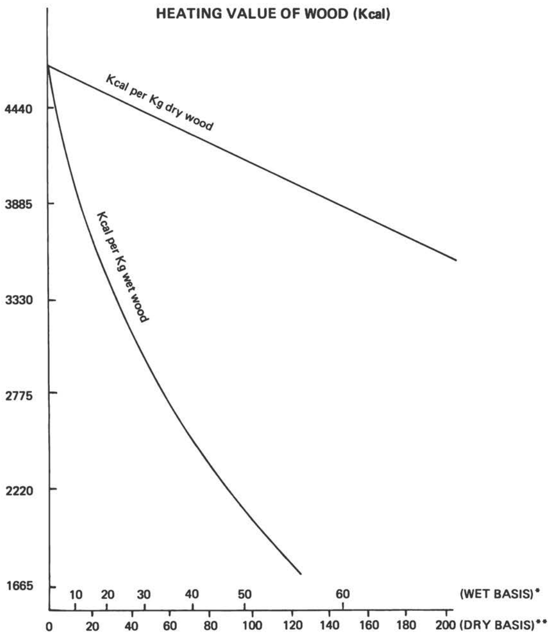
WOOD MOISTURE CONTENT (%) EFFECT OF WOOD MOISTURE CONTENT ON ITS HEATING VALUE
