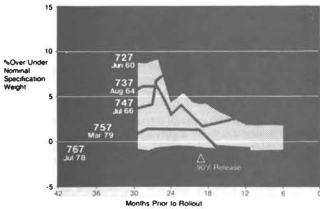
Figure 4.—Early weight information on the 767 allowed performance requirements to be met earlier than on previous programs.
