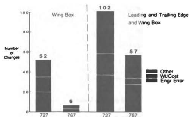
Figure 7.—Higher quality engineering and fewer changes late in the 767 program are attributed to CAD.
