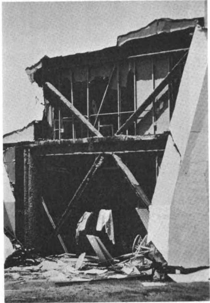
FIGURE 4.25 Closeup of damage to the facade of By-the-Sea Condominium.
