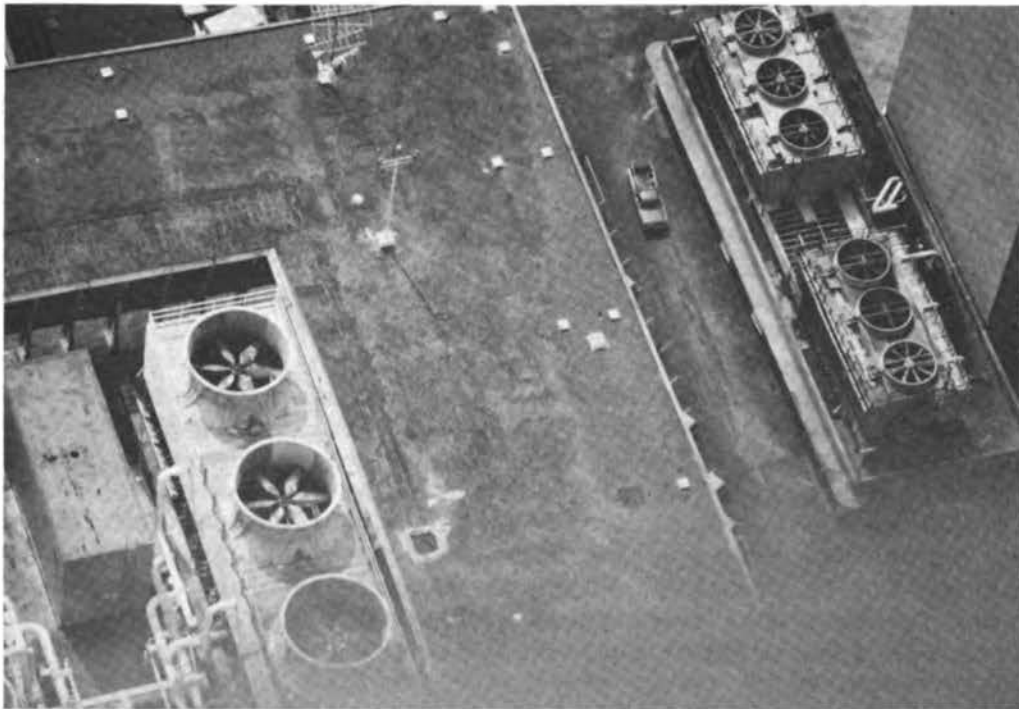
FIGURE 4.11 General view of the roof of the Tenneco Building.
