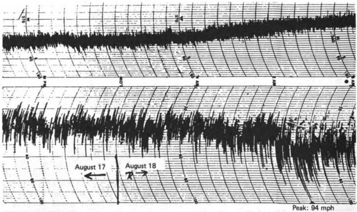
FIGURE 2.10D Anemometer record from Dow Chemical Plant B near Freeport illustrating wind regime in Hurricane Alicia near and following landfall.
