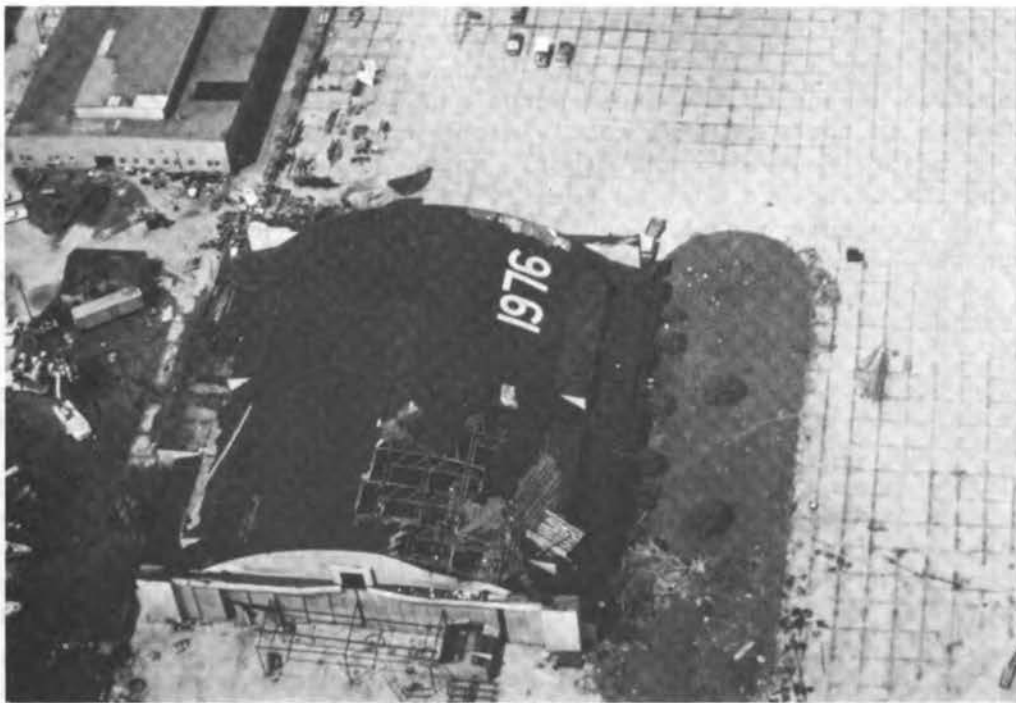
FIGURE 4.37 Wind damage to the roof of a hangar at Galveston Airport.
