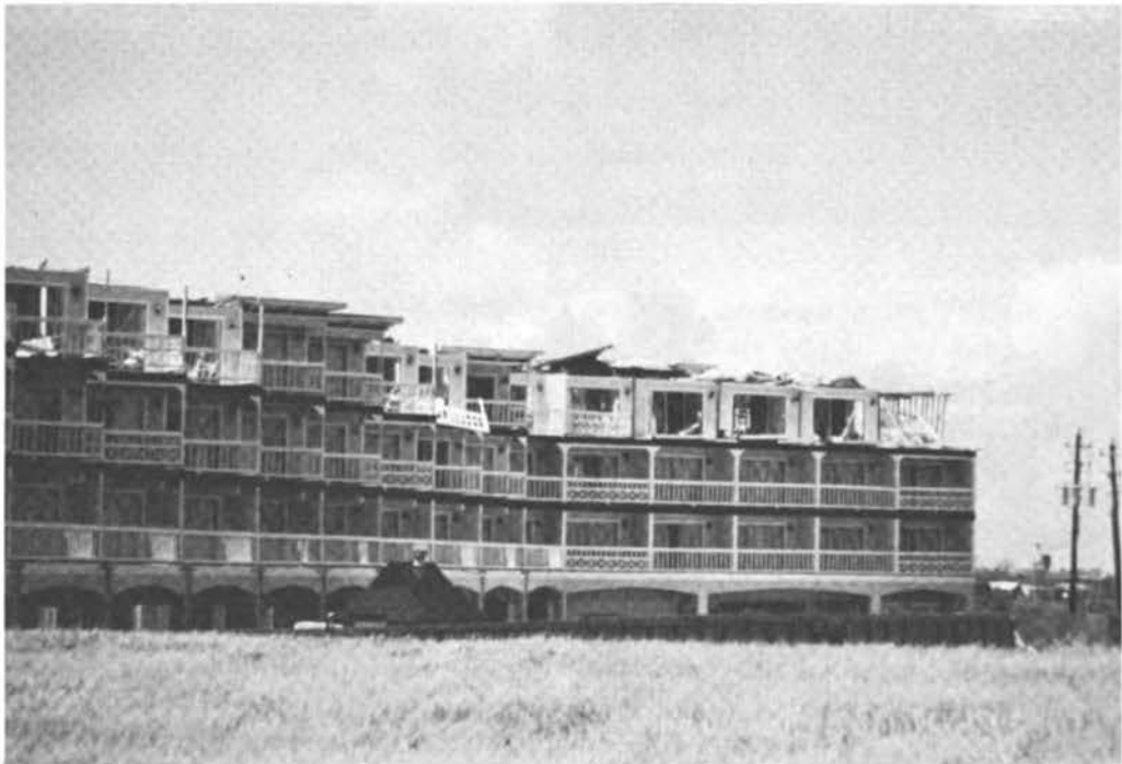
FIGURE 4.29 General view of the damaged wing of the Victoria Hotel.
