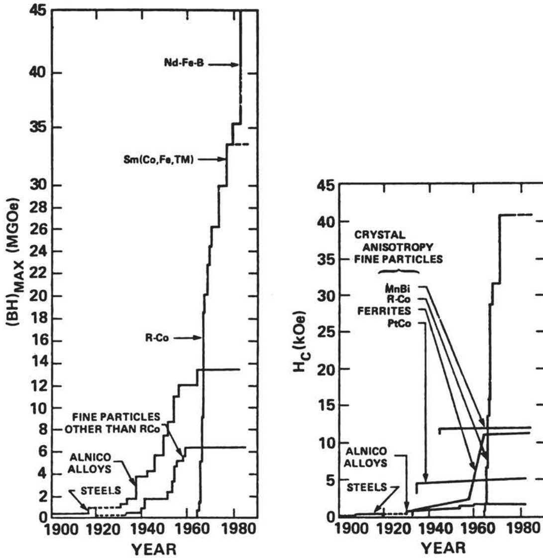
Figure 2 Energy product and coercivity of permanent magnets.
