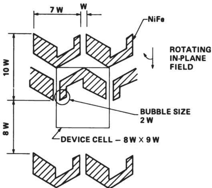
Figure 6 Bubble propagation structures showing device cell dimensions.
