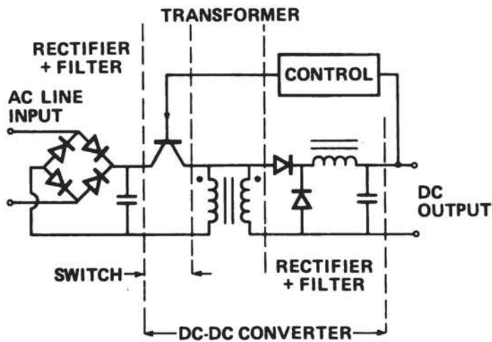
FIGURE 3 Simplified schematic diagram of typical off-line-switcher type power supply.
