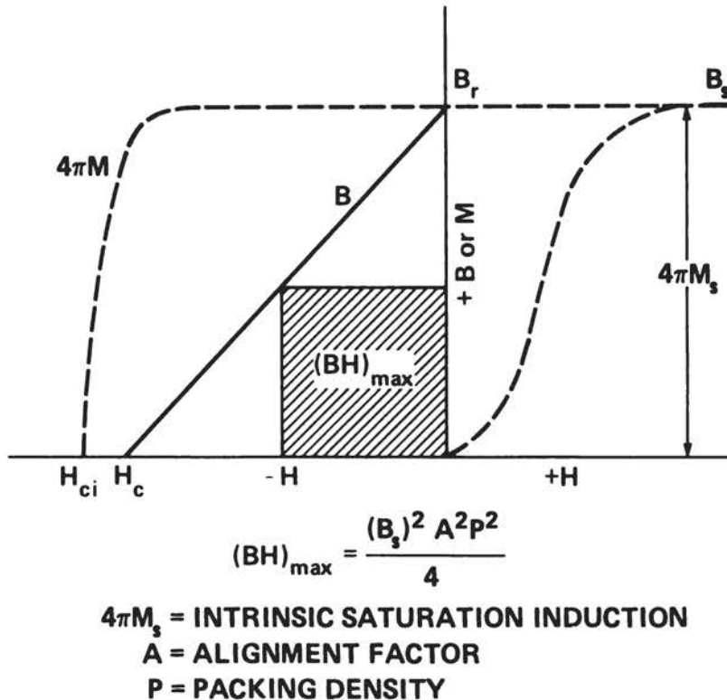
Figure 1 Hysteresis loop associated with a permanent magnet.
