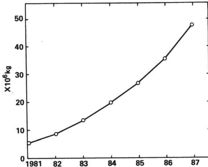
Figure 4 Consumption of magnetic particles in 1/2" video tape. Source: Magnetic Media Information Services Report MMIS, 1983.
