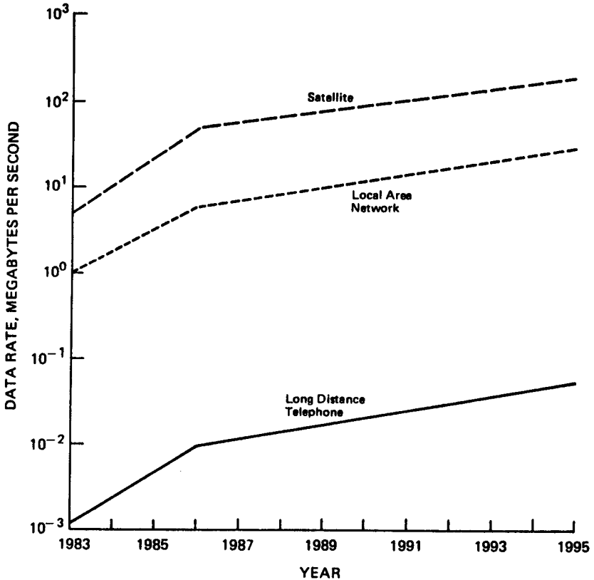
FIGURE 5.3 Projected growth in communications at constant cost.
