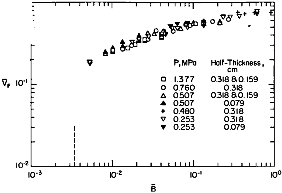
Dimensionless Spread Rates for Downward Spread over PMMA Samples [4].
