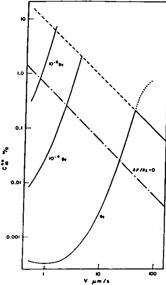
FIGURE 3.2. The critical concentration c_{\infty}^{**} of tin in lead above which instability occurs as a function of the velocity V of directional solidification for a temperature gradient G_L in the liquid of 200 K/cm. The solid curves represent gravitational accelerations g_e = 980 \text{ cm/s}^2 , 10^{-4} g_e , and 10^{-6} g_e . The upper line with negative slope represents the onset of morphological instabilities; the nearly parallel dashed-dot line labeled (\partial\rho/\partial z) = 0 represents the neutral density criterion. The dotted extension of the curve labeled g_e corresponds to oscillatory instabilities.
