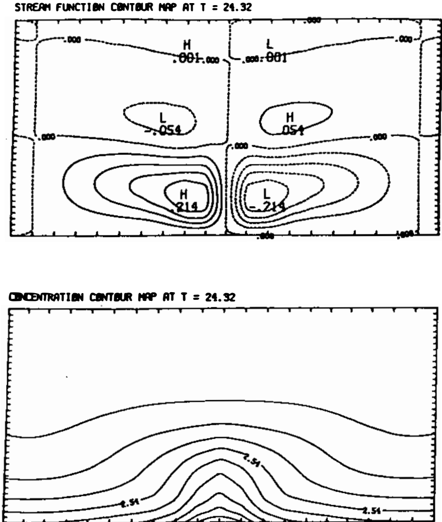
FIGURE 3.3. The steady-state stream function and concentration as a function of position for a bulk concentration 29 percent above the critical concentration for the onset of convection. Parameters used in the calculation are typical of semiconductor melts. In the concentration plot, the increment of (dimensionless) concentration between contours is 0.37. The maximum flow velocity is about 5 times the crystal growth velocity of typically 20 \mu\text{m/s} .
