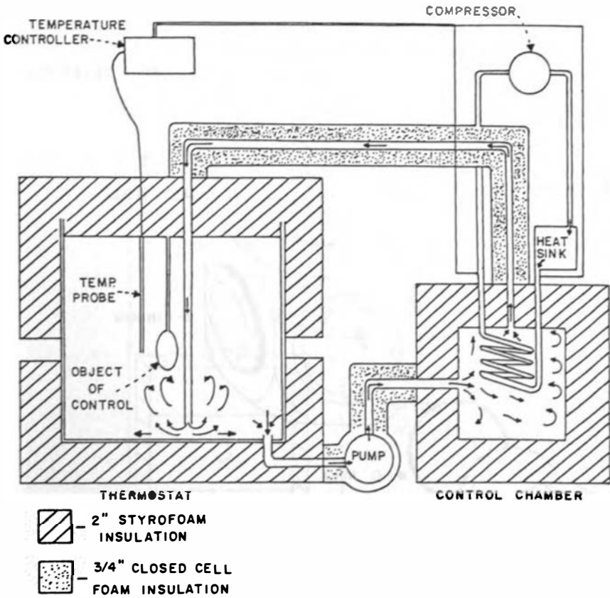
FIGURE 4.6. Schematic of thermostat for dendritic growth.
