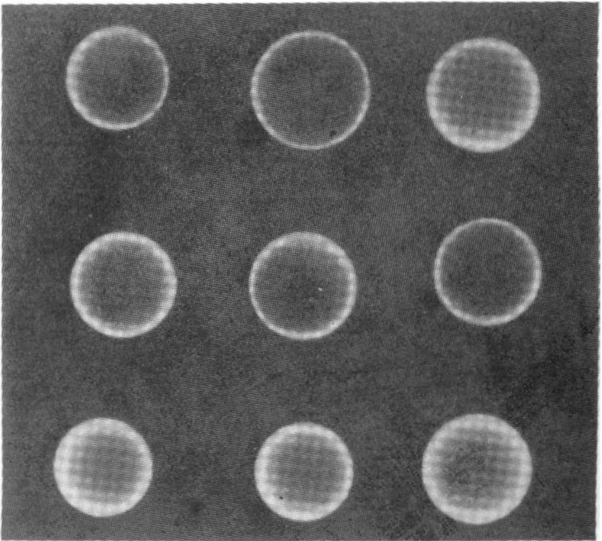
FIGURE 9.10. SEM photograph of AuPbSb amorphous shell. 1.5- \mu\text{m} diameter.
