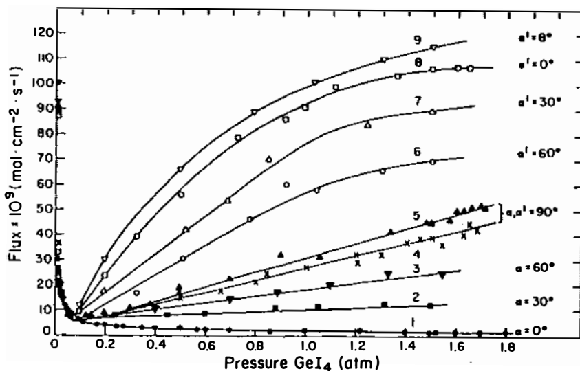
FIGURE 7.7. Mass transport rates of the GeSe-GeI 4 system as a function of ampoule inclination with respect to the gravity vector. Angle \alpha denotes inclination with hot zone above (curves 1-3; curve 1 vertical, stabilizing) and \alpha' denotes inclinations with hot zone below (curves 6-9; curve 8 vertical, destabilizing). Curves 4 and 5 ( \alpha = \alpha' = 90^\circ ) horizontal orientation of ampoule with and without indentations near hot end of ampoule, respectively. Values on the abscissa are initial pressures of GeI 4 . 10
