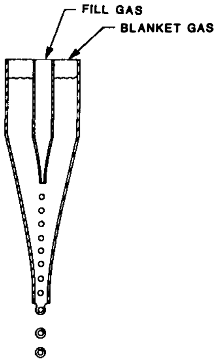
FIGURE 9.5. Nozzle configuration for production of small shells.
