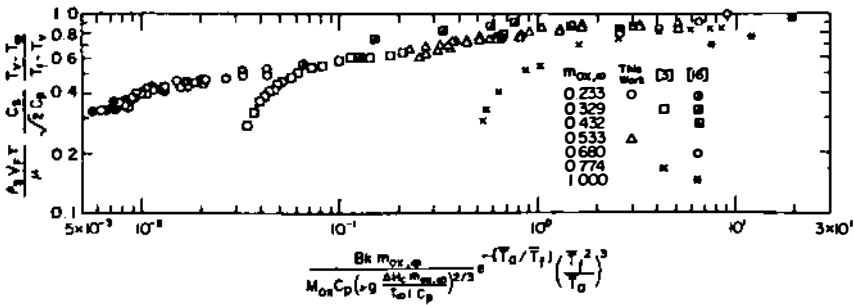
Dimensionless Spread Rates for Downward Spread over Paper Samples [3].
