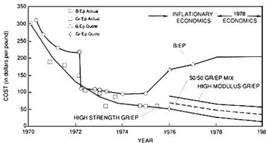
Figure B-2 Material properties and history assessment.
