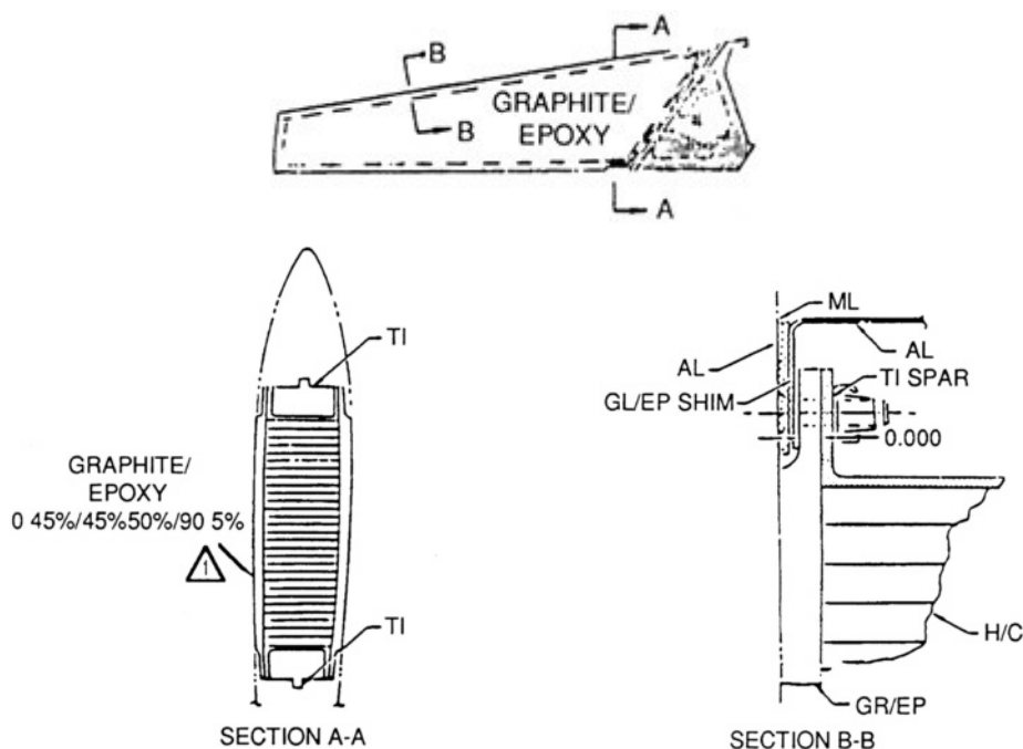
Figure B-3 Torque box assembly method.
