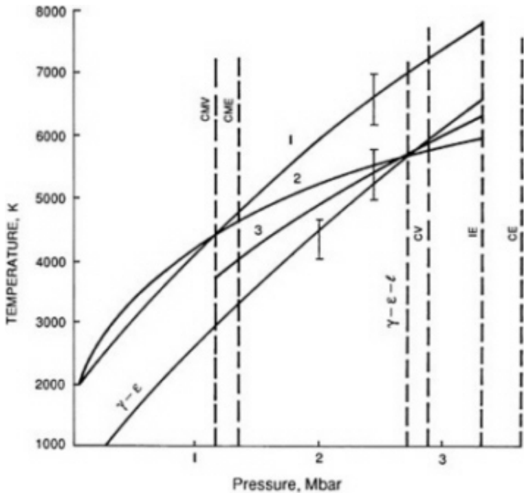
FIGURE 3 Pure iron melting curves according to various data and the boundary of the phase transition \gamma\text{—Fe—}\epsilon\text{—Fe} . The figures indicate melting curves: 1 is from the study by Williams et al. (1987); 2 is from the study by Anderson (1986) and experimental data from Brown and McQueen (1986); and 3 is based on the Lindeman formula with the Grunchaissen parameter of G = 1.45 = \text{const} , using experimental data from Brown and McQueen (1986). The transition boundary, \gamma\text{—}\epsilon , was constructed in the study by Anderson (1986) and together with the melting curve gives us the location of the triple point. The vertical segments illustrate errors in determining temperature for curves 1 and 2. The boundary labels are as follows: CM is the boundary between the core and the mantle; C denotes the center of the planet; I is the boundary of the solid inner core; and the final letter indicates Earth (E) or Venus (V). \gamma - \epsilon - I denotes the location of the triple point.
