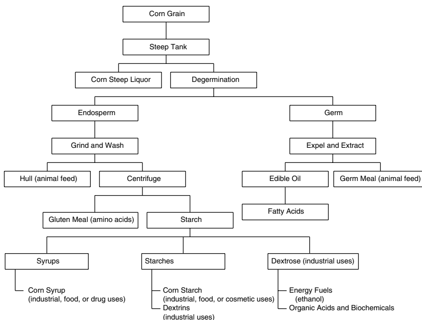
FIGURE 4-1 Corn processing and fermentation chemicals.
