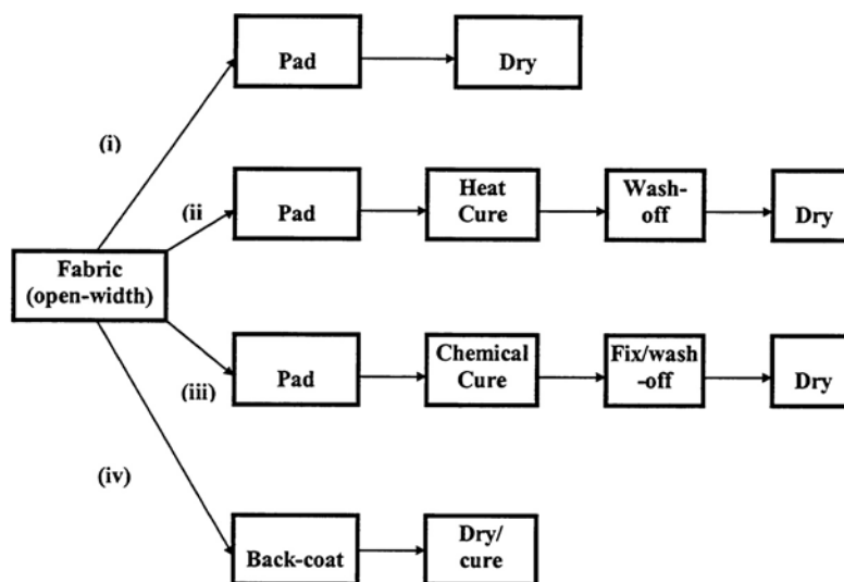
FIGURE B-1 Schematic representation of the most common methods of application of flame retardants to textile fabrics.
