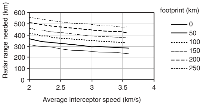
FIGURE 3.1 Trade-offs between radar range and interceptor velocity in a terminal-phase engagement.
