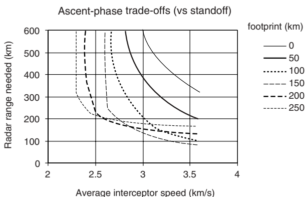
FIGURE 3.2 Trade-offs between radar range and interceptor velocity in an ascent-phase engagement.
