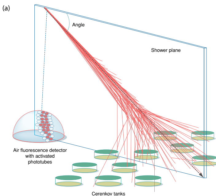
FIGURE 6.1.1 (a) Illustration of a ground-based array of Cerenkov water detectors for detecting shower particles with a fluorescence detector for imaging the atmospheric cascade generated by ultra-high-energy cosmic rays. (b) An array of phototubes suspended in ice that senses interactions of upward-going neutrinos; it uses the bulk of the Earth to filter out other types of particles; adapted from image courtesy of the IceCube Collaboration. (c) One of the Cerenkov shower detectors in the Pierre Auger Observatory array in Argentina; image courtesy of the Pierre Auger Observatory.
