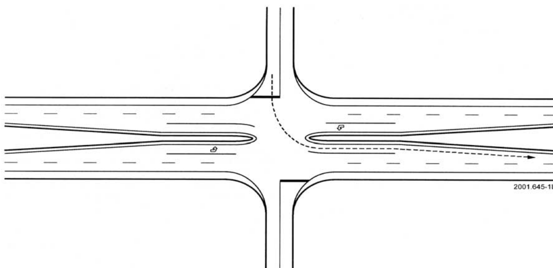
Figure 6. Typical divided highway intersection with median acceleration lanes (7).
