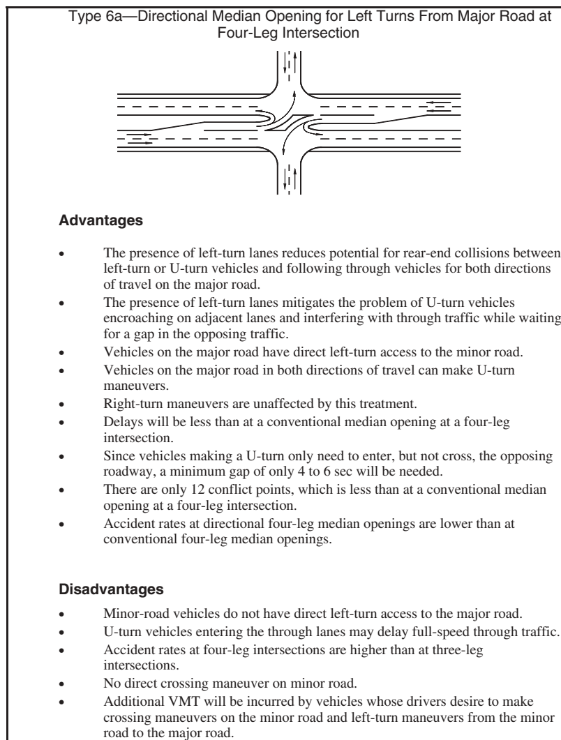
Figure C-17. Advantages and disadvantages of median opening type 6a—directional median opening for left turns from major road at four-leg intersection.
