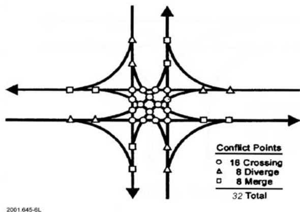
Figure 37. Vehicular conflicts at a conventional median opening at a four-leg intersection (27, 33).
