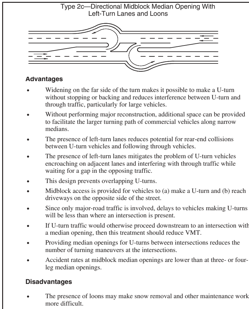
Figure C-8. Advantages and disadvantages of median opening Type 2c—directional midblock median opening with left-turn lanes and loons.
