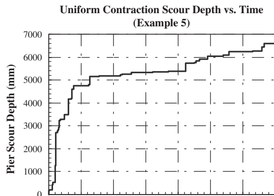
Figure 12.26. Uniform contraction scour depth versus time (Example 5).
