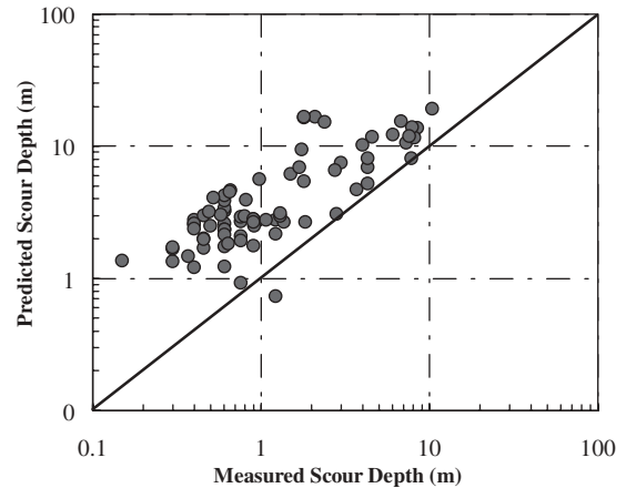
Figure 10.6. HEC-18 predictions against Froehlich (1988) Database.
