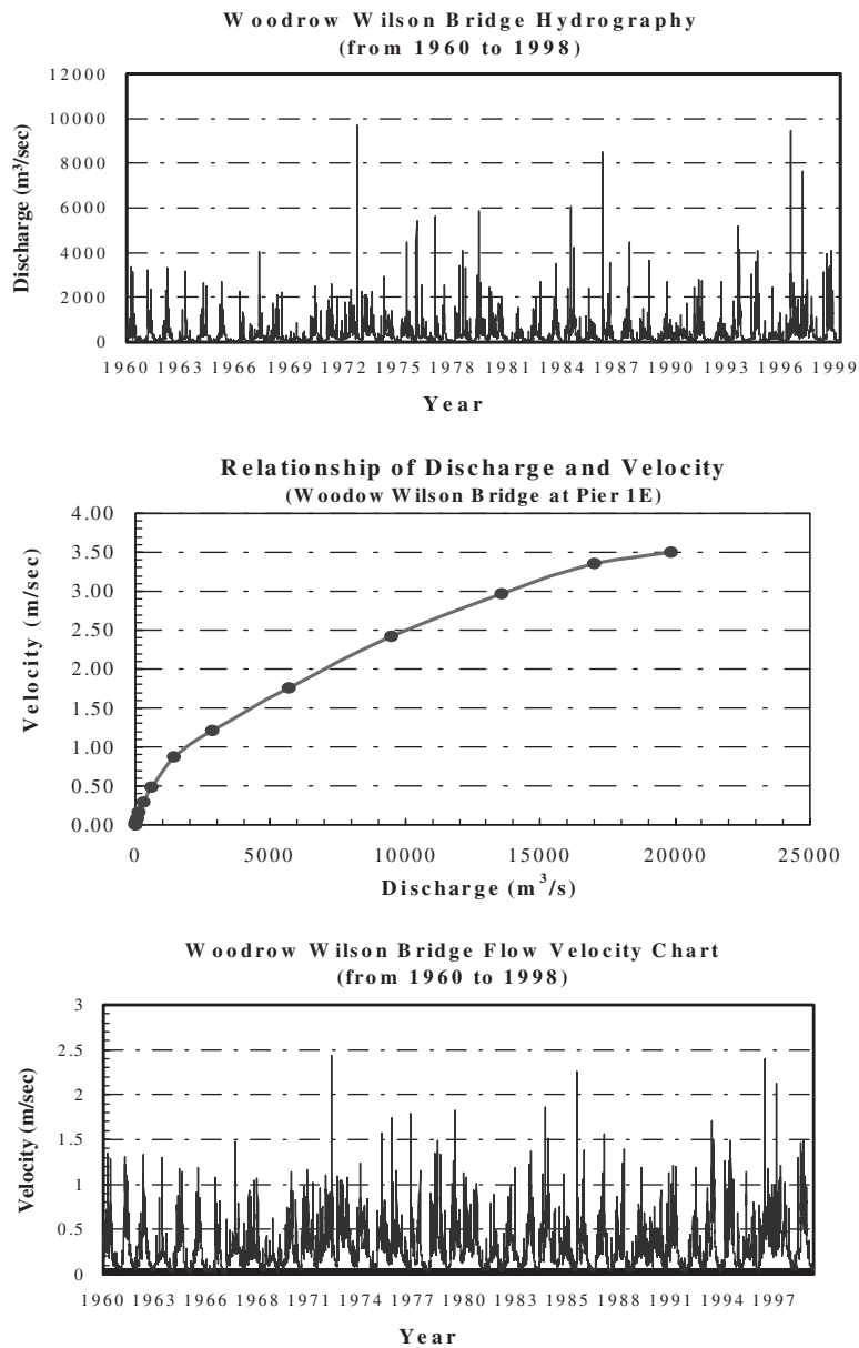
Figure 9.8. Example of hydrograph transformation for Pier 1E of the Woodrow Wilson Bridge on the Potomac River in Washington, D.C.
