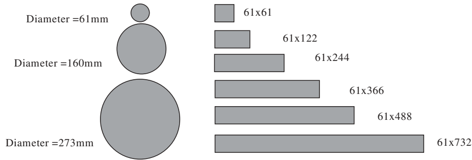
Figure 5.3. Pier models used in the complex pier scour tests.
