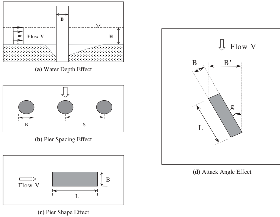
Figure 5.1. Parameter definition for complex pier scour.
