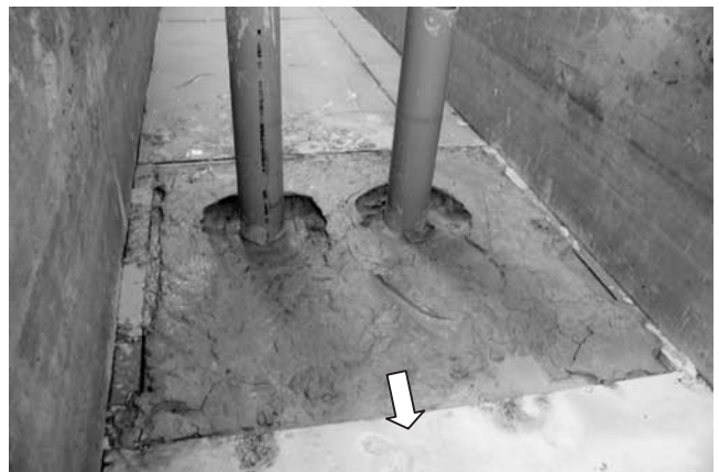
Figure A6 Scour Hole of Test Gr-2.
