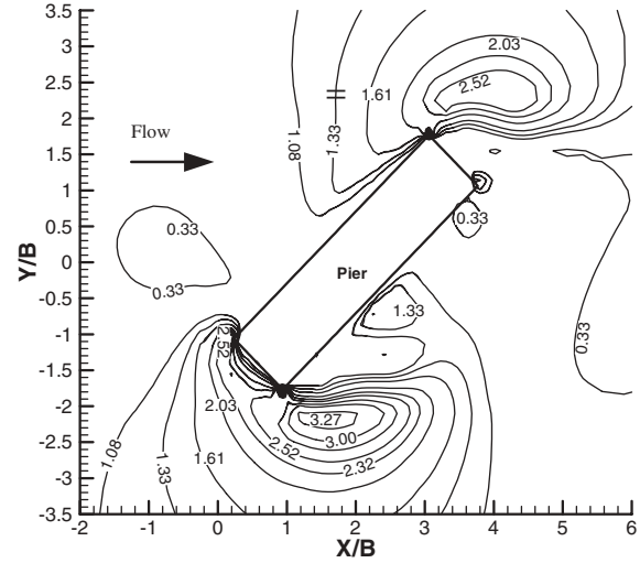
Figure 6.25. Bed shear stress ( \text{N/m}^2 ) contours for an attack angle equal to 45 degrees.
