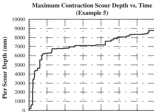
Figure 12.25. Maximum contraction scour depth versus time (Example 5).
