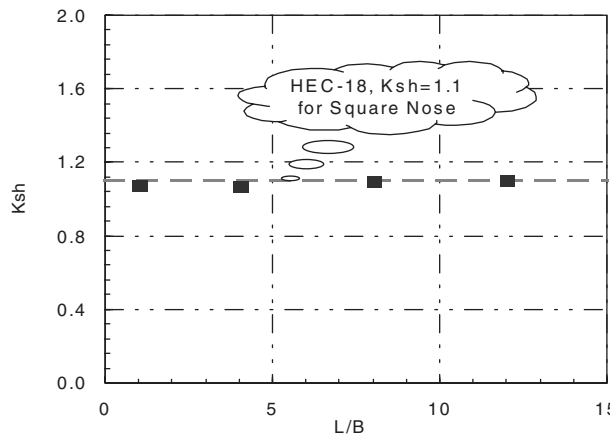
Figure 5.19. Correction factor for pier shape effect.
