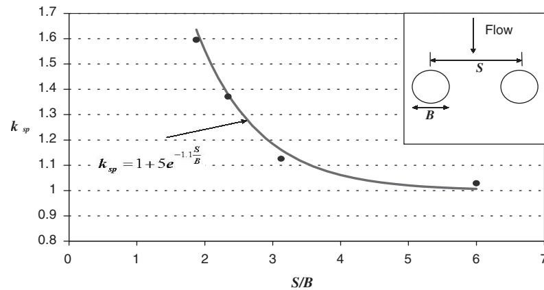
Figure 6.14. Relationship between k_{sp} ( = \tau_{max}/\tau_{max(single)} ) and S/B for deep water H/B > 2 ).
