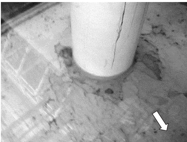
Figure A3 Pier Scour Hole under Shallow Water Condition—Back View.
