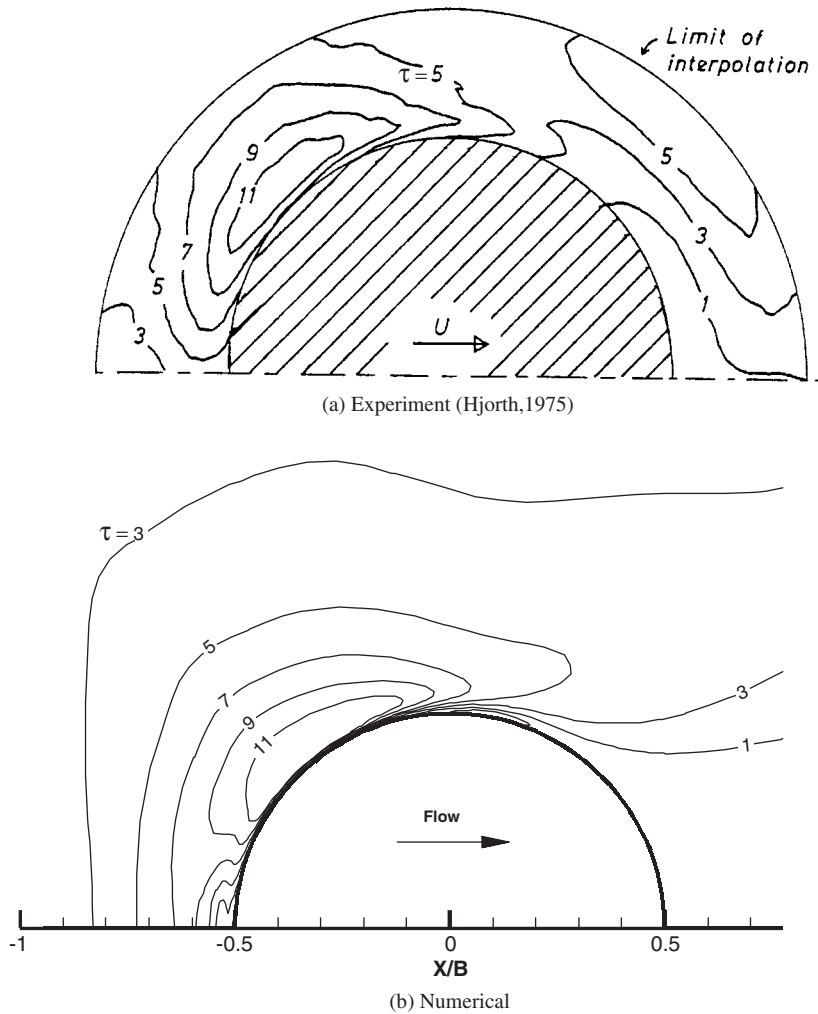
Figure 6.2. Comparison of bed shear stress distribution ( N/m^2 ) around a circular pier as calculated from an experiment by Hjorth (1975) and numerical computations ( B = 0.075 m, V = 0.30 m/s, H = 0.2 m).
