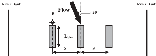
Figure 12.13. Plan view of rectangular piers group scour case (Example 3).
