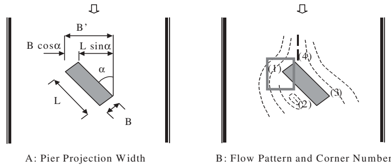
Figure 5.24. Skewed pier definitions.
