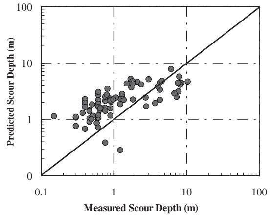
Figure 10.5. SRICOS-EFA predictions against Froehlich (1988) Database.
