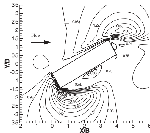
Figure 6.24. Bed shear stress ( N/m^2 ) contours for an attack angle equal to 30 degrees.
