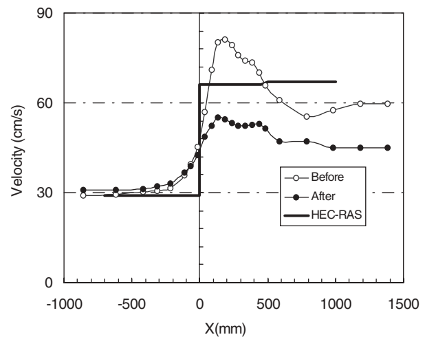
Figure 7.3. Velocity distribution along the channel centerline in Test 2.
