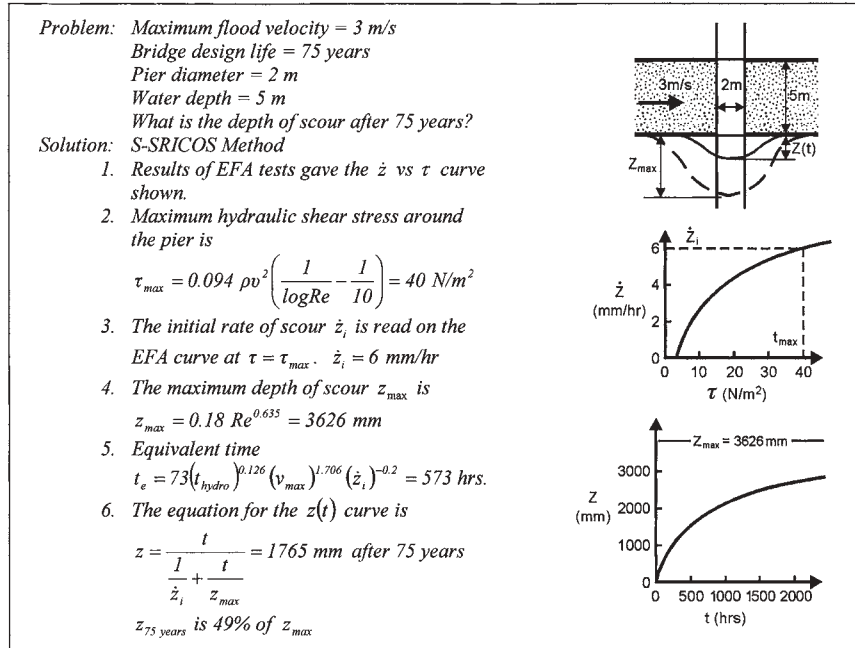
Figure 4.13. Example of scour calculations by the S-SRICOS Method.
