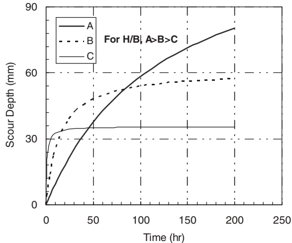
Figure 5.13. Comparison between scour in shallow and deep waters.
