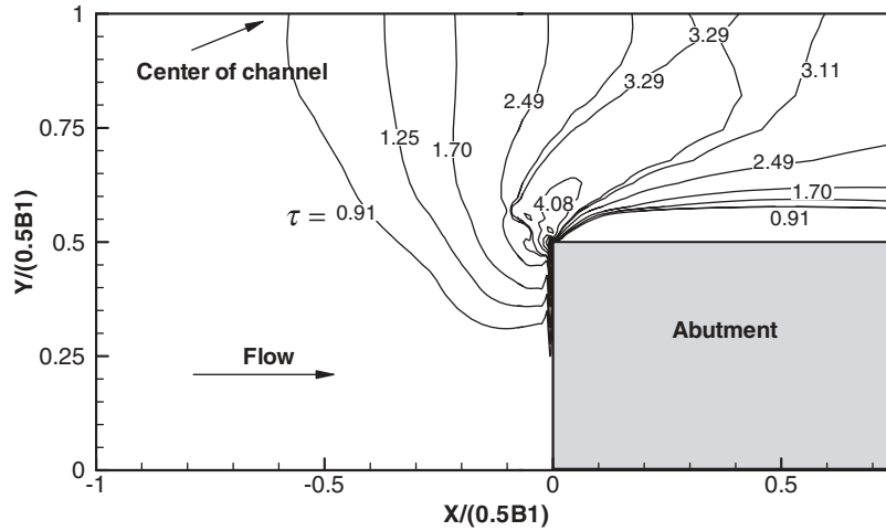
Figure 8.3. Initial bed shear stress distribution ( N/m^2 ) for B_1/B_2 = 0.50 and V = 0.45 m/s .
