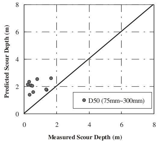
Figure 10.3. SRICOS-EFA predictions versus Mueller Database for various ranges of D_{50} .
