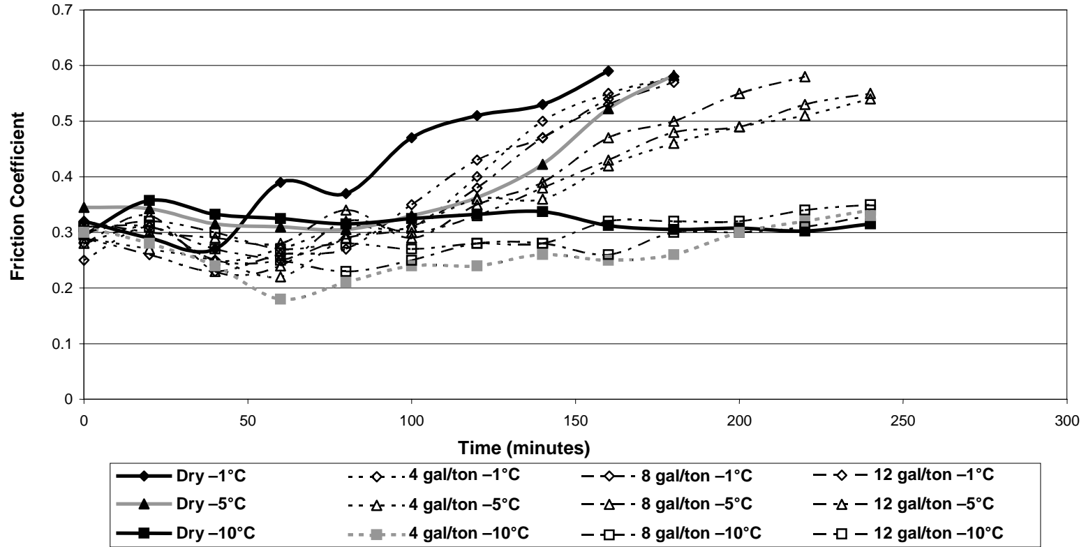
FIGURE 2 Water pretwet BRS and dry BRS friction versus time.
