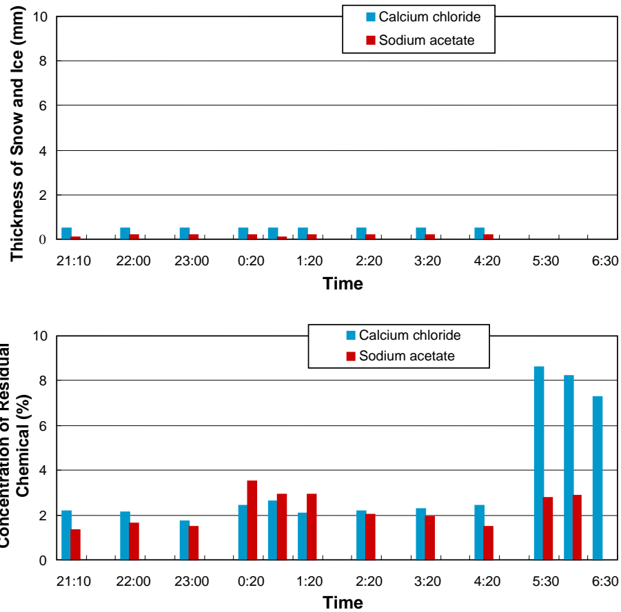
FIGURE 9 Change of the thickness of the snow and ice on the road surface and concentration of the residual chemical on the road surface.
