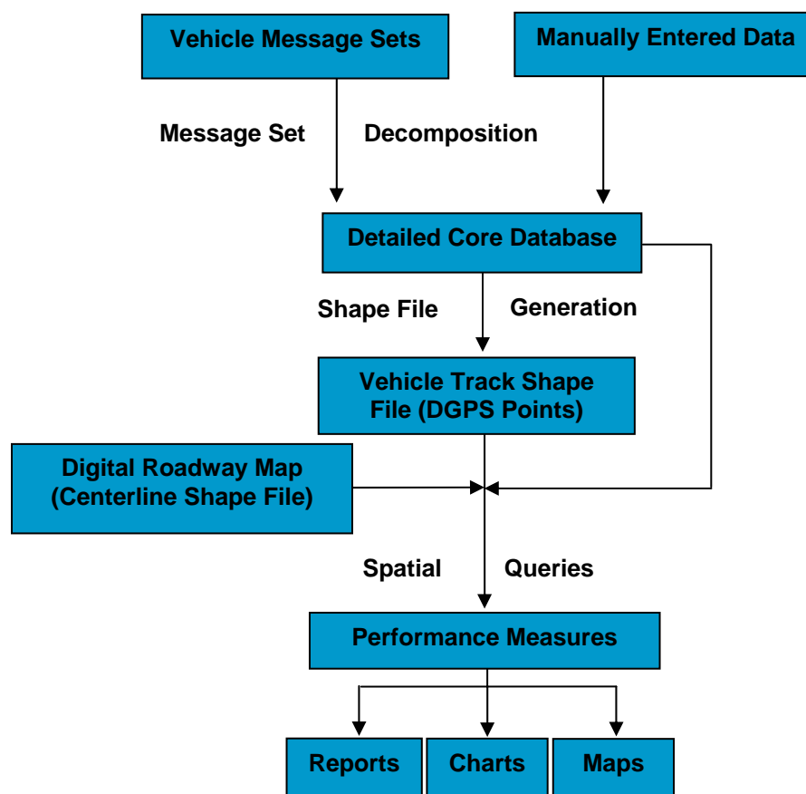
FIGURE 2 Wisplow data and program flow.
