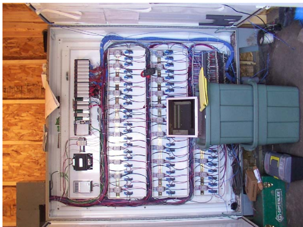
FIGURE 12 Microprocessor-based controller system.
