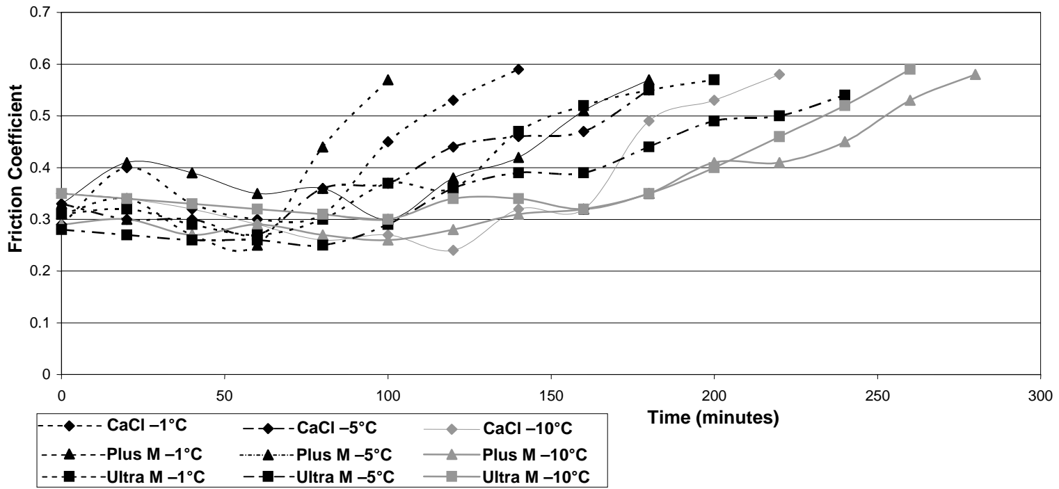
FIGURE 4 Eight gal/ton liquid chemical prewetted BRS friction versus time.
