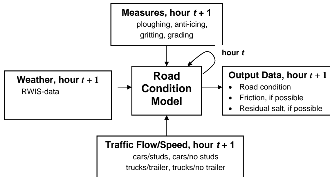
FIGURE 2 Input and output data to and from the road condition model.
