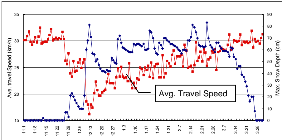
FIGURE 10 Average travel speed and maximum snow depth.
