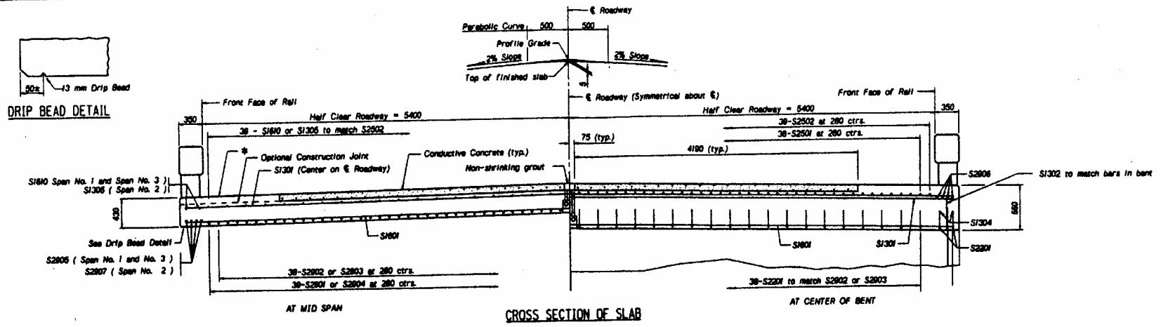
FIGURE 4 Cross section of slab.
