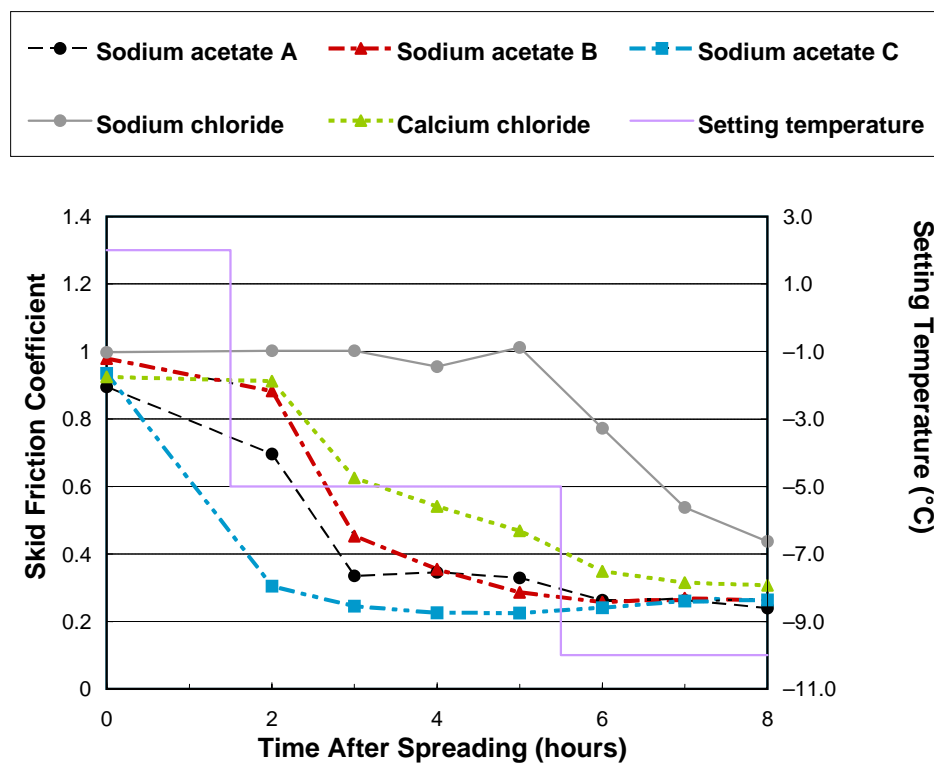
FIGURE 5 Results of measurement of skid friction coefficient in the laboratory.
