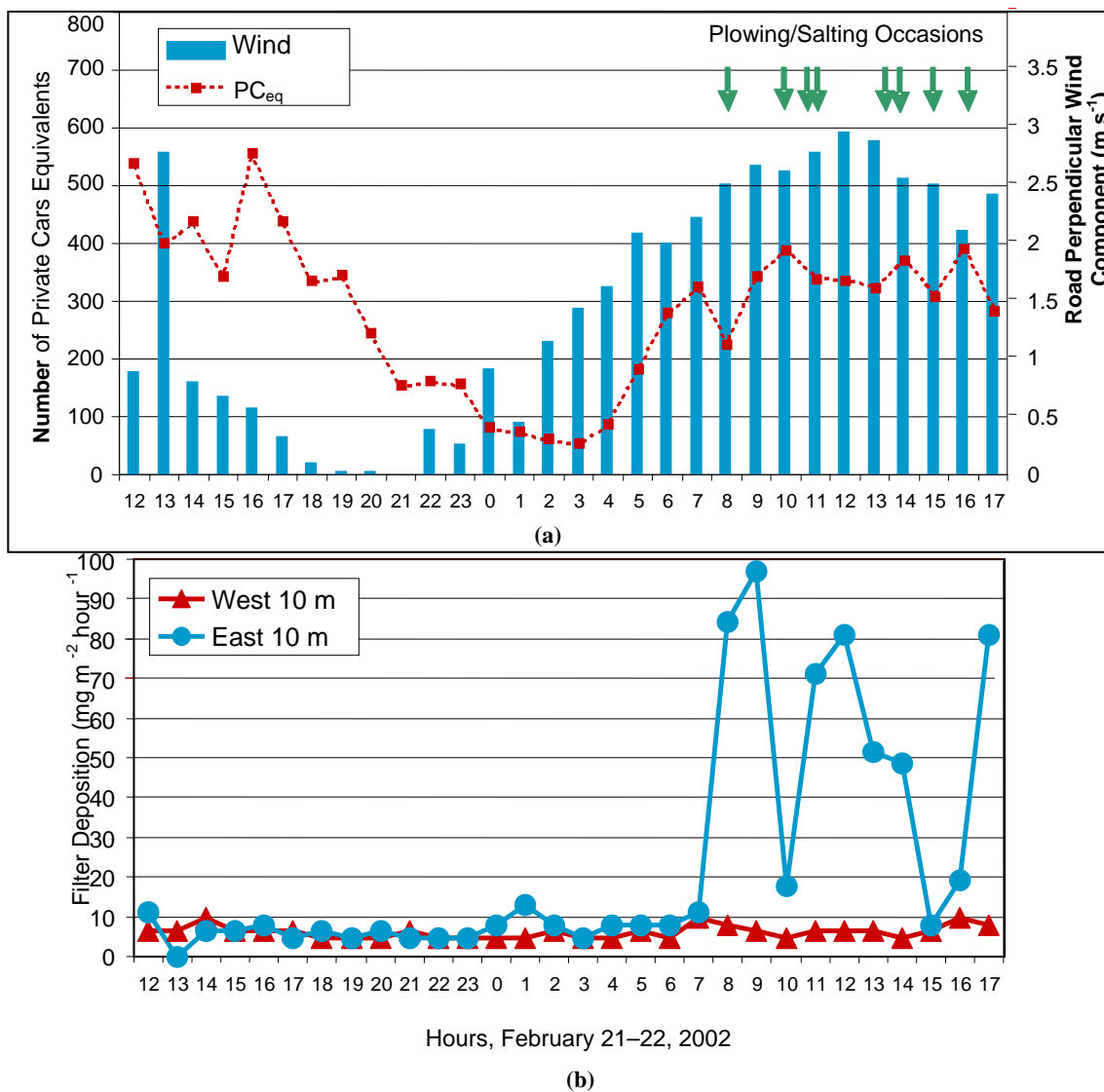
FIGURE 4 Field data from Vimmerby field site: (a) wind and traffic characteristics during the investigation period (the plowing and salting passages are marked by arrows, pointing out their occasions in time) and (b) the amount of chloride deposited on the salt vane filters on each side of the road.
