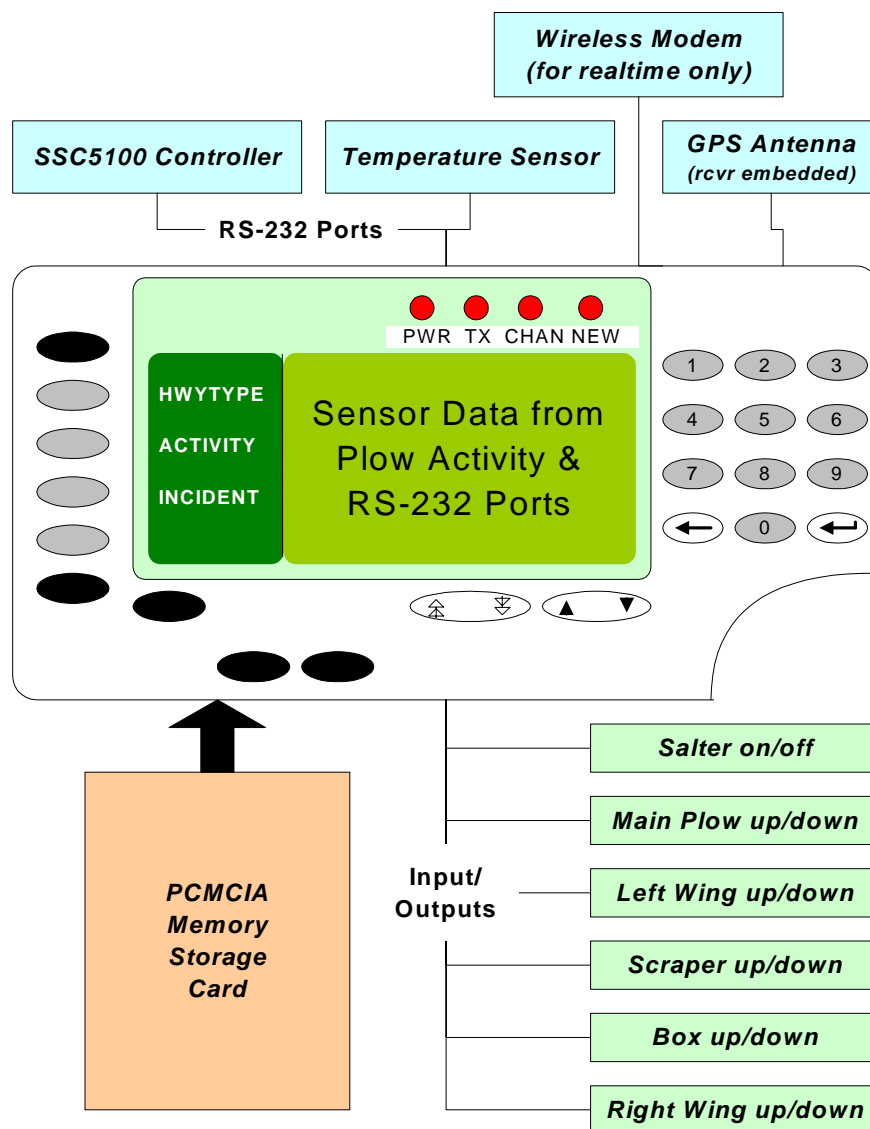
FIGURE 3 MDC block diagram with sensor connections.
