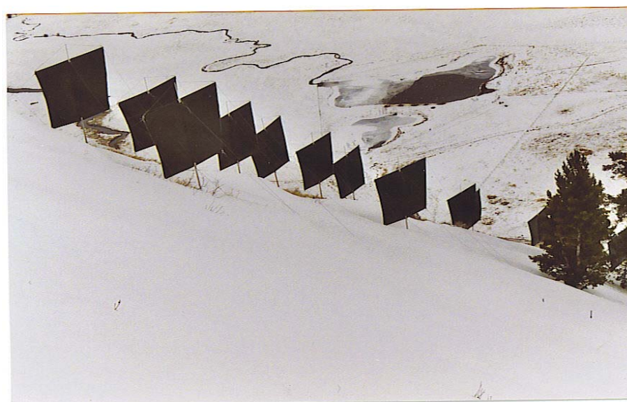
FIGURE 7 A view of a portion of the full snow-sail deployment of the 151 avalanche.
