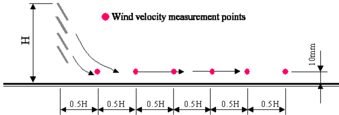
FIGURE 3 Blower snow fence and wind velocity measurement points.
