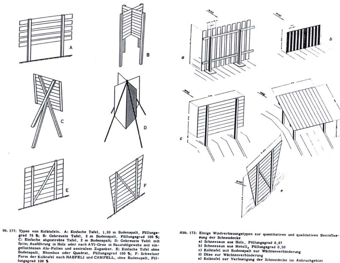
FIGURE 1 A schematic depiction of European kolktafeln circa 1960 (1).
