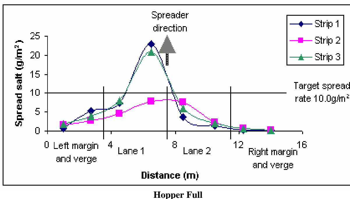
FIGURE 6 Example of symmetric dry salt spreading.
