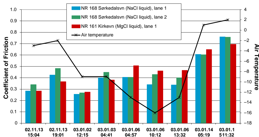
FIGURE 12 Results from friction measurements. (Testing MgCl_2 liquid as a prewetting agent to dry NaCl , the 2002–2003 winter season. )
