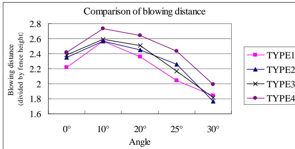
FIGURE 8 Comparison of blowing distance by interval and height of wind-straightening vane.
