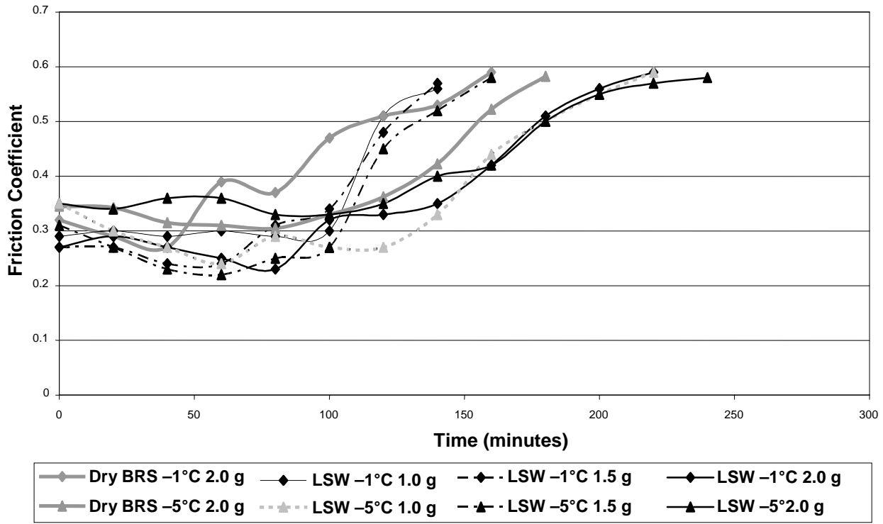
FIGURE 5 Caliber M2000 LSW friction versus time at -1^{\circ}\text{C} and -5^{\circ}\text{C} .
