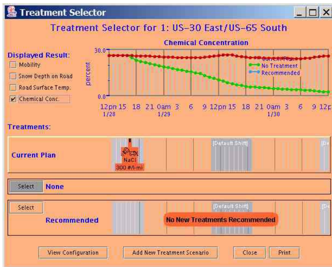
FIGURE 6 MDSS treatment selector screen. The red trace (top line, top window) shows the predicted chemical concentration if the treatment application is followed. The green trace (bottom line) shows the chemical dilution rate if no chemicals were applied.
