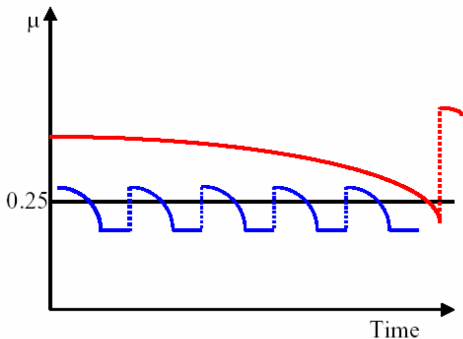
FIGURE 13 Diagram friction–time.
