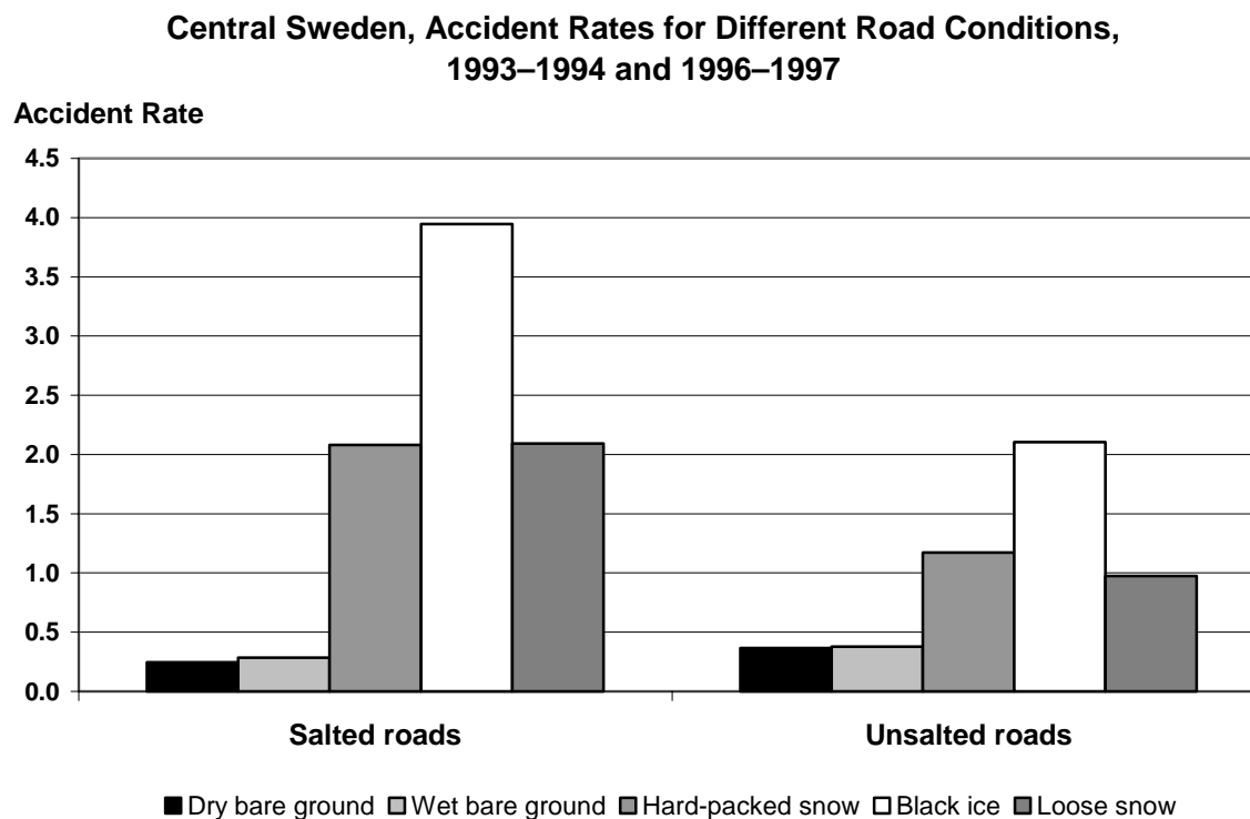
FIGURE 3 Average accident rates (accidents per million vehicle kilometers) for different road conditions, salted and unsalted roads.
