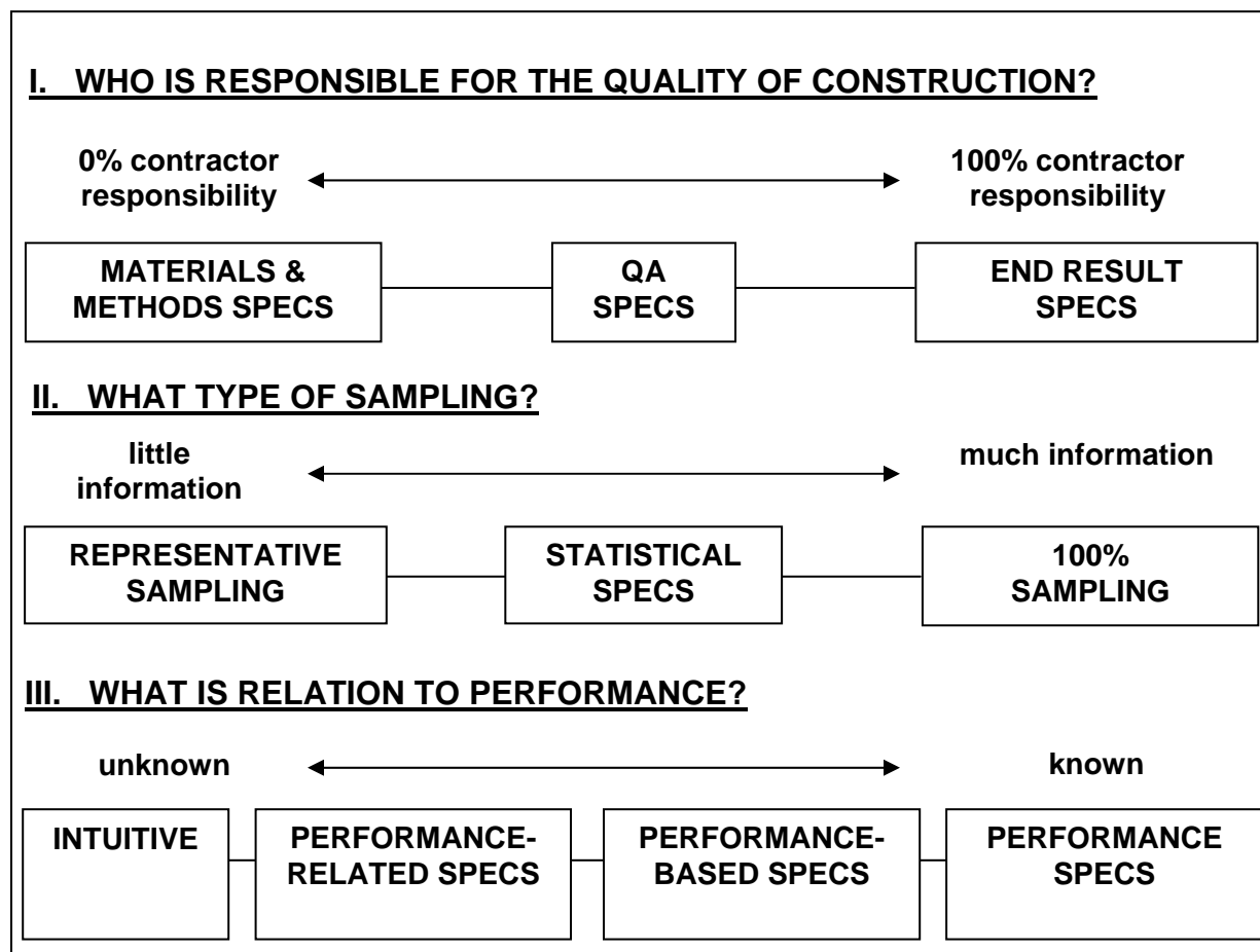
FIGURE 2 Classifying highway construction specifications (40). Highway construction specifications may be classified according to (I) who is responsible for the quality of construction, (II) the type of sampling employed, and (III) the relationship between quality criteria and constructed product performance. Thus, a QA specification according to classification I, for example, might be a statistical specification for classification II, and contain intuitive specification limits and pay adjustments for classification III. A specification might also, and usually does, contain one or more features within the same classification. For example, a specification that is primarily performance-related might contain some performance-based acceptance criteria and some intuitively developed acceptance criteria.
