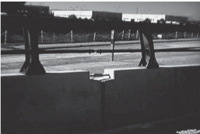
Figure 6. New Jersey border bridge used in Italy.
