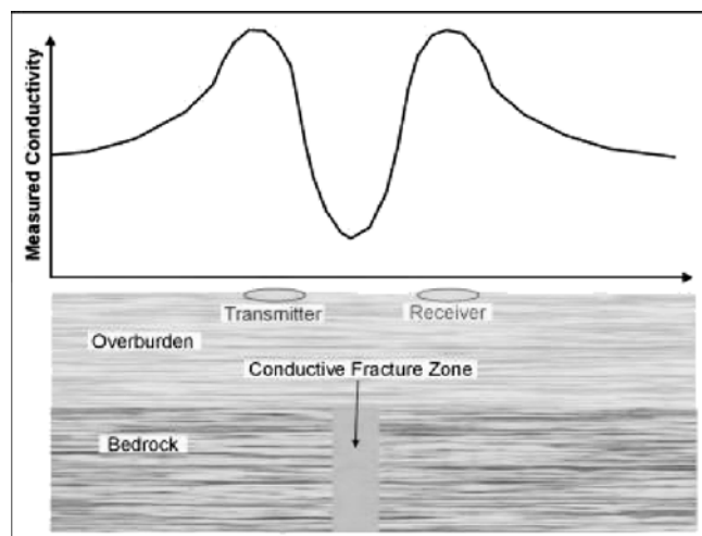
FIGURE A17 Example of the measured conductivity over a vertical conductive feature when taking readings in the vertical dipole mode.
