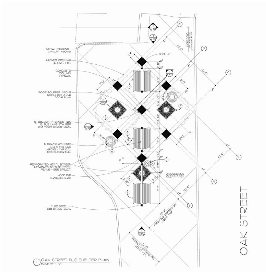
FIGURE 12 Floor plan of Gilbert park-and-ride passenger shelter.
