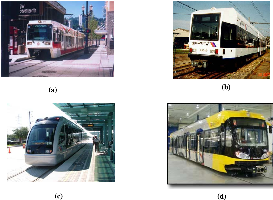
FIGURE 1 U.S. low-floor vehicle designs: (a) traditional design 70% low-floor, Portland; (b) first crashworthiness design, Hudson–Bergen; (c) newer design, Houston; and (d) newer design, Hiawatha.
