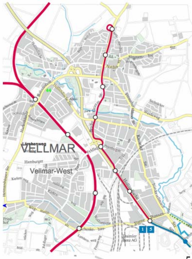
New RegioTram stations on existing railway.
