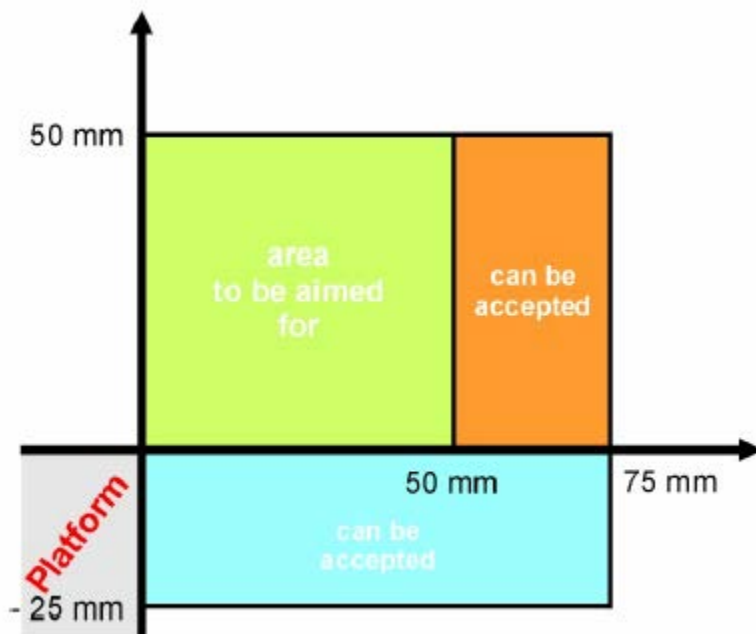
FIGURE 4 Boarding and alighting vertical step and horizontal gap recommendation.
