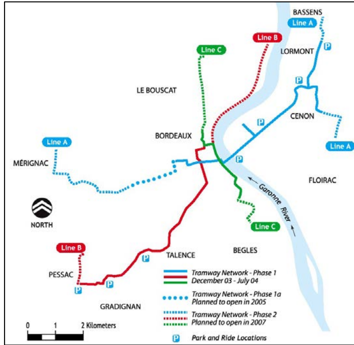
FIGURE 1 Bordeaux LRT system, France.
