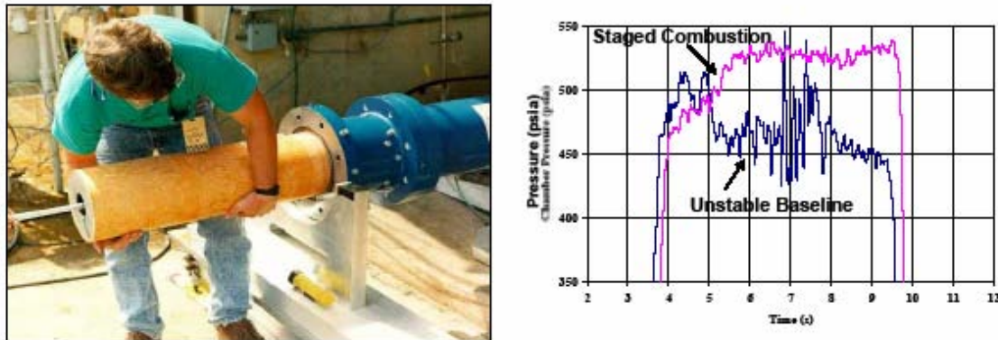
FIGURE 5-12 Staged combustion approach provided stable combustion and increased performance in the 11-in. diameter hybrid motors. SOURCE: Lockheed Martin Space Systems Company.
