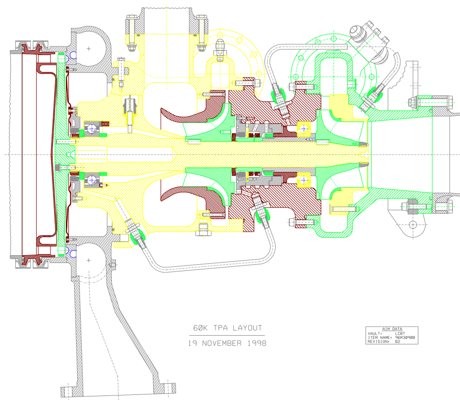
FIGURE 4-22 MC-1 Barber Nichols TPA. SOURCE: NASA, MSFC.
