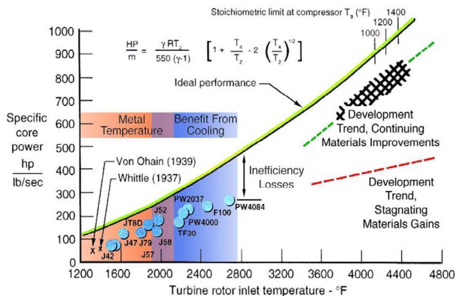
FIGURE 6-4 Materials and core engine performance. SOURCE: Hardwick (2005).
