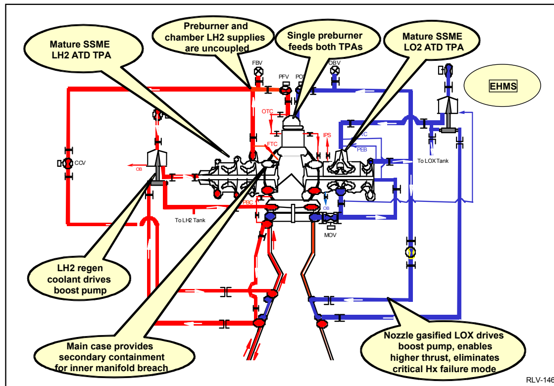
FIGURE 4-17 COBRA engine schematic. SOURCE: Pratt &amp; Whitney.
