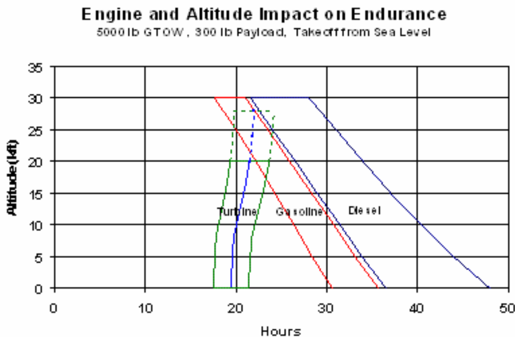
FIGURE 3-12 Impact of engine and altitude on endurance. SOURCE: DARPA (Undated).
