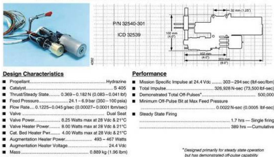
FIGURE 5-3 Aerojet MR-501B electrothermal hydrazine thruster (EHT). SOURCE: Aerojet (2004b).
