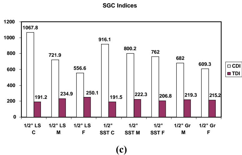
FIGURE 1 Compaction parameters of asphalt mixtures.
