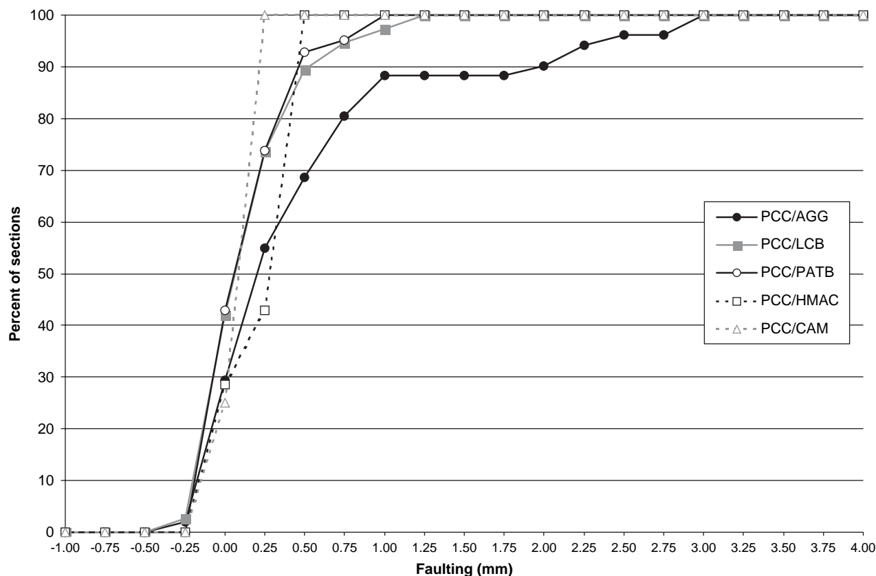
Figure 108. Cumulative frequency distributions of faulting for SPS-2 pavement sections.
