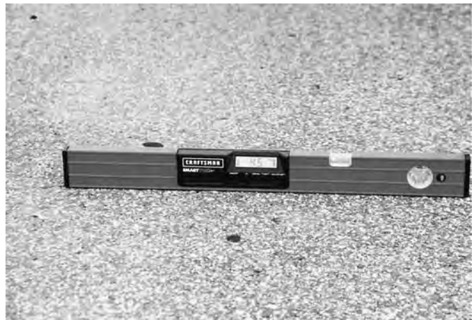
Figure 52. Digital level for measuring transverse and longitudinal grades.
