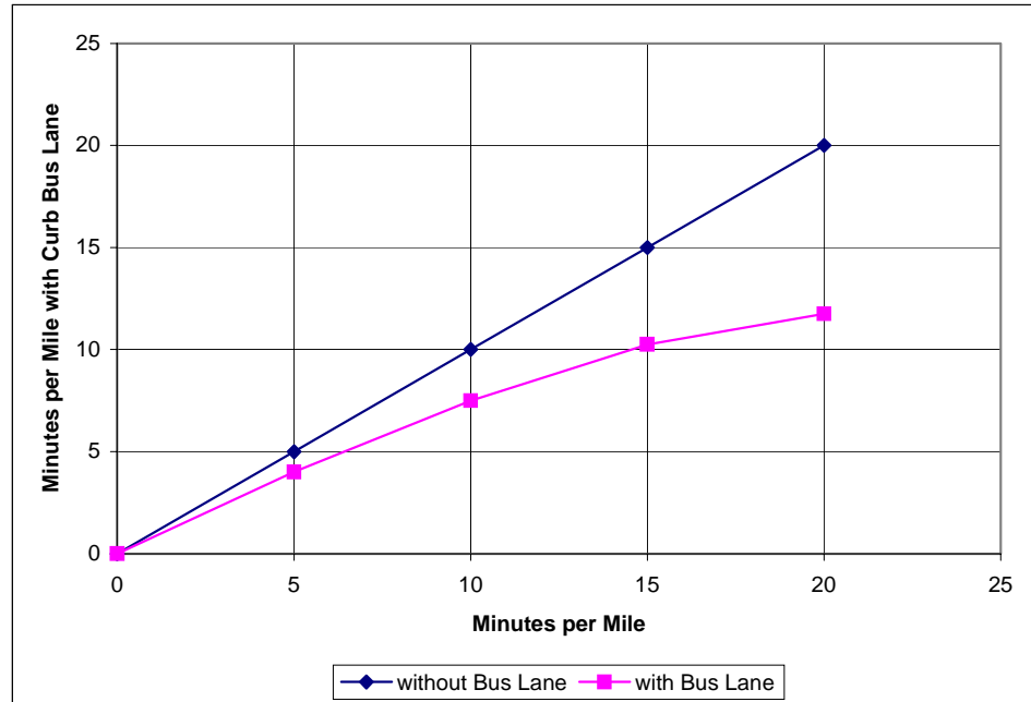
EXHIBIT 4-32 Time Savings with Curb Bus Lane
