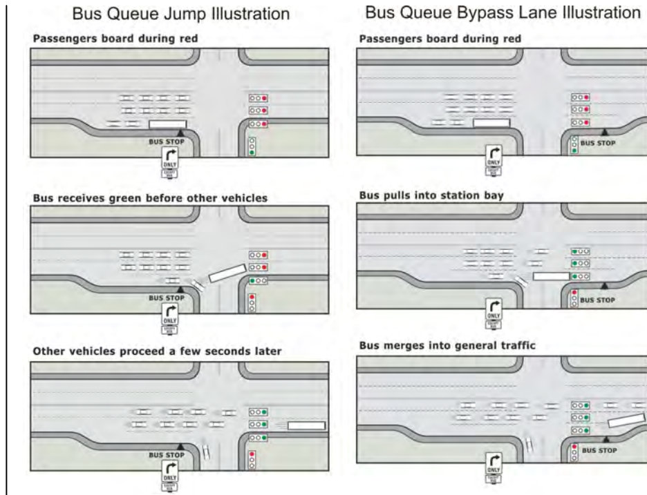
EXHIBIT 4-47 Queue Jump and Bypass Lane Operation
