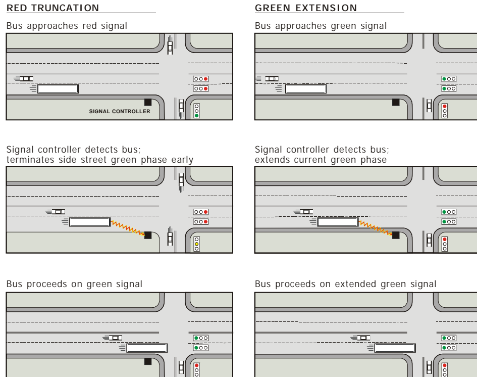
SOURCE: Transit Capacity and Quality of Service Manual (9) EXHIBIT 4-35 TSP Green Extension/Red Truncation Concept
