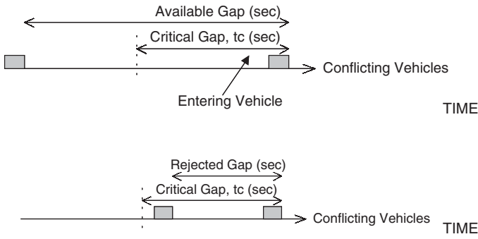
Figure 16. Concept of accepted and rejected gap.
