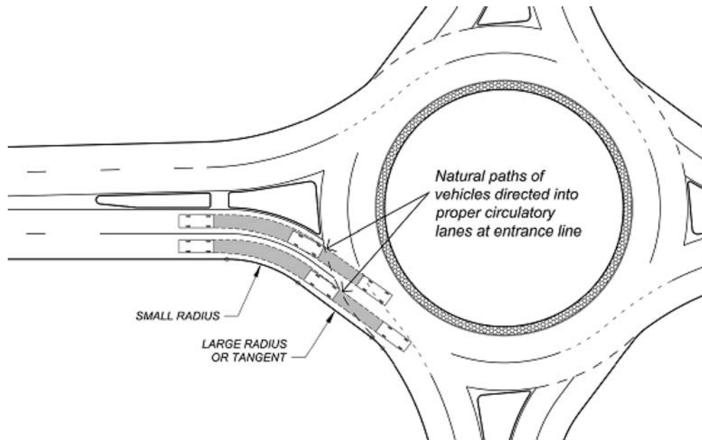
Figure 77. Design technique to minimize entry path overlap.
