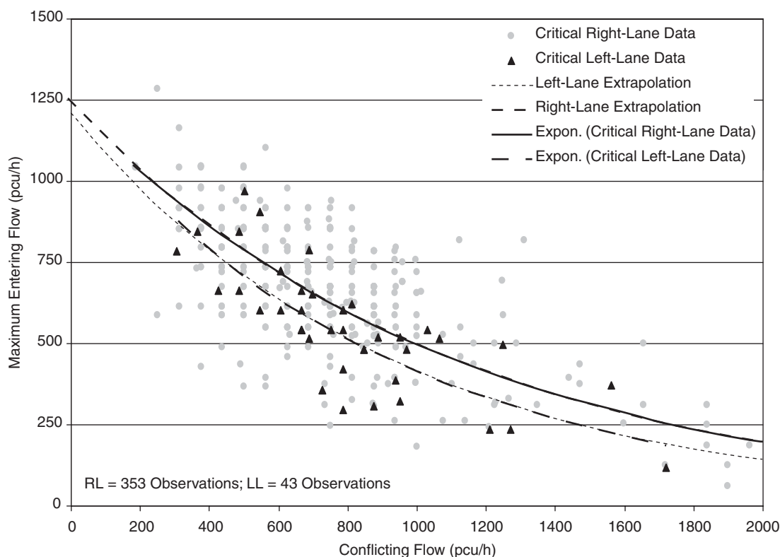
Figure 35. Critical right-lane and left-lane entry data.
