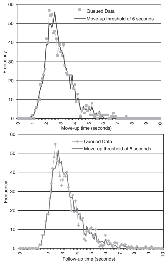
Figure 19. Move-up and follow-up time frequency (WA04-N).
