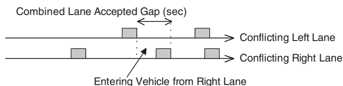
Figure 18. Concept of combined lane gaps.
