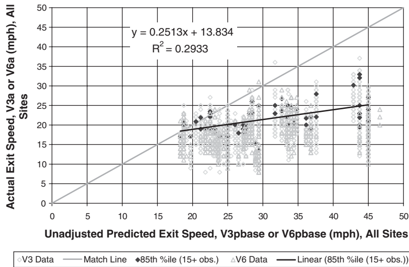
Figure 46. Actual vs. unadjusted predicted values for through-movement and left-turn-movement exit speeds, all sites.
