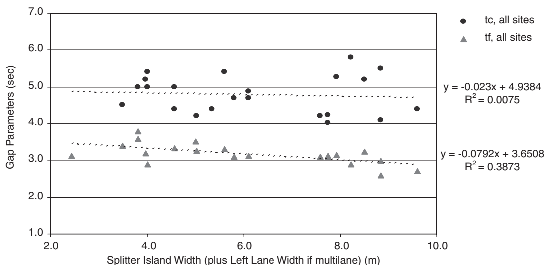
Figure 23. Critical headway and follow-up headway as a function of splitter island width (plus left-lane width if multilane).
