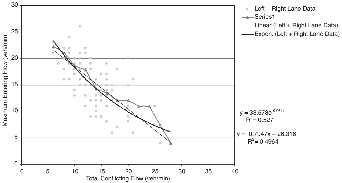
Figure 33. Regression and class means prediction for entry capacity.
