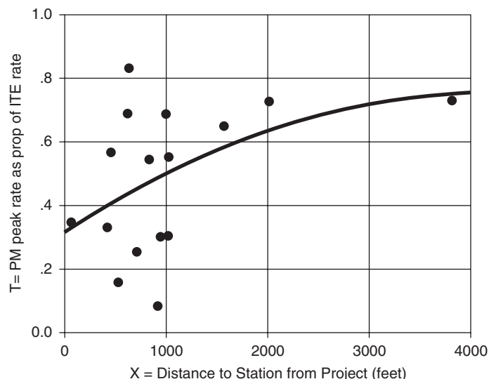
Figure 2.17. TOD-housing vehicle trip rate (as a proportion of ITE rate) by walking distance to station; quadratic curve; N = 17 .
