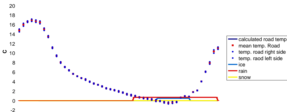
FIGURE 8 Road surface temperature, calculated and measured.
