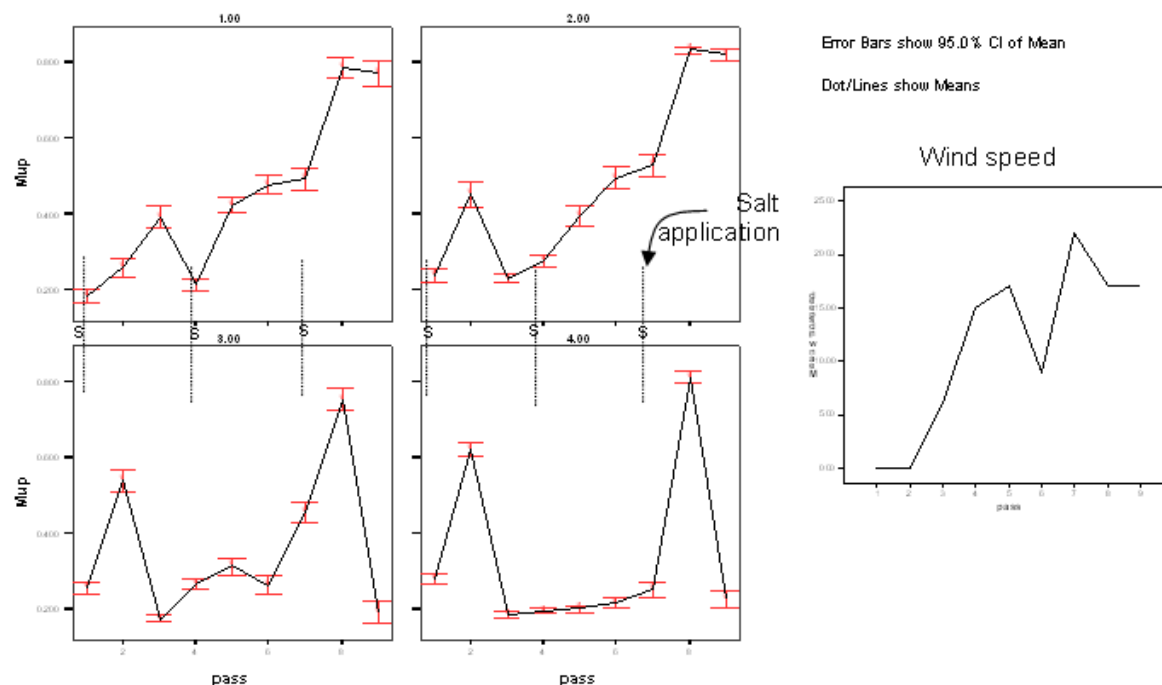
FIGURE 12 Mean friction, wind speed, and times of salt application for nine traverses in Zones 1, 2, 3, and 4, Field Area 3, January 9, 1999.
