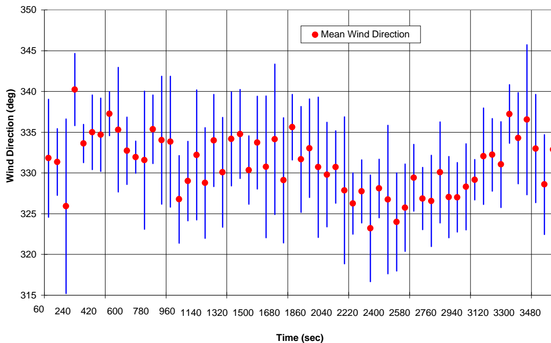
FIGURE 3 This graph shows wind direction at 10 m on December 15, 2005, at 1600 UTC. The red dots are 1-min averages of wind direction. The blue line at each observation time is the standard deviation from the average wind direction.
