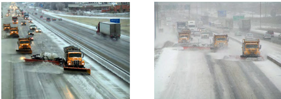
FIGURE 2 TowPlows in gangs.
