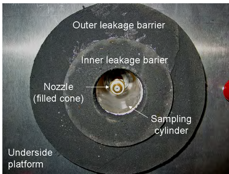
FIGURE 3 View of the underside of the sampling unit, showing the rubber beadings.
