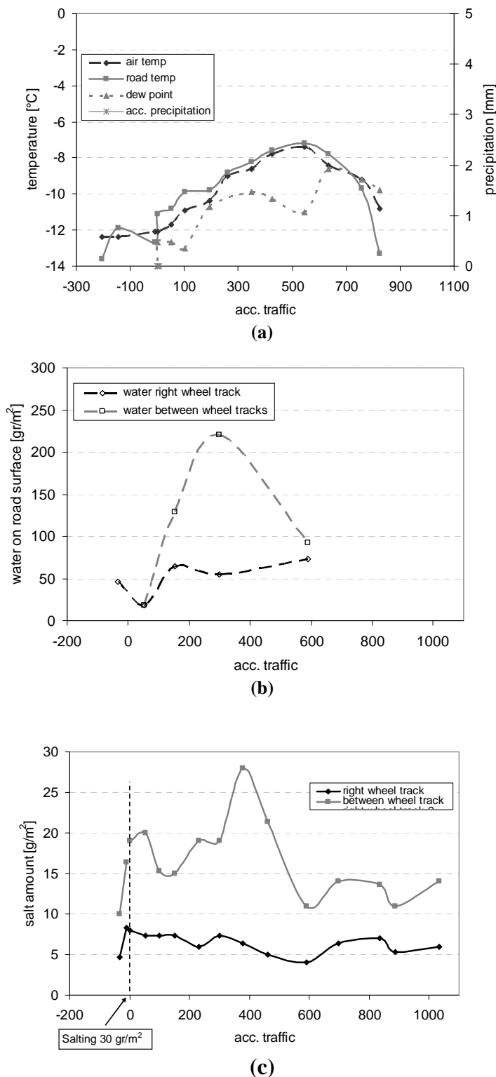
FIGURE 5 The data recorded in Case 1: (a) weather parameters, (b) amount of water on road surface, and (c) salt amount on road surface.
