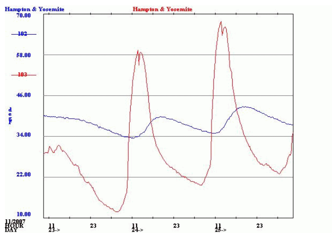
FIGURE 9 Pavement temperature graph.
