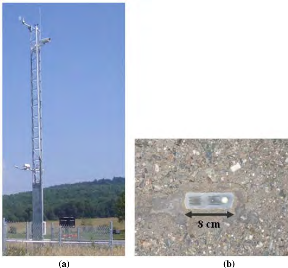
FIGURE 1 (a) Example of a traditional ESS set-up with a 10-m mast and (b) a close-up of an embedded road weather sensor in the pavement surface.
