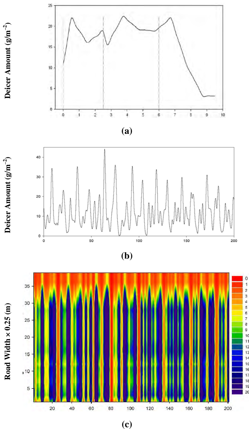
FIGURE 4 Example of transversal, longitudinal, and pavement amount of deicer: (a) example of transversal distribution of deicer (in \text{g/m}^2 ), (b) example of longitudinal distribution of deicer (in \text{g/m}^2 ) over a 200-m road section, and (c) brine mass title (in %) applied by a winter maintenance service over a 200-m road section [0% in red (no deicer), 20% in deep blue (close to a -23^\circ\text{C} freezing point)].
