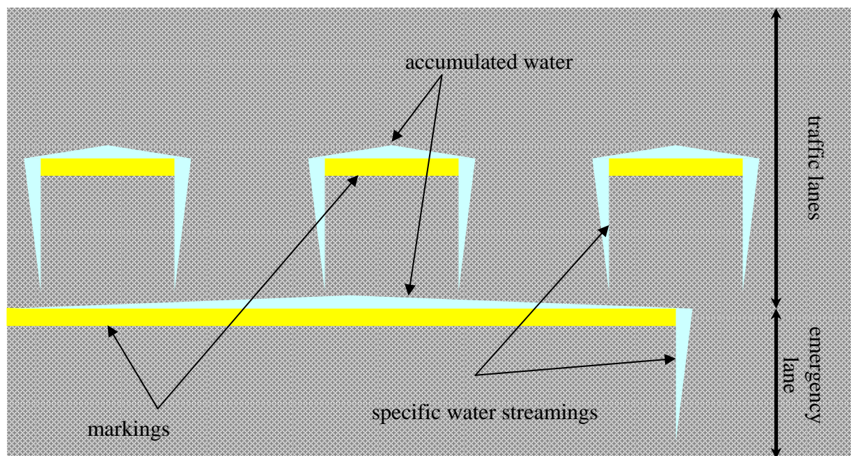
FIGURE 1 Pavement section with water accumulation anomalies due to markings (not at scale).
