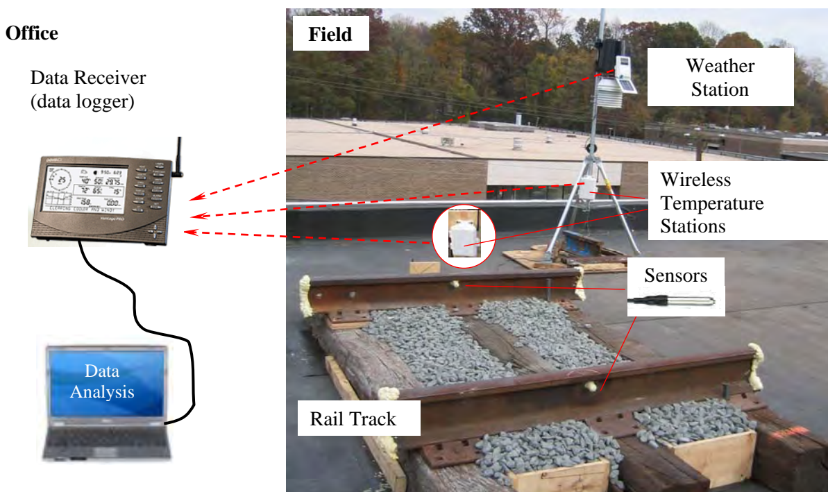
FIGURE 3 Rail-weather station.
