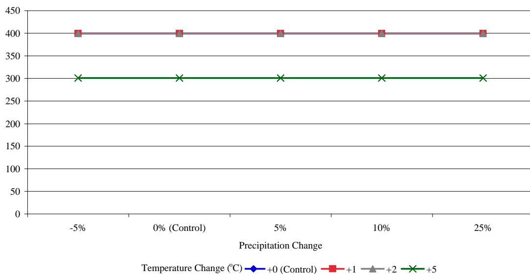
FIGURE 9 Ontario transverse cracking.
