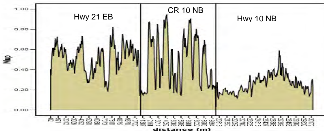
FIGURE 6 Friction trace for Field Area 2.
