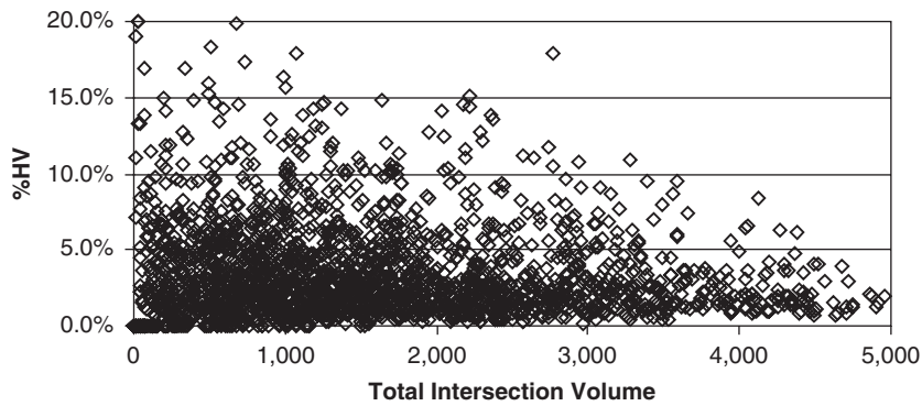
Figure 11. %HV as a function of total intersection volume.
