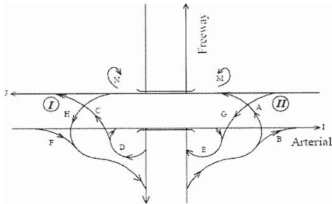
Figure B-6. Illustration of origin-destination demands through a PARCLO AB-2Q interchange.
