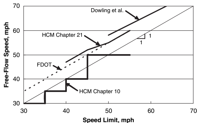
Figure 19. Comparison of guidance relating free-flow speed to speed limit.
