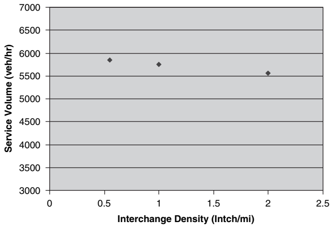
Figure 23. Service volume versus interchange density.
