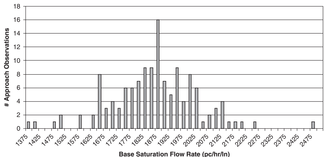
Figure 16. Frequency of the base saturation flow rate.
