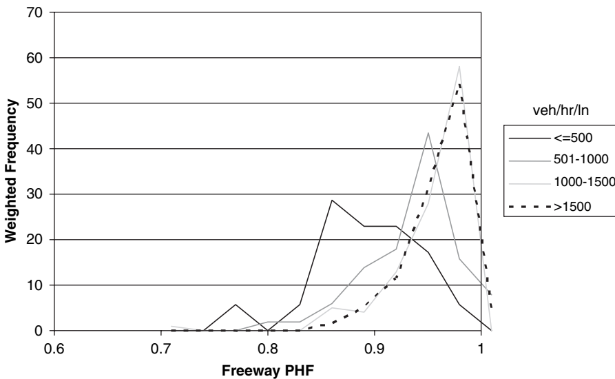
Figure 6. Weighted frequency of the freeway PHF for increasing volume bands.
