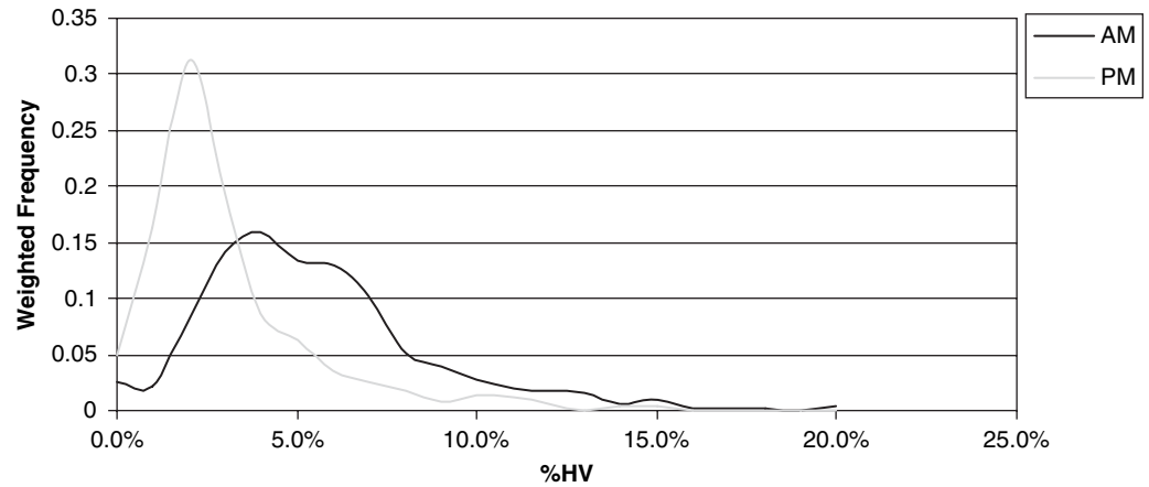
Figure 9. Weighted frequency of intersection %HV as a function of time period.
