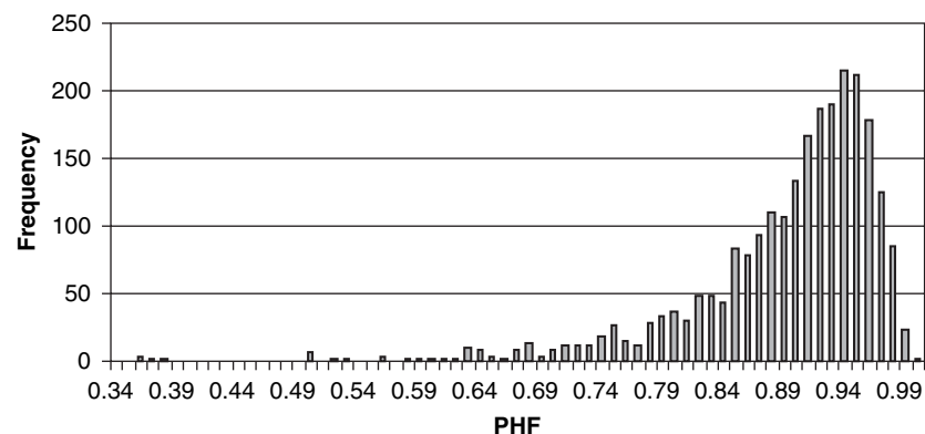
Figure 12. Frequency of intersection PHF.
