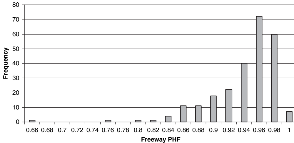
Figure 3. Frequency of freeway PHF.
