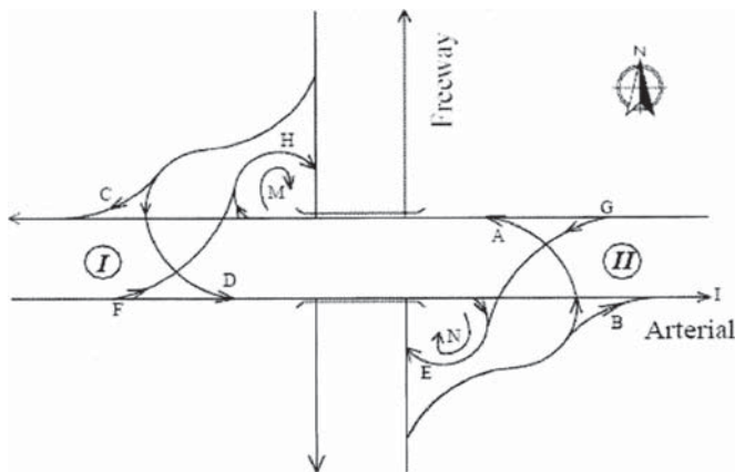
Figure B-2. Illustration of origin-destination demands through a PARCLO A-2Q.
