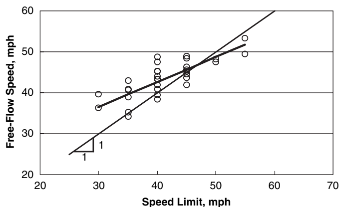
Figure 20. Relationship between speed limit and free-flow speed.
