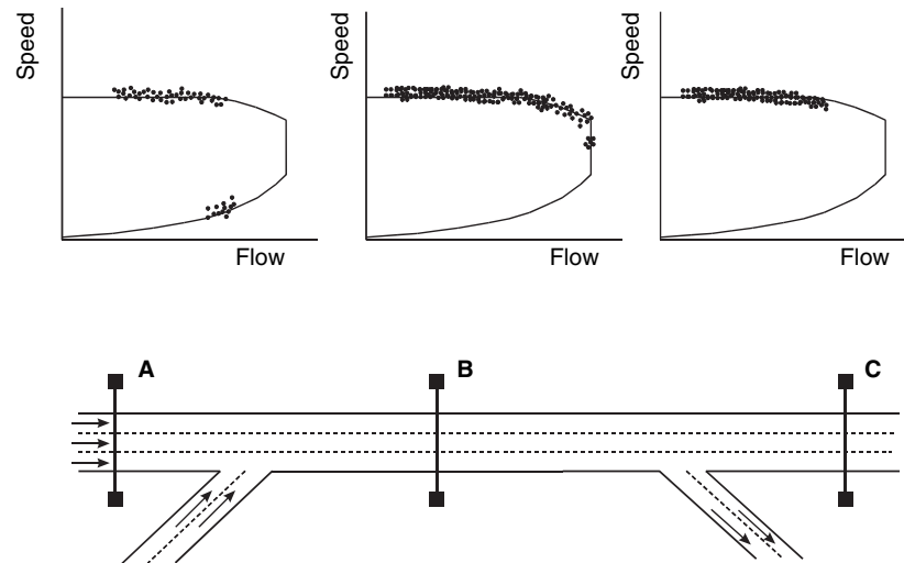
Figure 17. Measurement of capacity.
