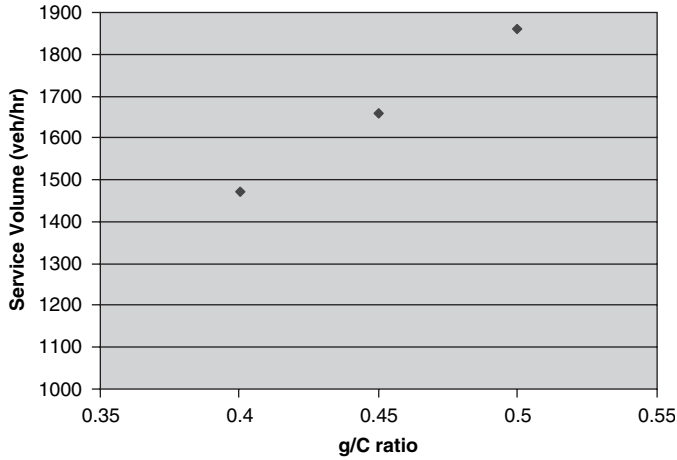
Figure 25. Service volume versus g/C ratio.
