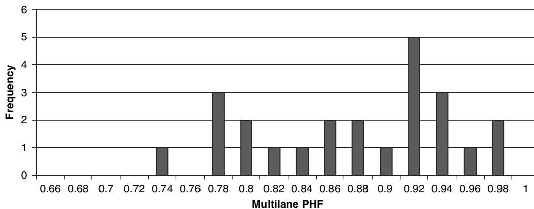
Figure 4. Frequency of multilane PHF.
