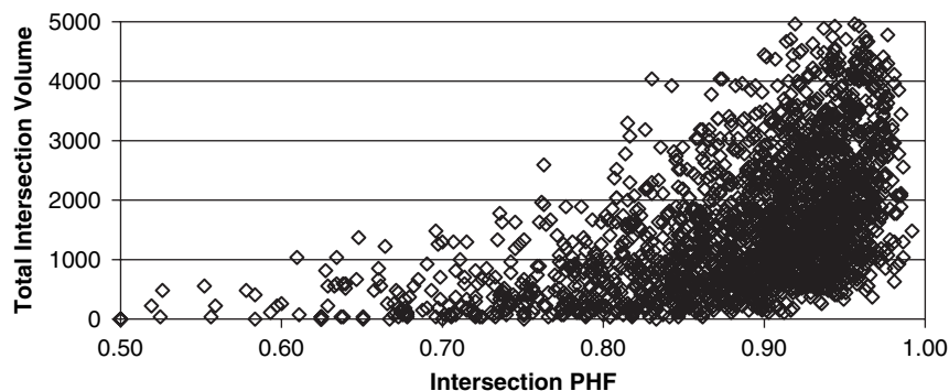
Figure 14. Intersection PHF as a function of total intersection volume.
