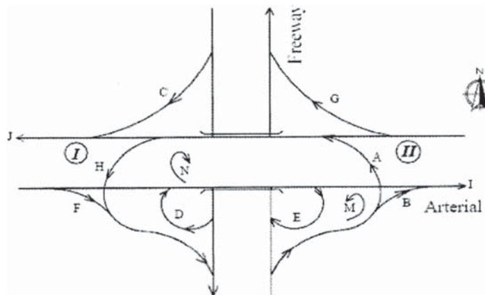
Figure B-4. Illustration of origin-destination demands through a PARCLO AB-4Q interchange.
