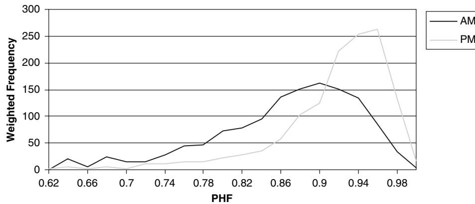
Figure 15. Intersection PHF as a function of time period.
