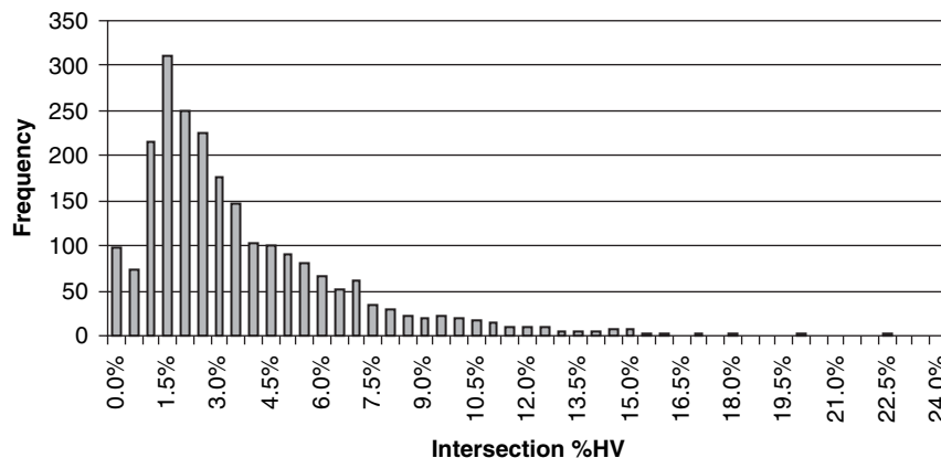
Figure 7. Frequency of intersection %HV.
