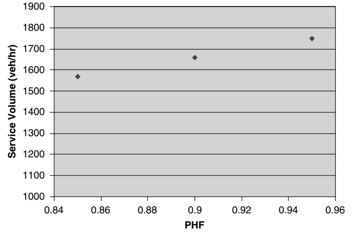
Figure 26. Service volume versus PHF.
