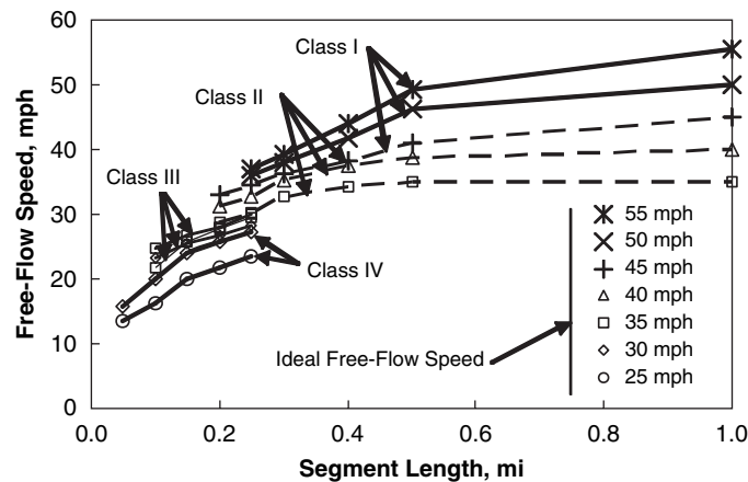
Figure 21. Influence of segment length on free-flow speed.
