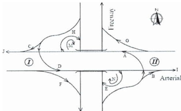
Figure B-5. Illustration of origin-destination demands through a PARCLO A-4Q interchange.
