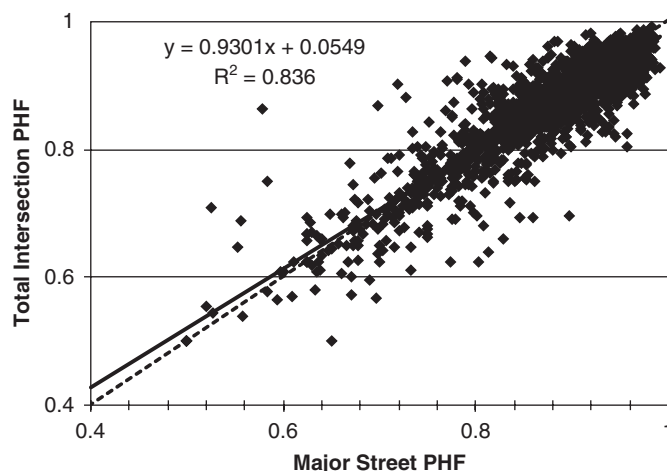
Figure 13. Intersection PHF as a function of major street PHF.
