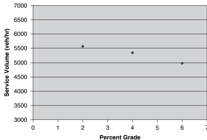
Figure 22. Service volume versus percent grade.
