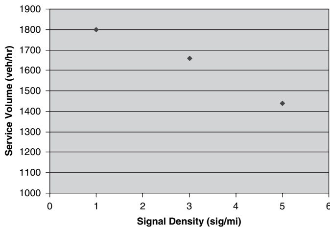
Figure 27. Service volume versus signal density.
