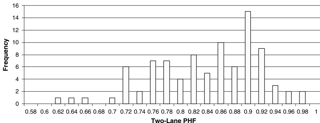
Figure 5. Frequency of two-lane PHF.
