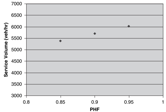
Figure 24. Service volume versus PHF.
