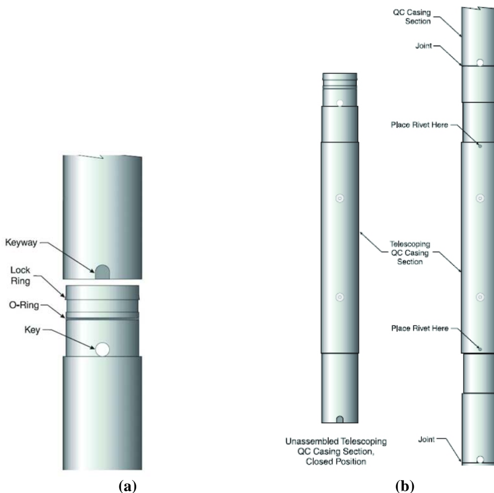
FIGURE 9 Inclinometer casing connections: (a) regular and (b) telescoping (Slope Indicator Company).
