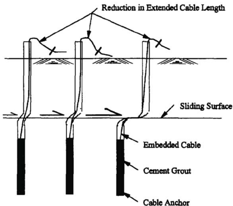
FIGURE 16 Extensometer cable installed in inclinometer casing to extend monitoring (Deschamps, 1998).
