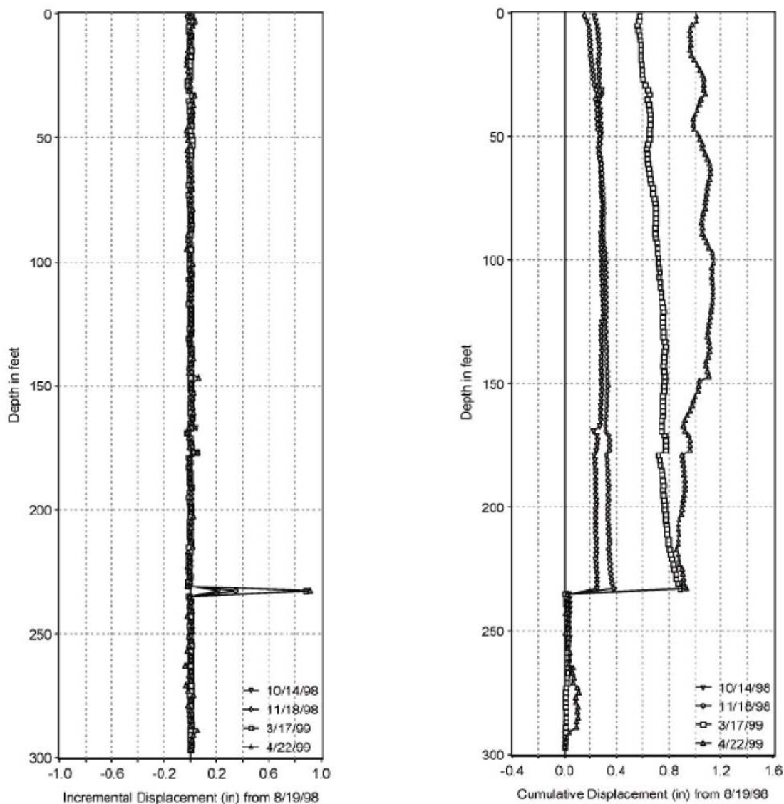
FIGURE 23 Comparison of data sets using incremental and cumulative displacement profiles (Slope Indicator Company, 2006a).
