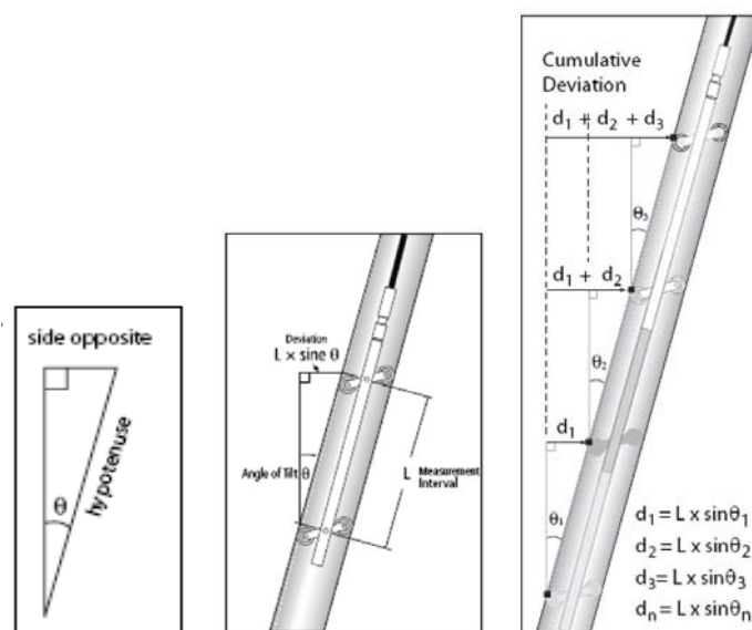
FIGURE 21 Measurement principles (Slope Indicator Company, 2006a).
