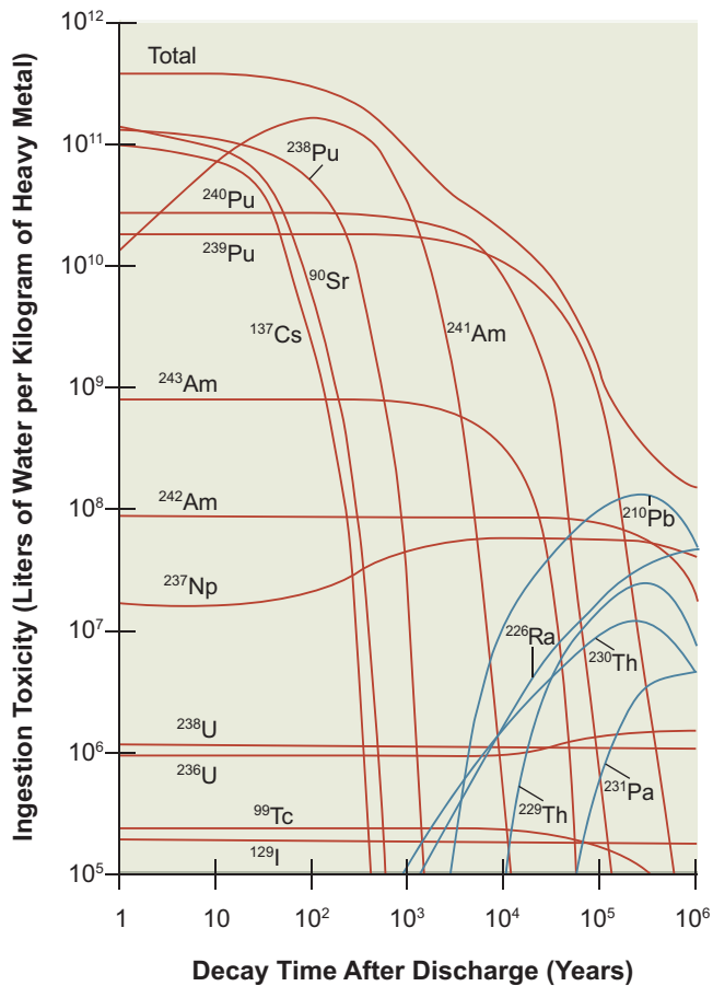
FIGURE 8.D.2 Toxicity of nuclides in used fuel from a light-water reactor. Toxicity is defined here as the volume of water required to dilute the radionuclide to its maximum permissible concentration per unit mass of the radionuclide. High index numbers denote more toxic radionuclides—that is, more water is required to dilute these radionuclides to “safe” levels. The toxicity levels shown in this figure are for direct human ingestion of used fuel and therefore would not necessarily apply for other exposure pathways. For example, radionuclide toxicities for exposures from groundwater would be dominated by isotopes that are soluble and not sorbed completely by the host rock. Source: Oak Ridge National Laboratory.
