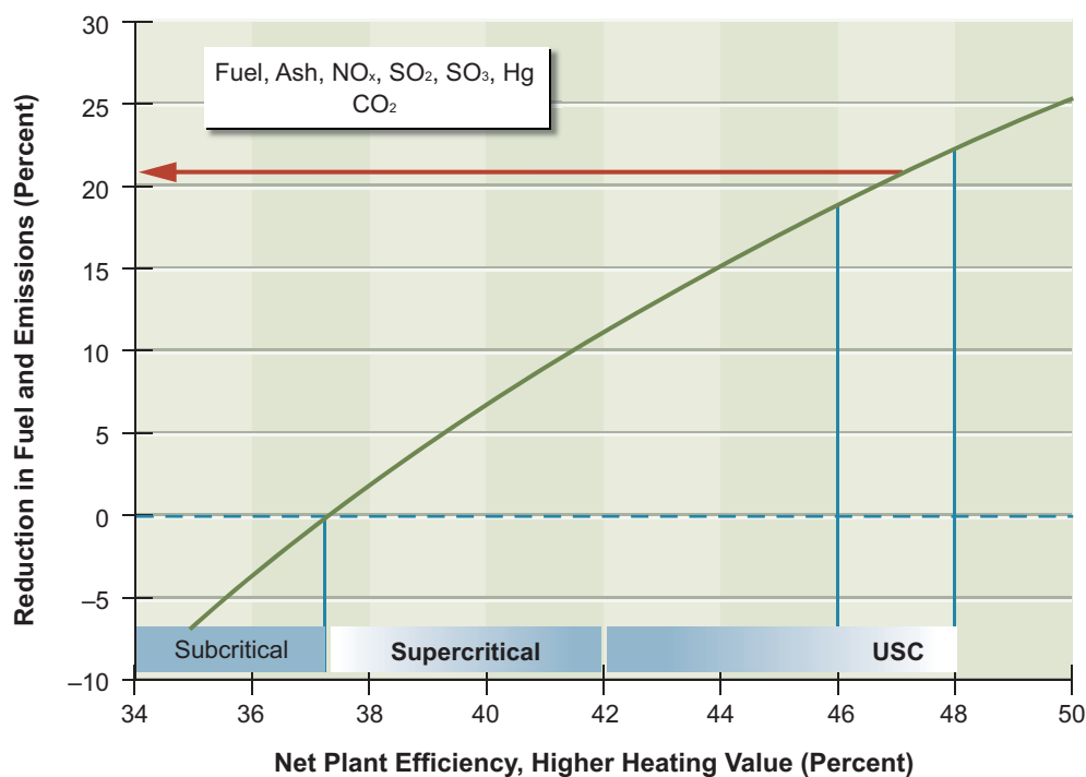
FIGURE 7.3 An ultrasupercritical (USC) boiler with an efficiency of 46–48 percent would reduce \text{CO}_2 emissions by 20 percent compared with a standard subcritical boiler.
