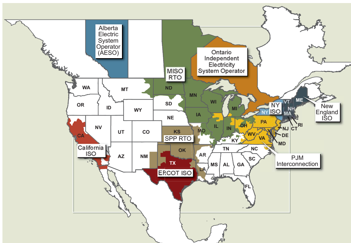
FIGURE 9.3 Independent System Operators (ISO) and Regional Transmission Organizations (RTO) in North America. Regions in which the power industry has been restructured, such as Texas, the Northeast, the Upper Midwest, and much of California, are colored. In these areas, ISO/RTOs are responsible for operating the transmission system. In the white regions, where the industry has not been restructured, vertically integrated power utilities continue to operate the transmission system. Source: North American Electric Reliability Corporation.
