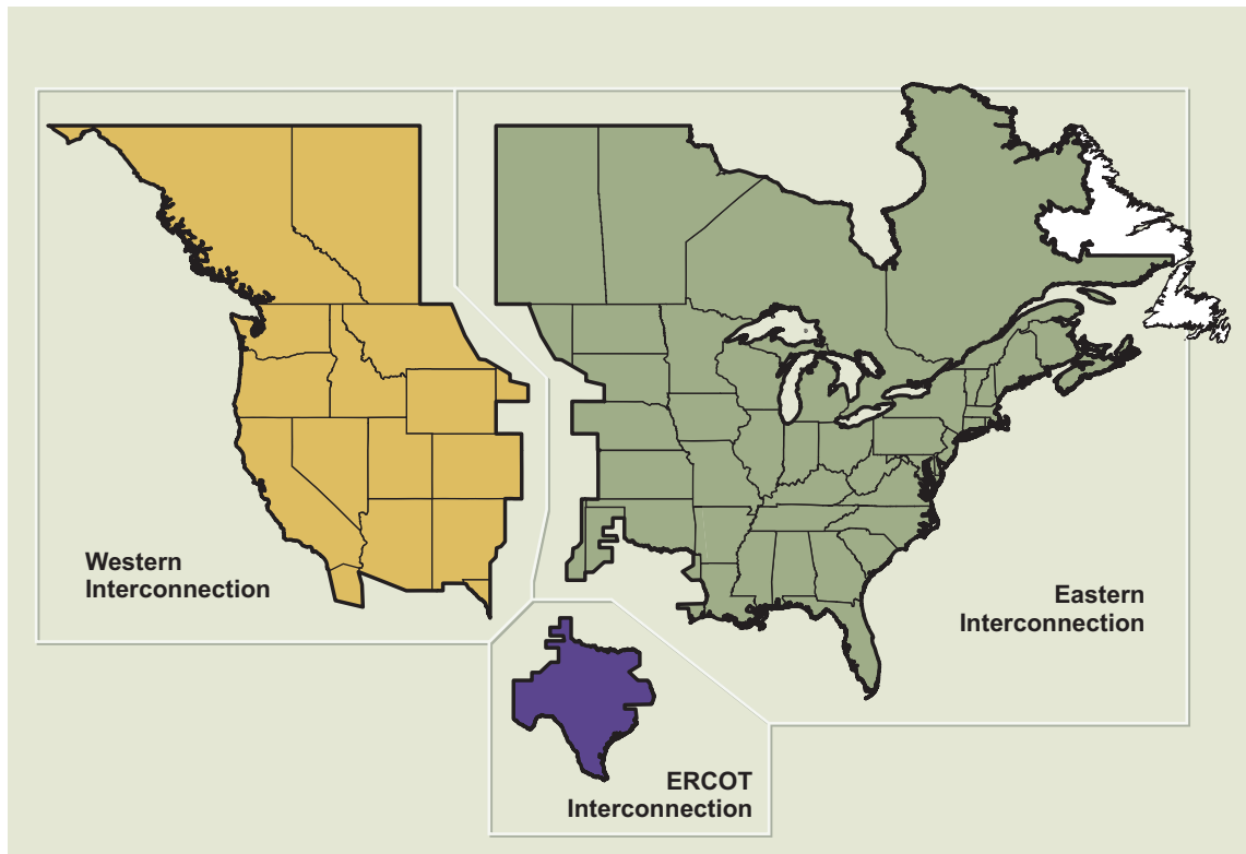
FIGURE 9.4 North American power interconnections. The Quebec Interconnection is shown as part of the Eastern Interconnection because operations are coordinated. Source: North American Electric Reliability Corporation.
