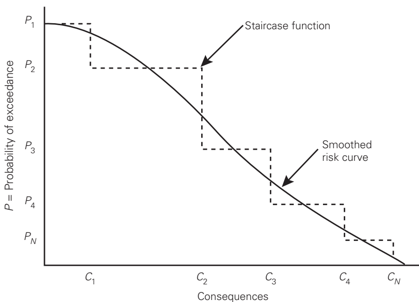
FIGURE 2-6 Risk curve.
