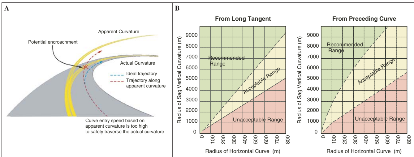
A. A vertical sag curve produces a visual image (shaded roadway) that a driver would perceive as having an apparent radius that is larger than the actual radius.
