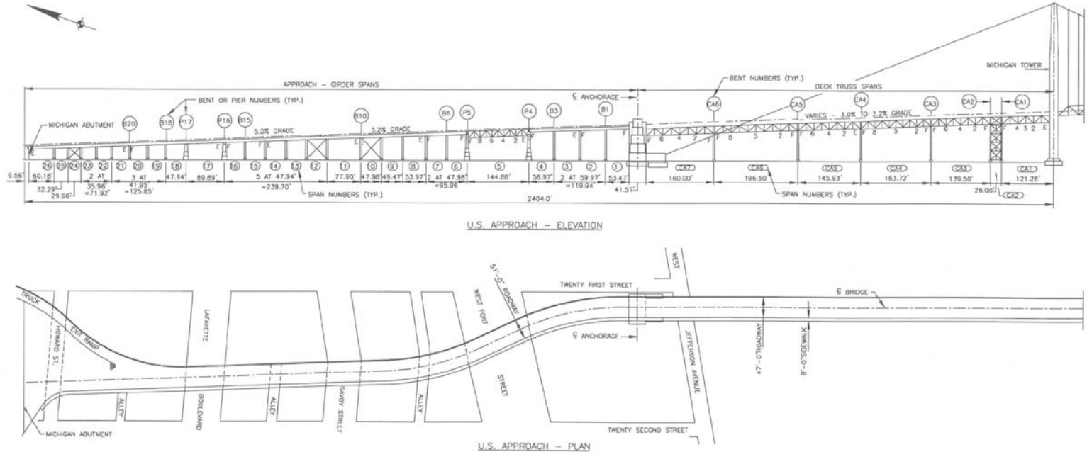
FIGURE 2 Plan and elevation of U.S. approach spans.
