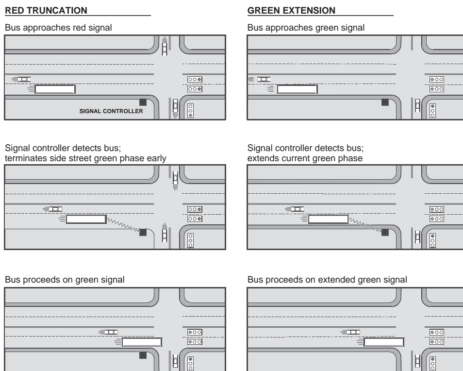
FIGURE 11 Red truncation/green extension TSP concept [Source: TCRP Report 118 (5)].
