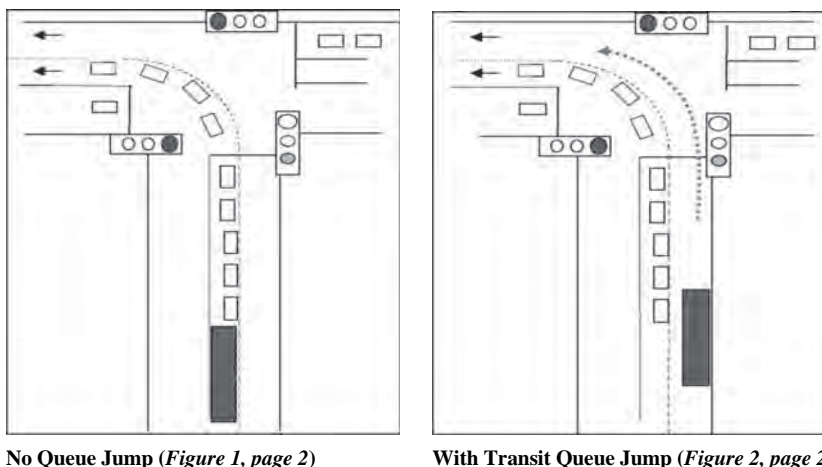
FIGURE 21 Queue jump at “T” intersection without special transit signal display (27).
