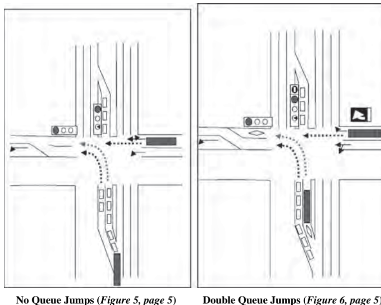
FIGURE 23 Multiple queue jumps at a four-legged intersection (27).
