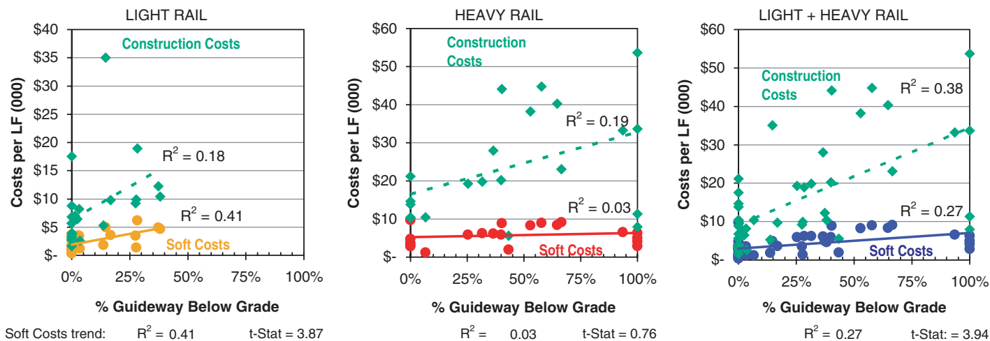
Figure 73. Soft costs and construction costs per linear foot with percent of guideway below grade.
