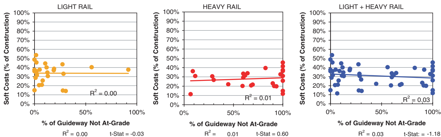
Figure 55. Soft costs as a percentage of construction versus percentage of guideway not at grade (retained cut and built-up fill designated as “at grade”).
