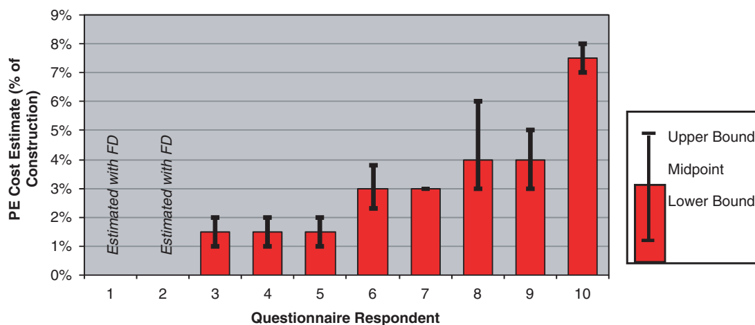
Figure 5. Preliminary engineering soft cost estimates.
