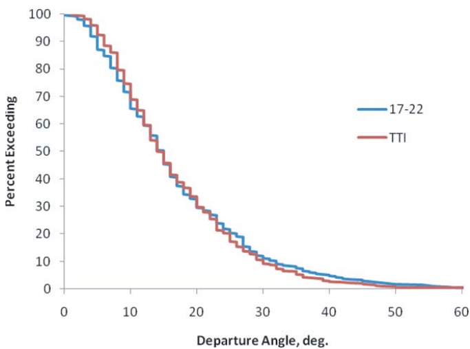
Figure 2. 17-22 and TTI departure angle distributions.
