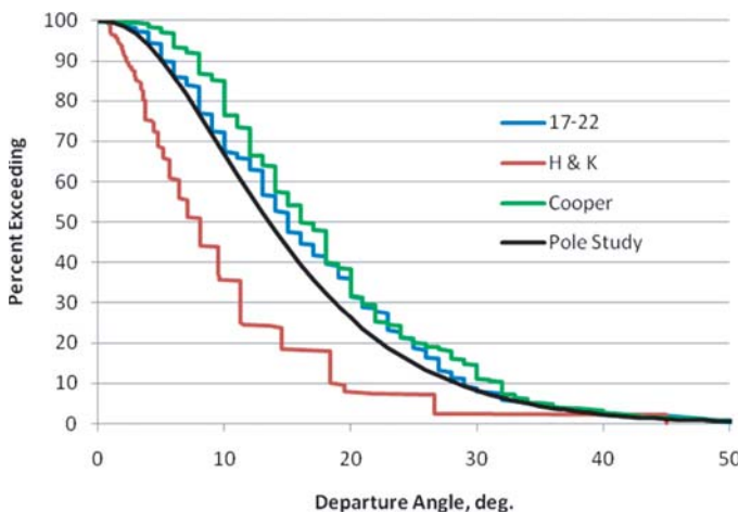
Figure 6. Comparison of freeway departure angle distributions.
