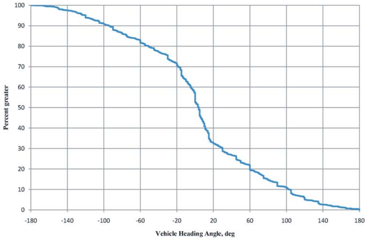
Figure 13. Vehicle orientation angle distribution.
