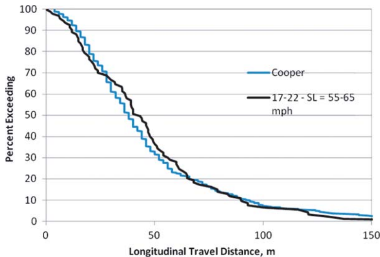
Figure 15. Cooper and 17-22 (55-65 mph) encroachment data comparison.
