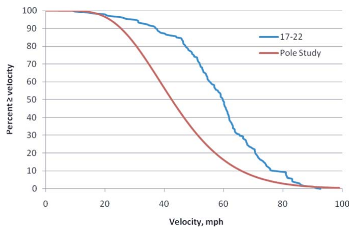
Figure 5. Freeway velocity distributions from Pole Study and 17-22.
