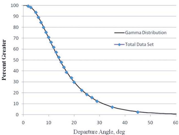
Figure 9. Square root of departure angle used to model departure angle (all data).
