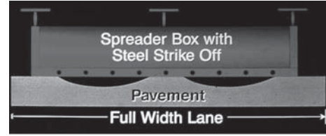
FIGURE 18 Scratch coat diagram (ISSA 2010a).
