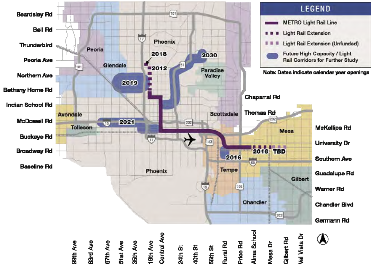
FIGURE 3 High-capacity–LRT system.
