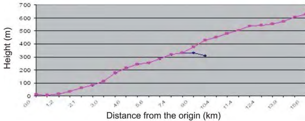
FIGURE 1 Longitudinal section, Tenerife light rail (II).
