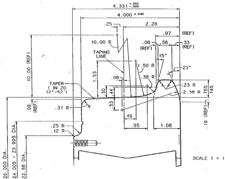
FIGURE 2 NLR wheel-rail interface: Penn machine drawing 9733.
