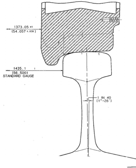
FIGURE 2 NLR wheel-rail interface: Penn machine drawing 9733.
