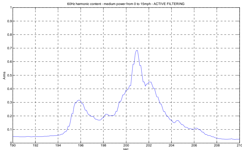
FIGURE 14 60-Hz emission level versus time for active filter propulsion system configuration.
