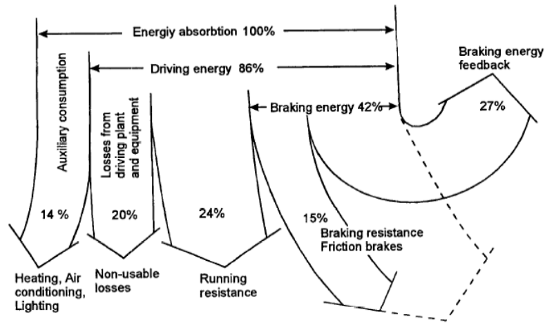
FIGURE 10 Division of rolling stock energy consumption (source: UITP).
