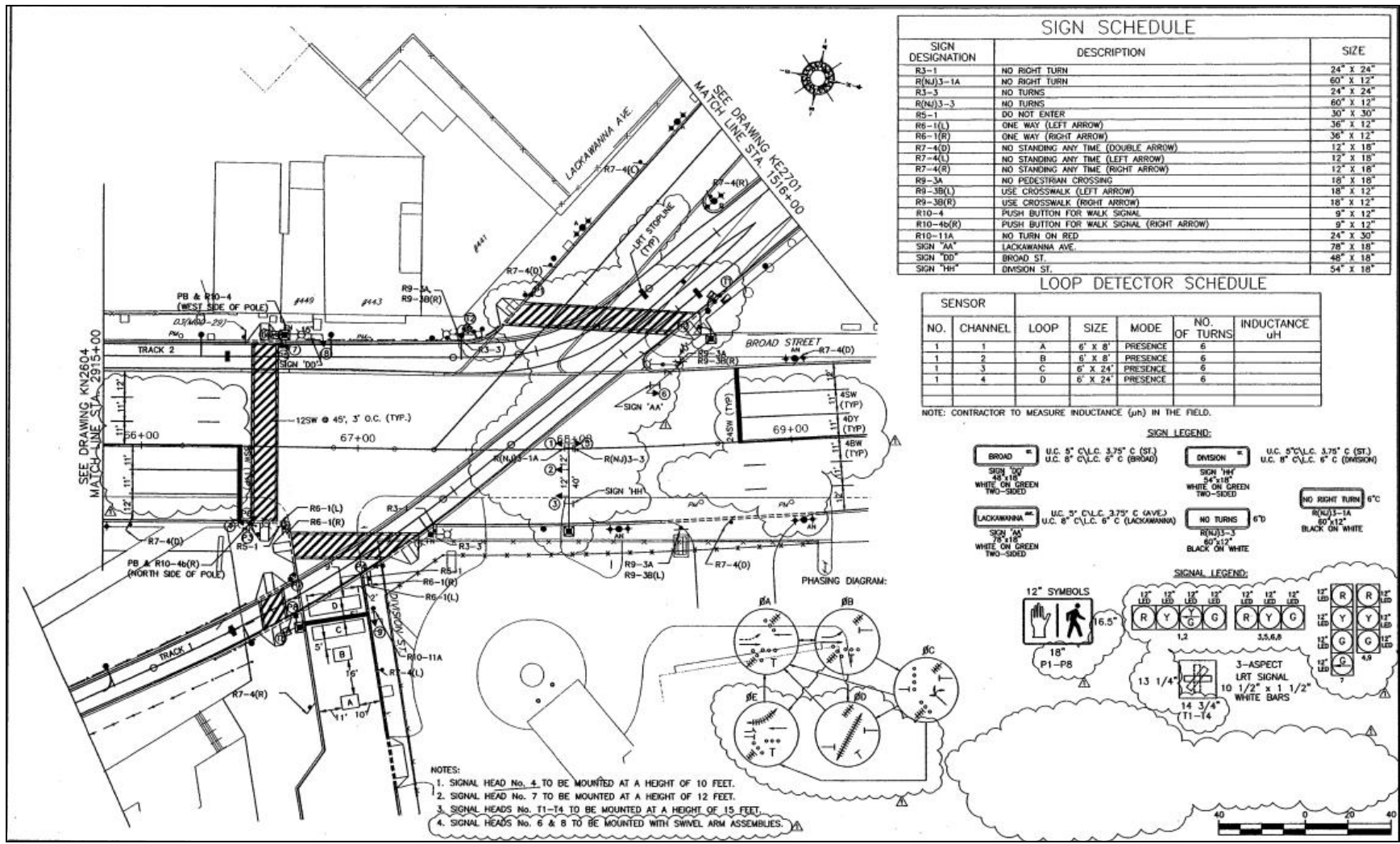
FIGURE 3 Traffic plan at intersection of Broad Street-Lackawanna Avenue-Division Street.
