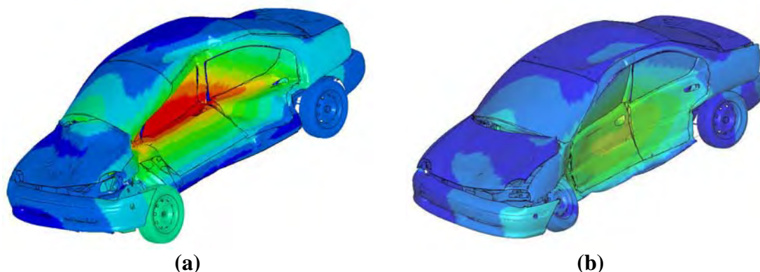
FIGURE 7 Calculated crush for HV 1 in the 90-degree, 20-mph collisions: (a) without bumper (maximum crush 67 cm) and (b) with bumper (maximum crush 43 cm).
