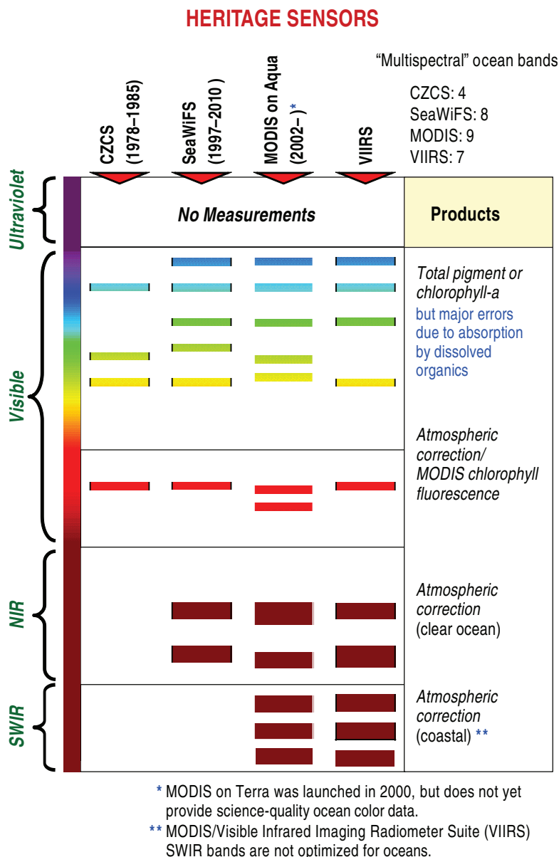
FIGURE 3.3 Comparison of spectral coverage of heritage sensors. SOURCE: Adapted with permission from Charles McClain, NASA/Goddard Space Flight Center.
