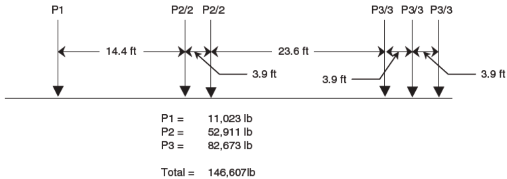
Figure 9 Mexican live load configuration.
