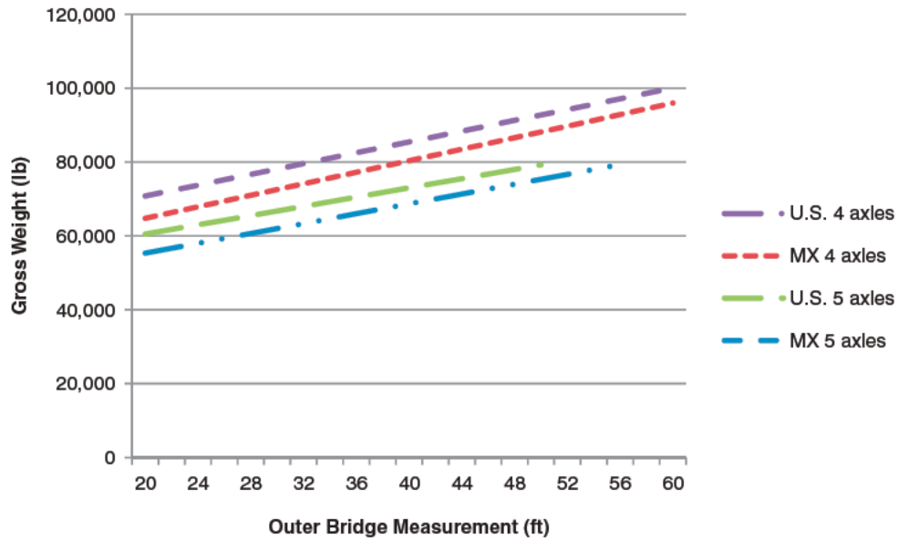
Figure 8 Comparison of U.S. Federal Bridge Formula B and the Mexico Bridge Formula.
