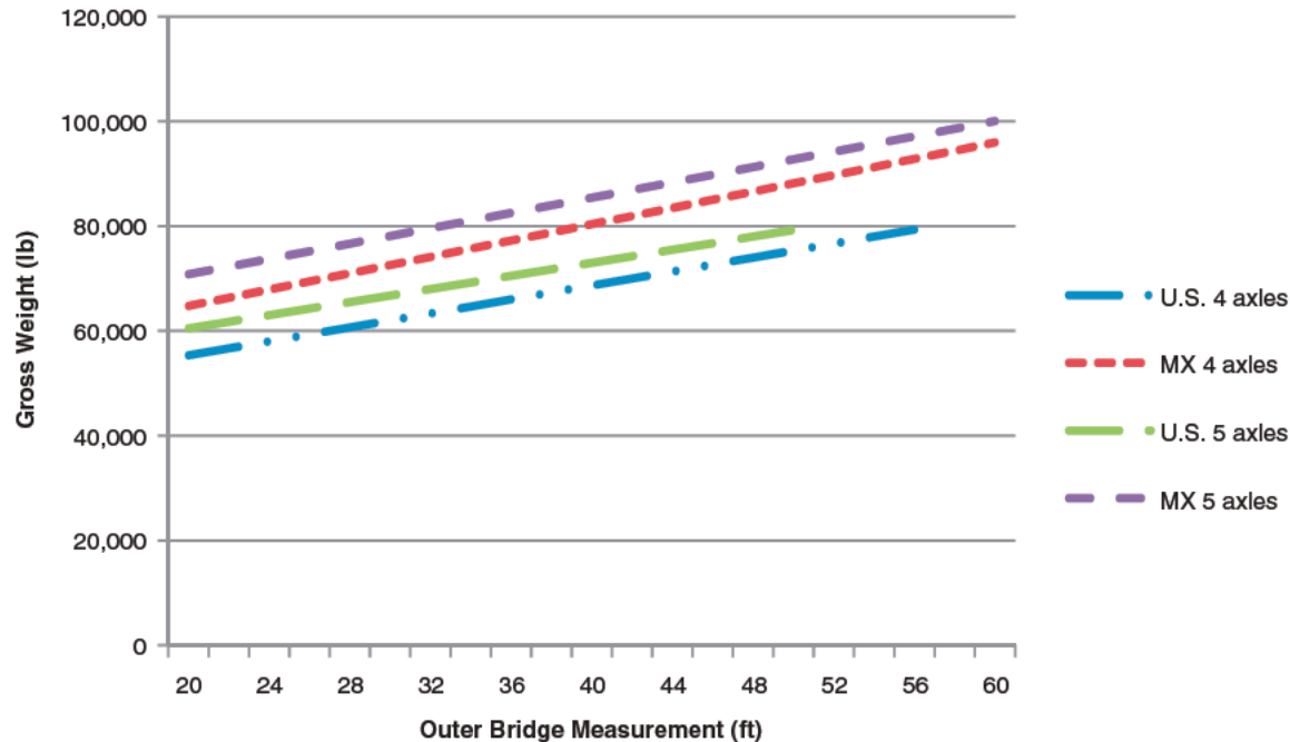
Figure 1 Comparison of U.S. Federal Bridge Formula B and the Mexico Bridge Formula.
