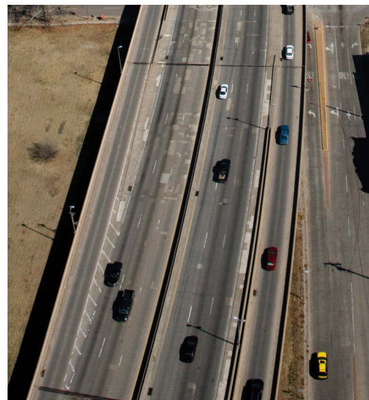
The I-40 Crosstown Expressway before the realignment project's start-up; the 50-year-old facility carries a daily traffic volume of more than 119,000 vehicles but was designed for 76,000. When the new facility opens in 2012, the old alignment will become a city street, providing the primary access into the downtown.
