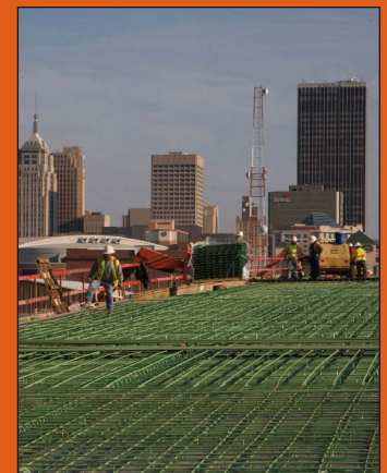
COVER: Workers tie reinforcing steel for the Shields Avenue bridge over the new I-40 alignment in Oklahoma City. (Photo courtesy of Oklahoma DOT)
