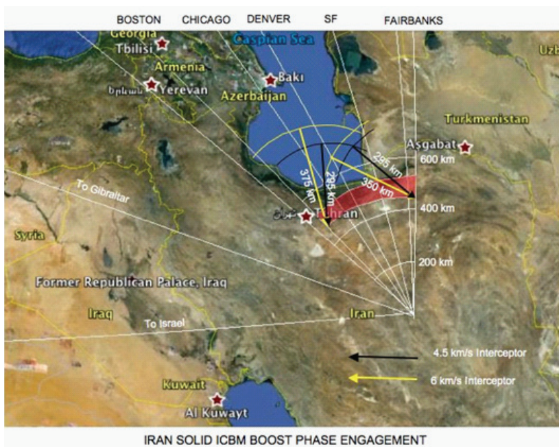
FIGURE 2-16 Notional boost-phase engagement of solid ICBMs launched from Iran.
