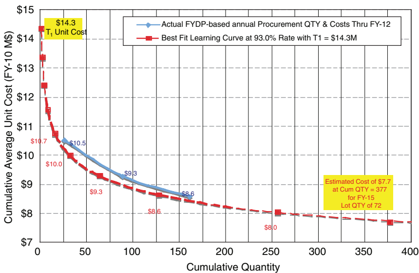
FIGURE E-9 THAAD missile. Cumulative average unit cost learning curve.
