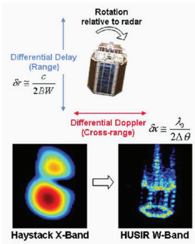
FIGURE 5-2 Example of ISAR satellite imaging from the Haystack radar complex.
