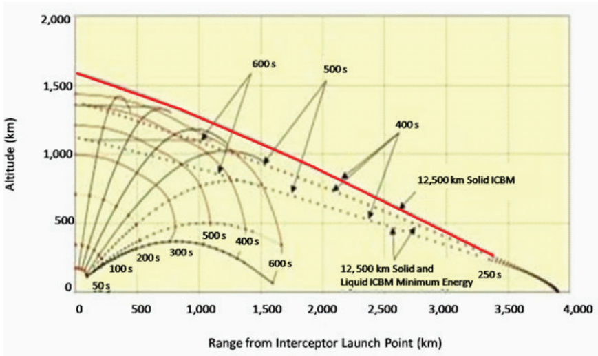
FIGURE 3-1 Notional ICBM trajectories from Iran to U.S. East Coast.
