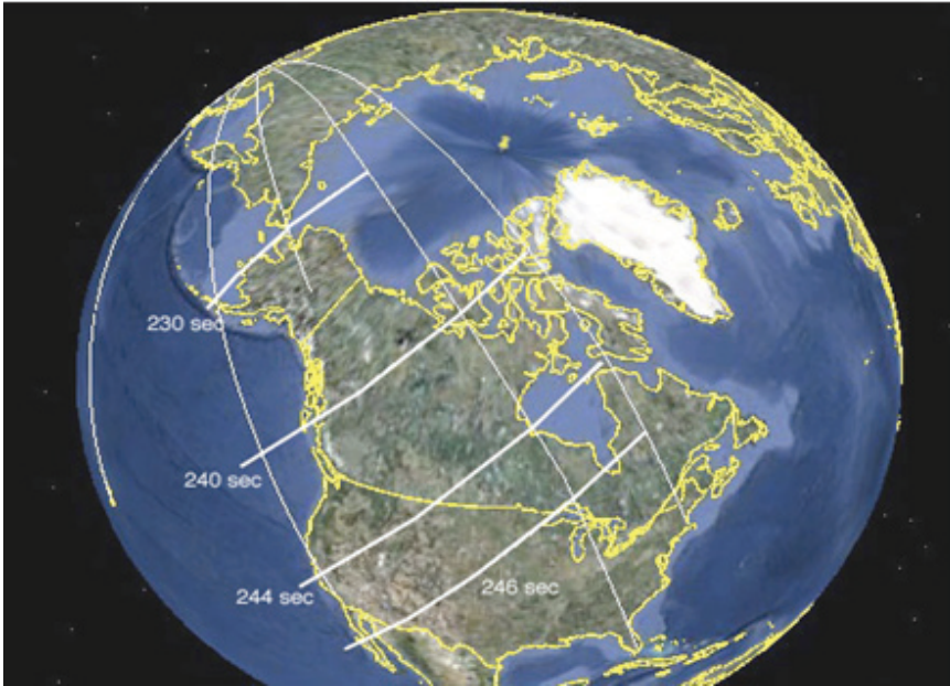
FIGURE 2-5 Thrust cutoff time contours for a notional two-stage liquid ICBM with an assumed total burn time of 250 sec and a maximum nonrotating Earth range of 12,000 km launched from North Korea.
