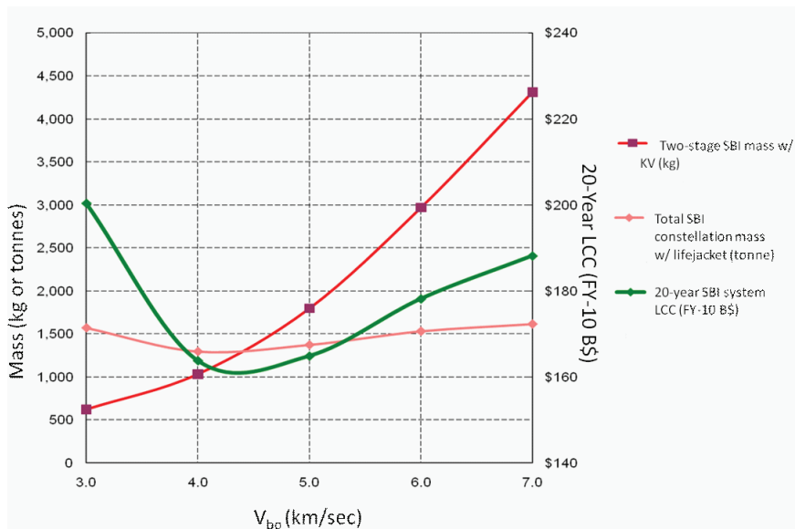
FIGURE E-4 Optimal booster burnout velocity at lowest LCC.
