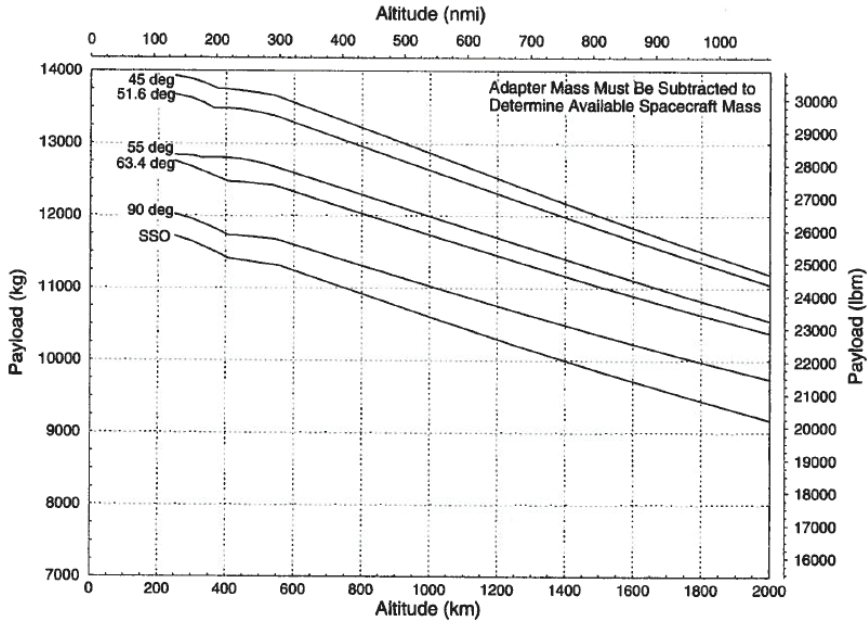
FIGURE E-5 Delta IV medium + (5.4) LEO launch lift capability. SOURCE: S.J. Isakowitz, J.B. Hopkins, and J.P. Hopkins, Jr. 2004. International Reference Guide to Space Launch Systems , 4th edition, American Institute of Aeronautics and Astronautics.
