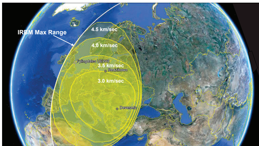
FIGURE 3-6 Notional single-shot coverage for interceptors with fly-out velocity varied parametrically between 3.0 and 4.5 km/sec against depressed trajectories from central Iran. EOR is assumed.
