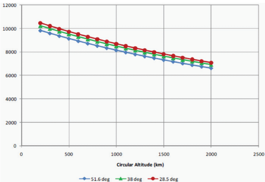
FIGURE E-7 Falcon 9 Block II LEO launch lift capability. SOURCE: Space X Falcon 9 User's Guide, SCM 2009-010 Revision 1, Figure 4.1, "Falcon 9 Block 2 Performance to Low Earth Orbit (Cape Canaveral)."
