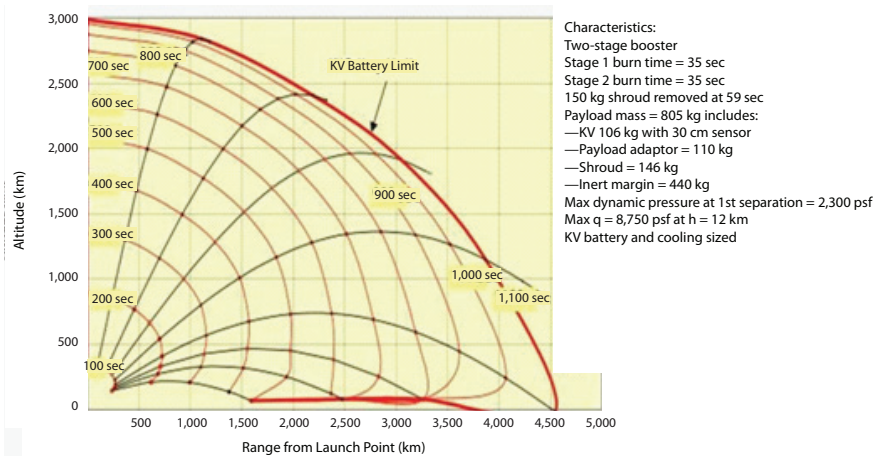
FIGURE 5-4 Recommended notional GMD-E interceptor fly-out contours with 6 km/sec interceptor fly-out contours and two-stage 70-sec total burn.
