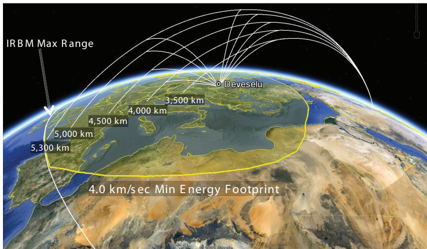
FIGURE 3-2 Notional engagement opportunities of a 4-km/sec fly-out velocity interceptor against minimum energy threats from central Iran flying directly over the planned Deveselu site.
