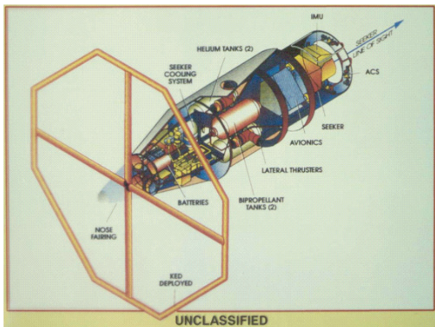
FIGURE 5-7 Exoatmospheric Re-entry Interceptor Subsystem (ERIS) KKV configuration showing enhancement device concept in the deployed position. SOURCE: David K. Barton, Roger Falcone, Daniel Kleppner, Frederick K. Lamb, Ming K. Lau, Harvey L. Lynch, David Moncton, et al. 2004. Report of the American Physical Society Study Group on Boost-Phase Intercept Systems for National Missile Defense: Scientific and Technical Issues , American Physical Society, College Park, Md., October 5, p. S207.
