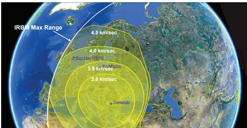
FIGURE 3-4 Notional single-shot coverage for interceptors with fly-out velocity varied parametrically between 3.0 and 4.5 km/sec against minimum energy notional 5,600-km solid IRBM trajectories from central Iran. EOR is assumed.
