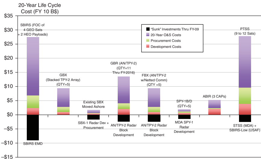
FIGURE 4-2 Twenty-year LCCs for sensors for U.S. boost-phase and non-boost phase alternatives. Note that (1) the 20-yr LCC estimate for SBIRS includes O&S costs of the replenishment GEO satellites and host satellites with HEO payloads and associated launches needed to sustain the 4 + 2 constellation with an average expected on-orbit life of 10 years per satellite; (2) the 20-yr LCC estimate for Precision Tracking and Surveillance System (PTSS) includes the O&S cost of the replenishment satellites and launches needed to sustain the constellation based on an average expected on-orbit life of 7 years per satellite. HEO, high Earth orbit; GEO, geostationary Earth orbit; GBX, ground-based X-band radar; STSS, space tracking and surveillance system; FOC, full operational capability.
