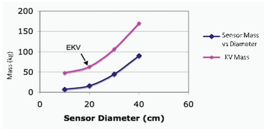
FIGURE 5-6 GMD-E midcourse KV and sensor mass as a function of aperture diameter.
