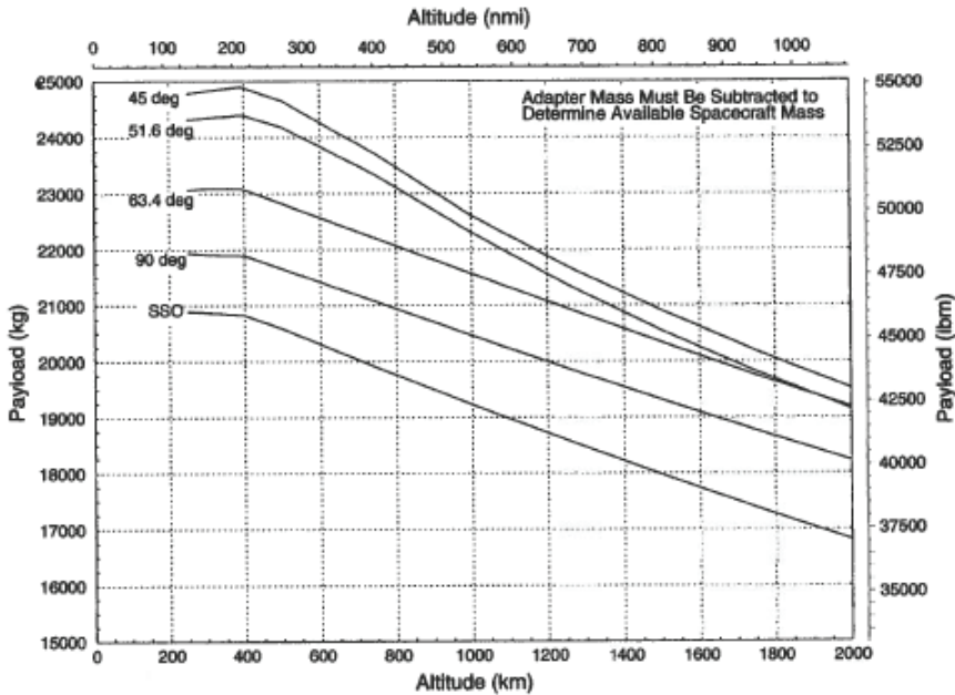
FIGURE E-6 Delta IV heavy LEO launch lift capability. SOURCE: S.J. Isakowitz, J.B. Hopkins, and J.P. Hopkins, Jr. 2004. International Reference Guide to Space Launch Systems , 4th edition, American Institute of Aeronautics and Astronautics.
