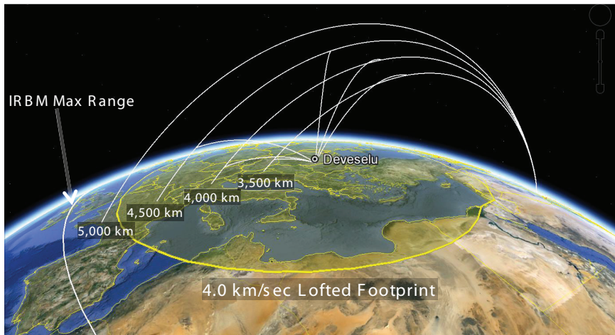
FIGURE 3-3 Notional engagement opportunities of a 4-km/sec fly-out velocity interceptor against moderately lofted threats from central Iran flying directly over the planned Deveselu site.
