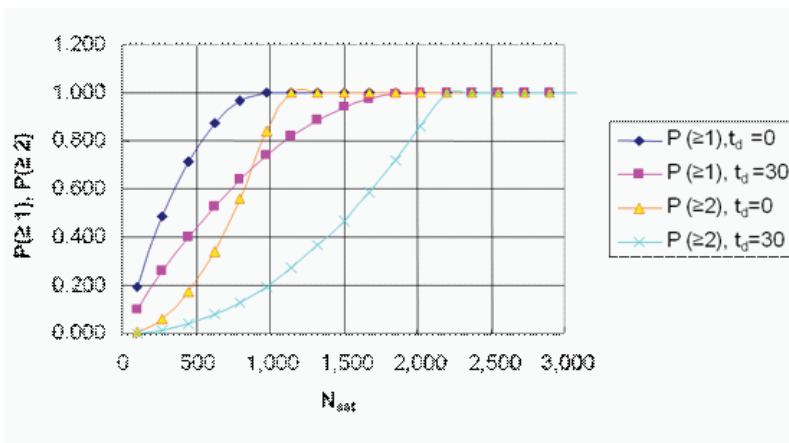
FIGURE 2-18 Probability as a function of the number of satellites in the constellation for a solid-propellant ICBM launched from Iran and notional 5.0 km/sec interceptors.
