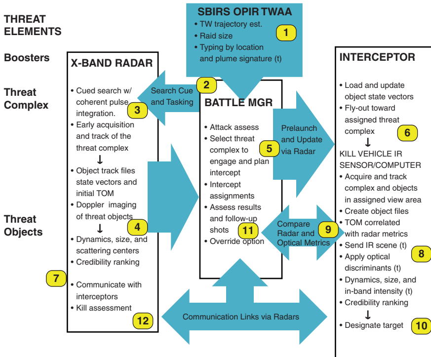
FIGURE 5-1 Synergy of concurrent radar and KV optical observations. OPIR, other program infrared; TWAA, tactical warning and attack assessment; IR, infrared.
