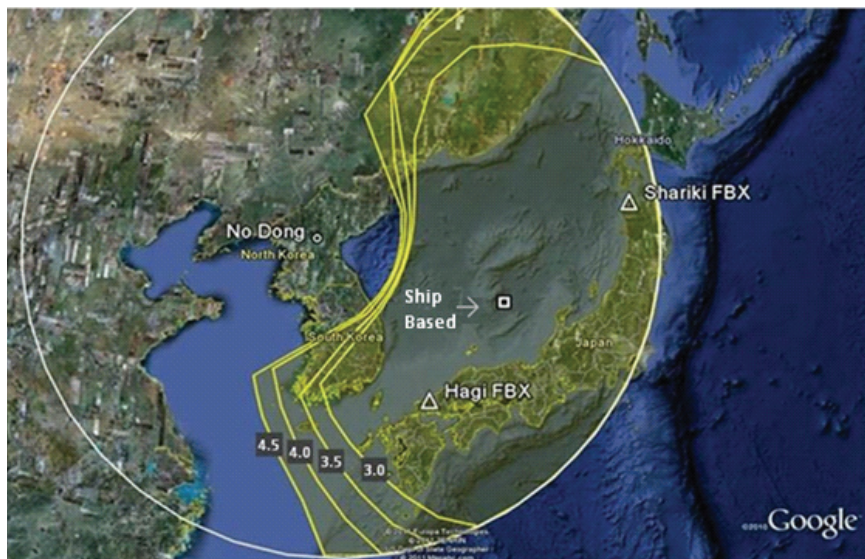
FIGURE 3-13 Notional ship-based single-shot EOR coverage of Japan: depressed MRBM trajectories. Note Hagi FBX location is notional.
