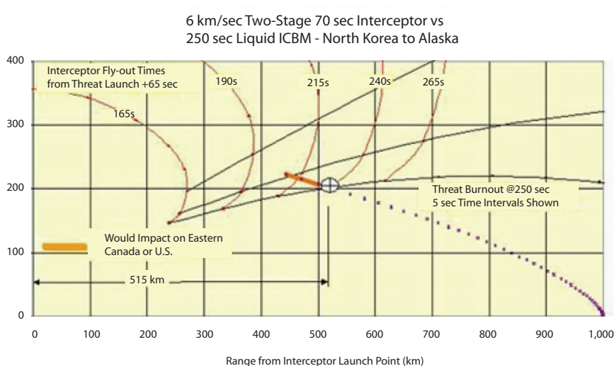
FIGURE 2-10 Fly-out fan for a notional 6 km/sec interceptor engaging a liquid-propellant ICBM head-on to determine R_i .
