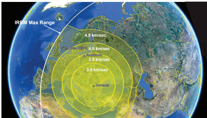
FIGURE 3-5 Notional single-shot coverage for interceptors with fly-out velocity varied parametrically between 3.0 and 4.5 km/sec against lofted trajectories from central Iran. EOR is assumed.
