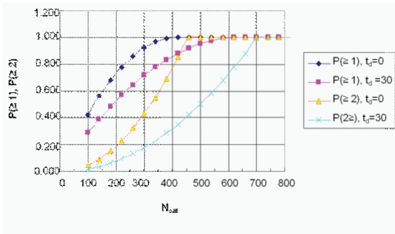
FIGURE 2-19 Probability as a function of the number of satellites in the constellation for a liquid-propellant ICBM launched from Iran and notional 5.0 km/sec interceptors.
