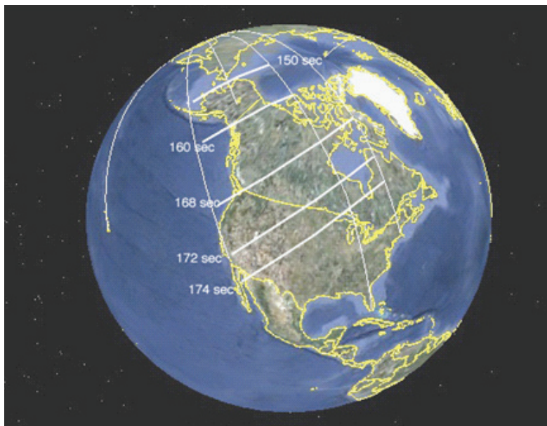
FIGURE 2-6 Thrust cutoff time contours for a notional three-stage solid ICBM with an assumed burn time of 180 sec and a maximum nonrotating Earth range of 12,000 km launched from North Korea.
